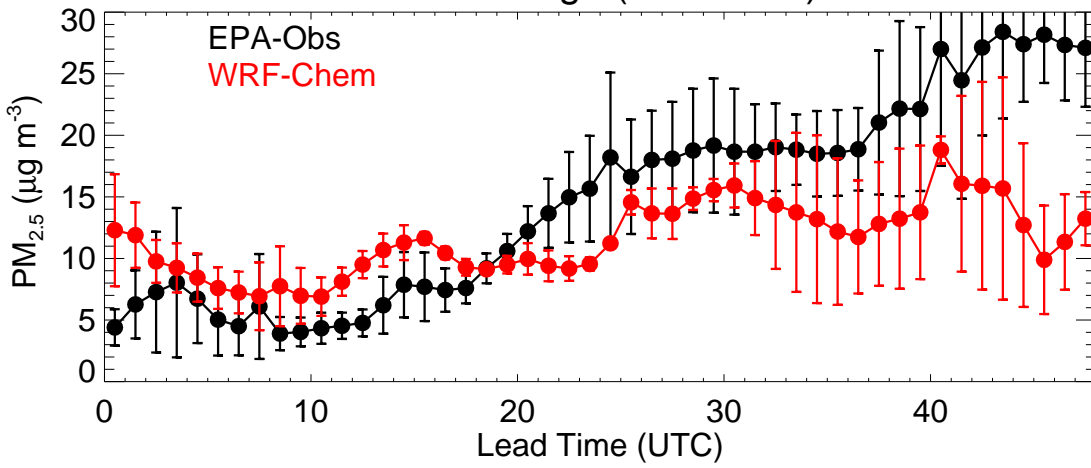
Front Range (20211108)
