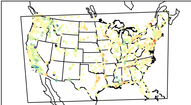
Mean Bias (20211108)
