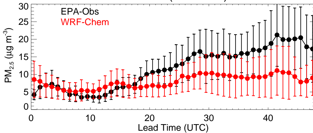
Colorado (20211108)
