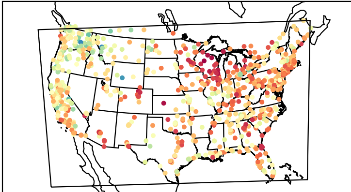
Correlation Coefficient (20211108)
