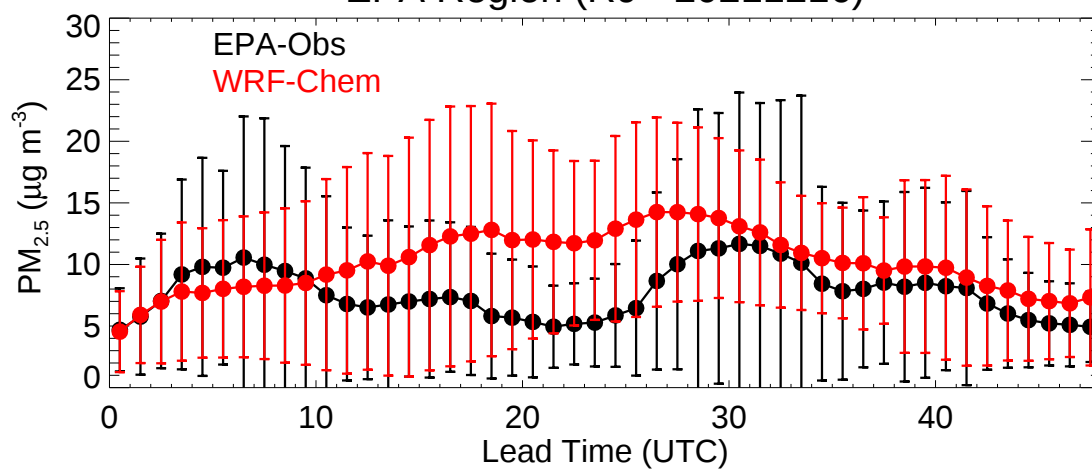
EPA Region (R10 - 20211216)
