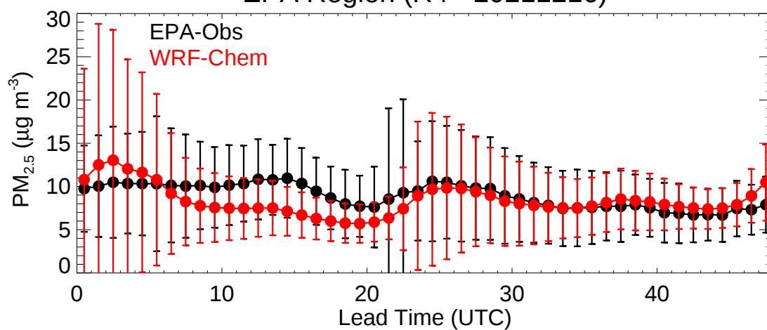
EPA Region (R5 - 20211216)
