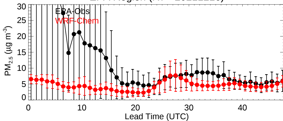
EPA Region (R8 - 20211216)
