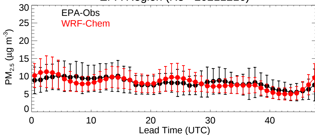
EPA Region (R4 - 20211216)
