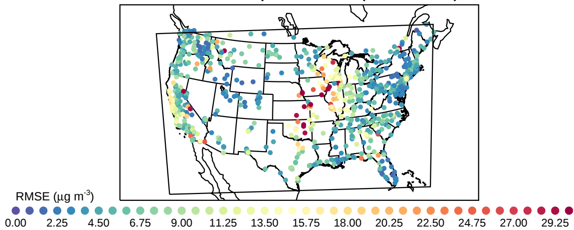
Root Mean Square Error (20211216)
