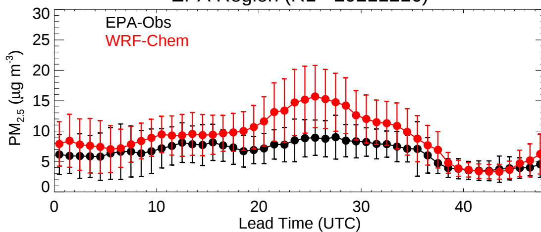
EPA Region (R2 - 20211216)
