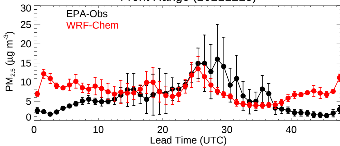
Front Range (20211218)
