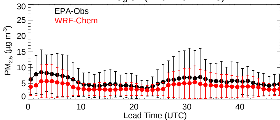
Colorado (20211218)
