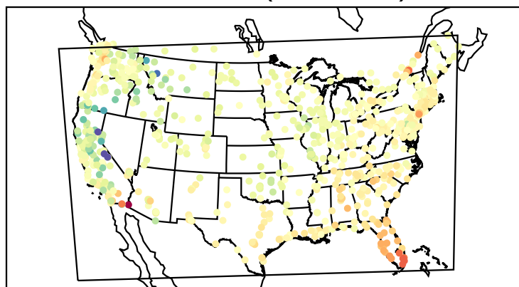
Mean Bias (20211218)
