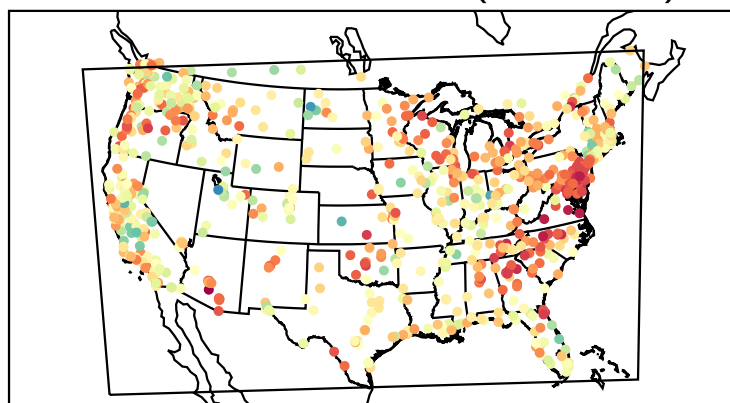
Correlation Coefficient (20211218)
