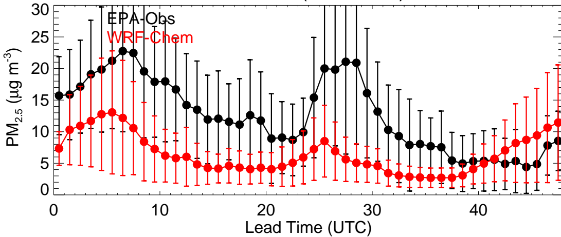
Colorado (20220226)
