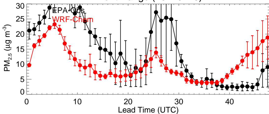
Front Range (20220226)
