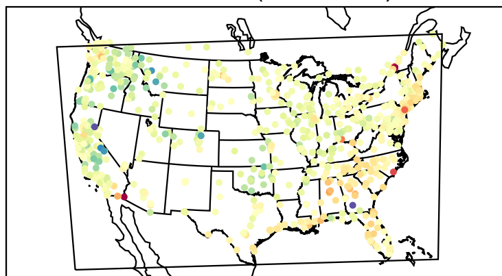
Mean Bias (20220226)
