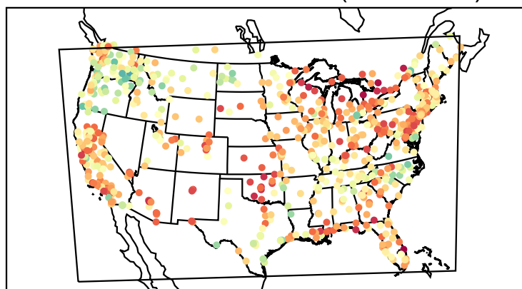
Correlation Coefficient (20220226)
