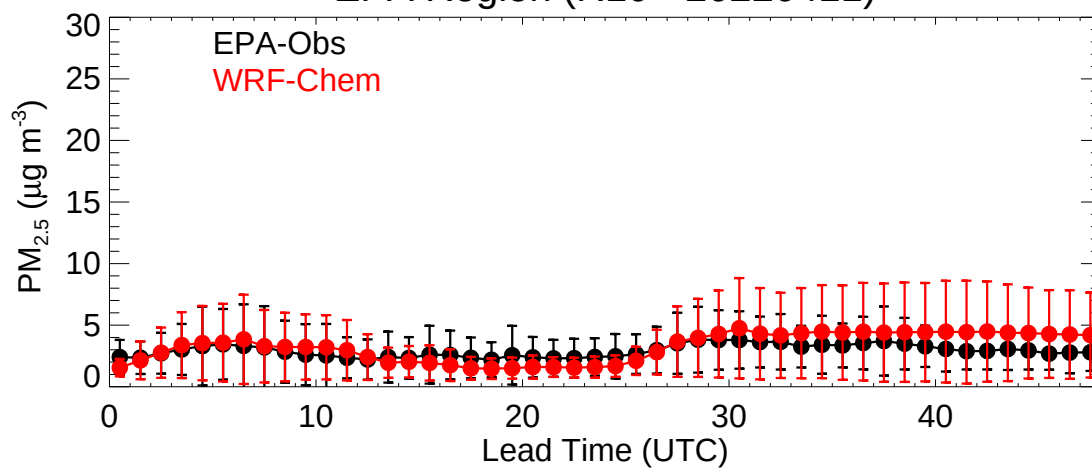
Colorado (20220411)
