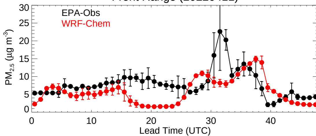
Front Range (20220411)
