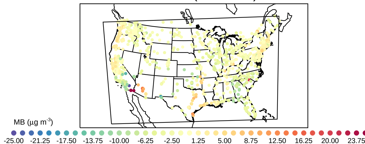
Mean Bias (20220411)
