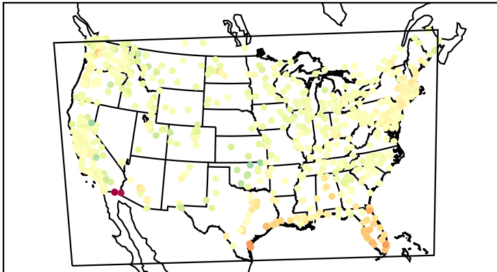
Mean Bias (20220416)
