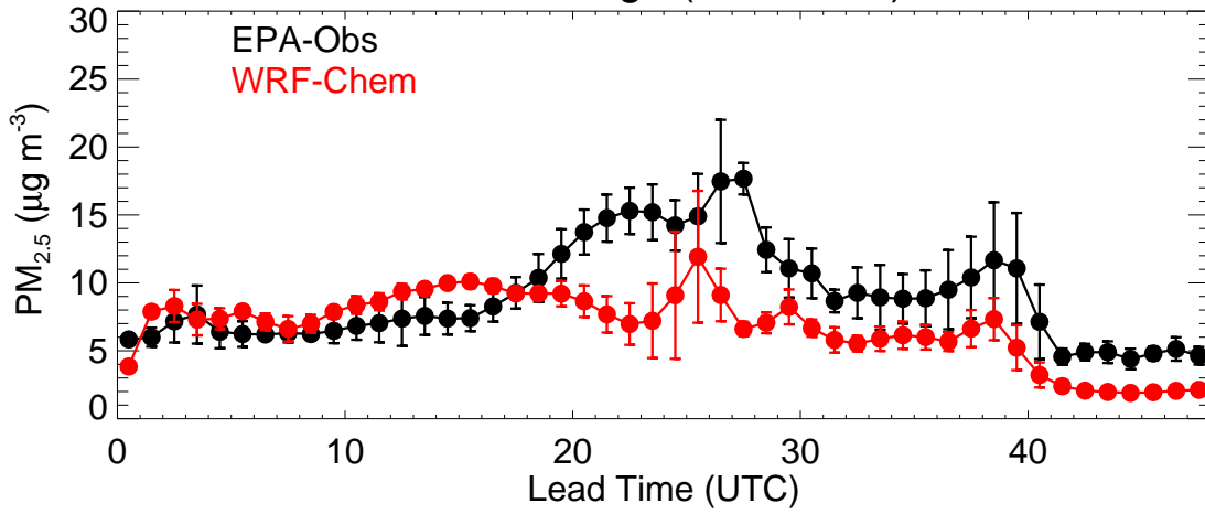
Front Range (20220416)
