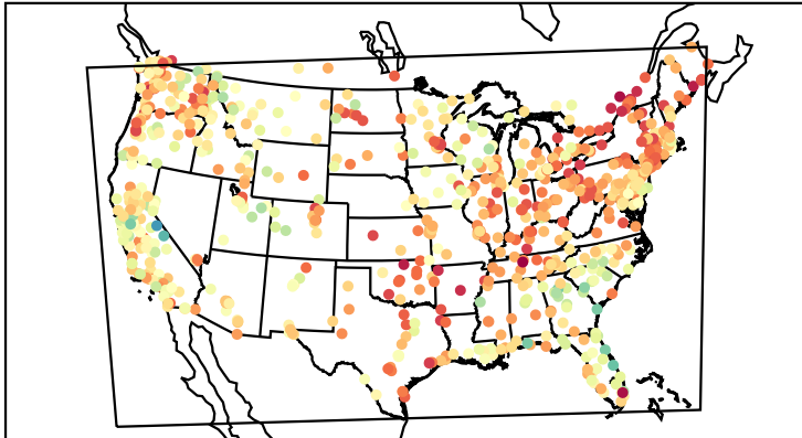
Correlation Coefficient (20220416)
