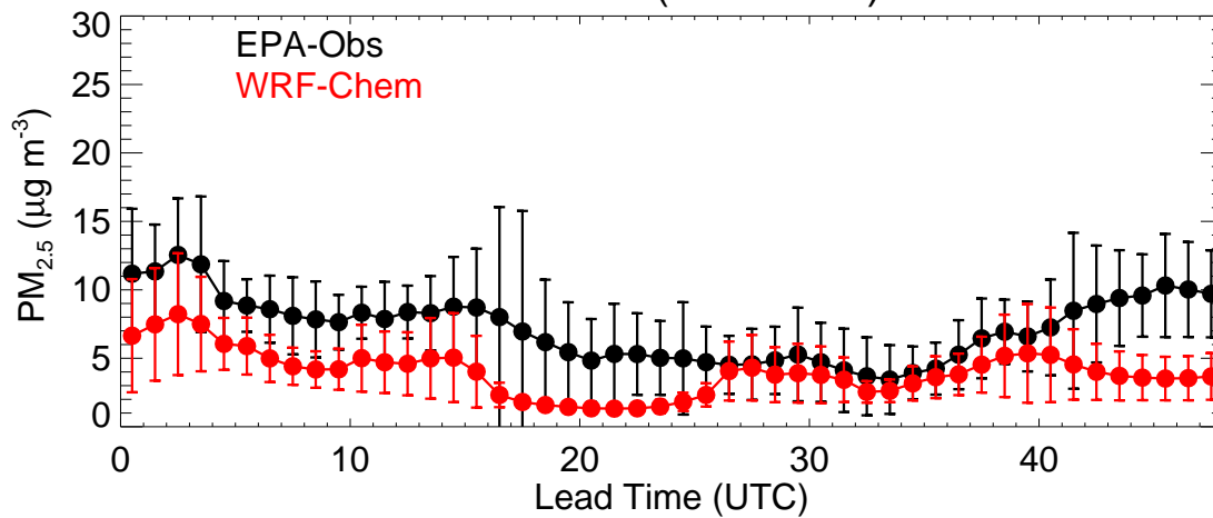
Colorado (20220417)
