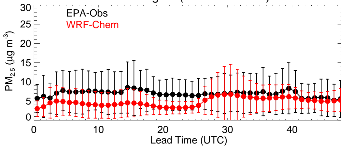
EPA Region (R10 - 20220418)
