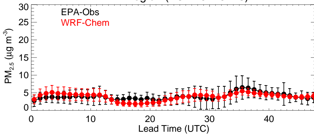
EPA Region (R4 - 20220418)
