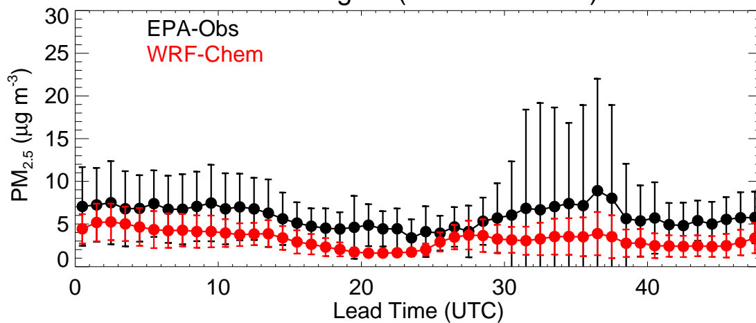
EPA Region (R8 - 20220418)
