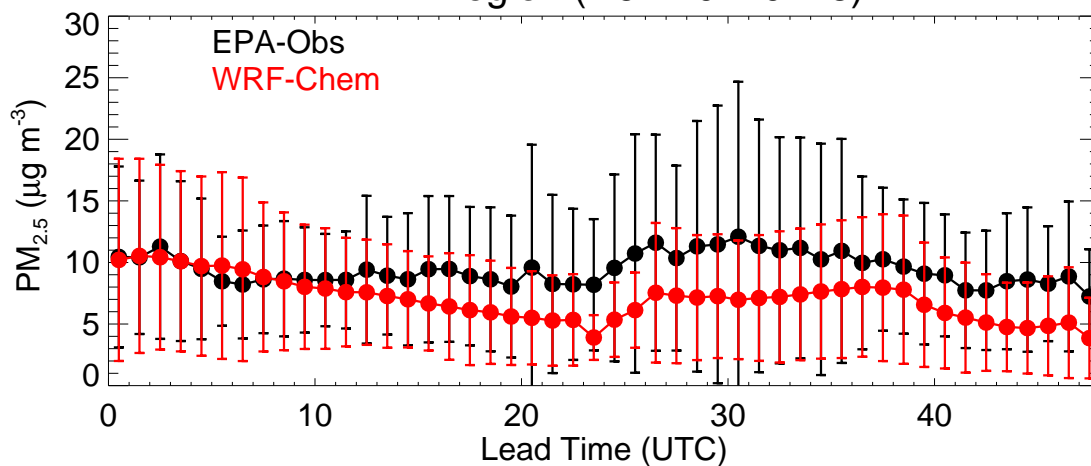
EPA Region (R7 - 20220418)
