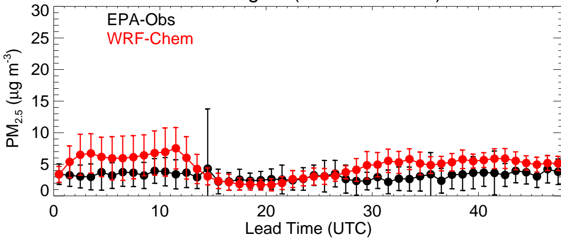
EPA Region (R2 - 20220418)
