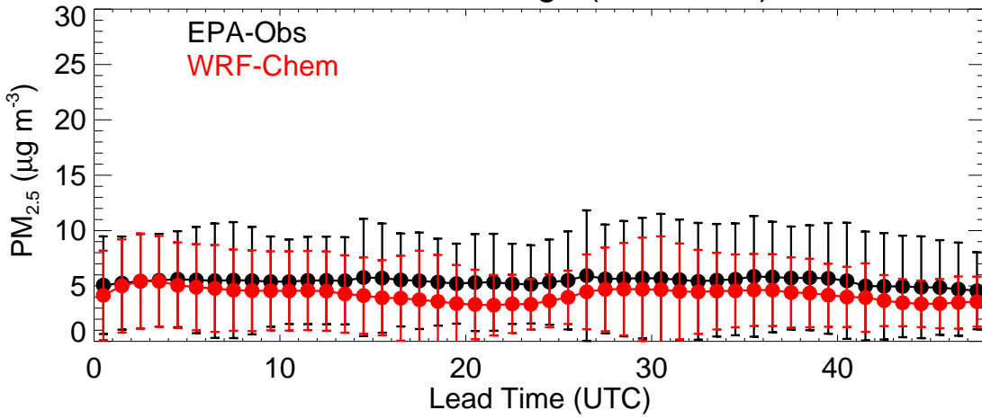
EPA Region (R1 - 20220418)
