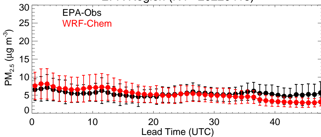
EPA Region (R5 - 20220418)
