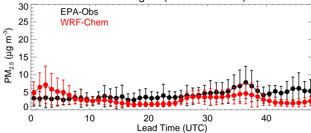
EPA Region (R8 - 20220425)
