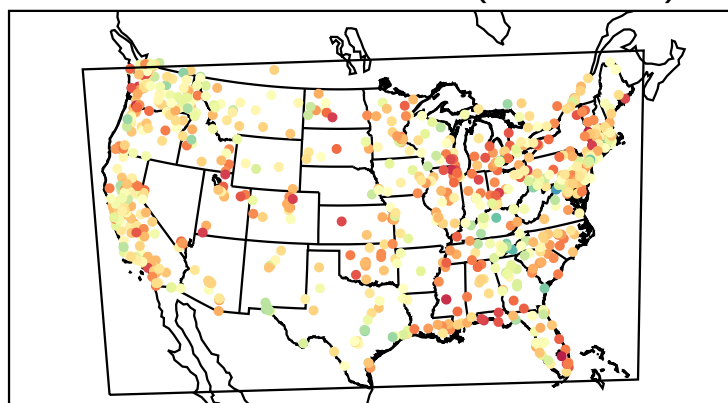
Correlation Coefficient (20220524)
