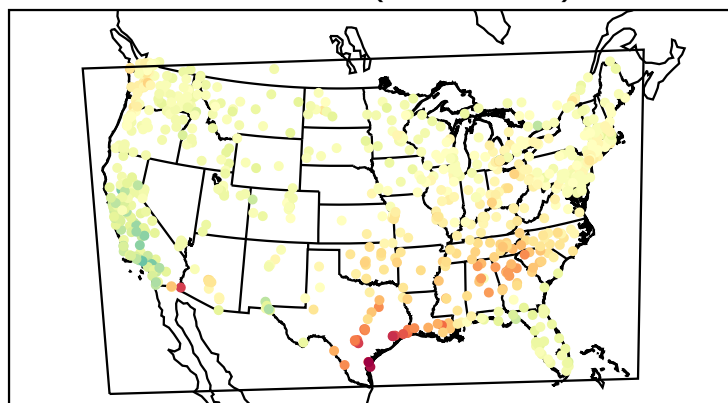
Mean Bias (20220524)
