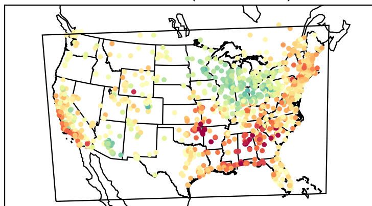
Mean Bias (20220622)
