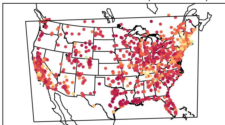
Correlation Coefficient (20220622)
