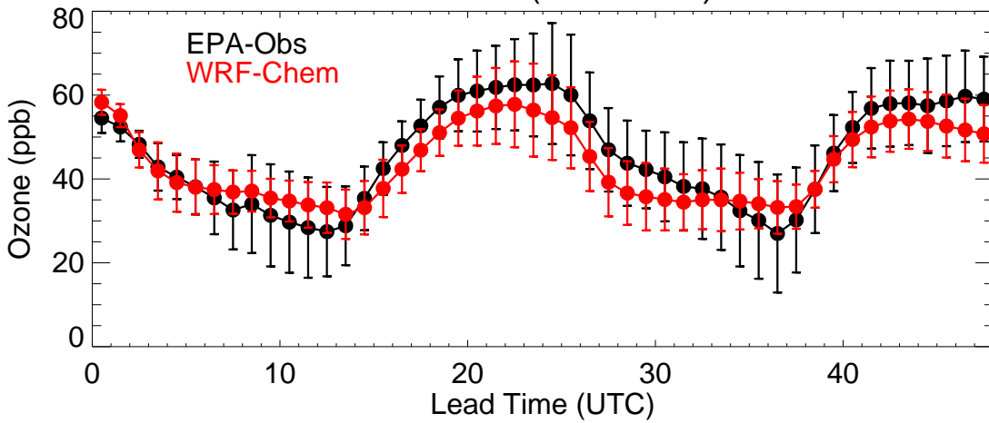
Colorado (20220622)
