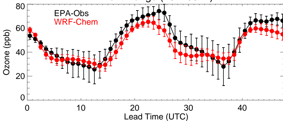
Front Range (20220622)
