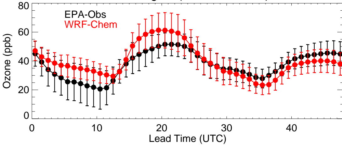
EPA Region (R5 - 20220711)
