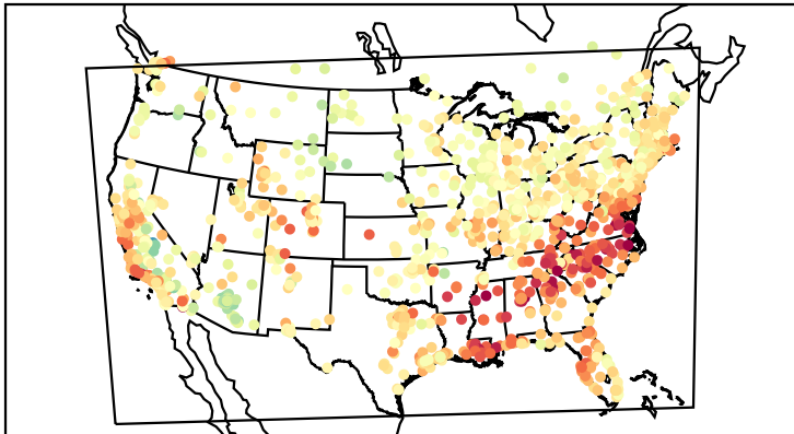
Mean Bias (20220713)
