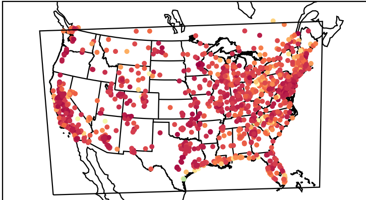
Correlation Coefficient (20220713)
