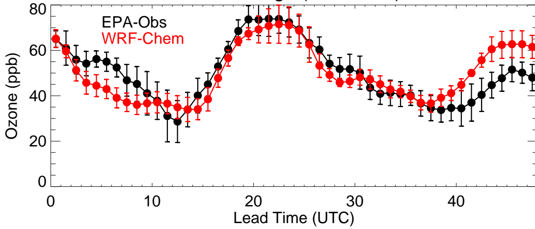
Front Range (20220727)
