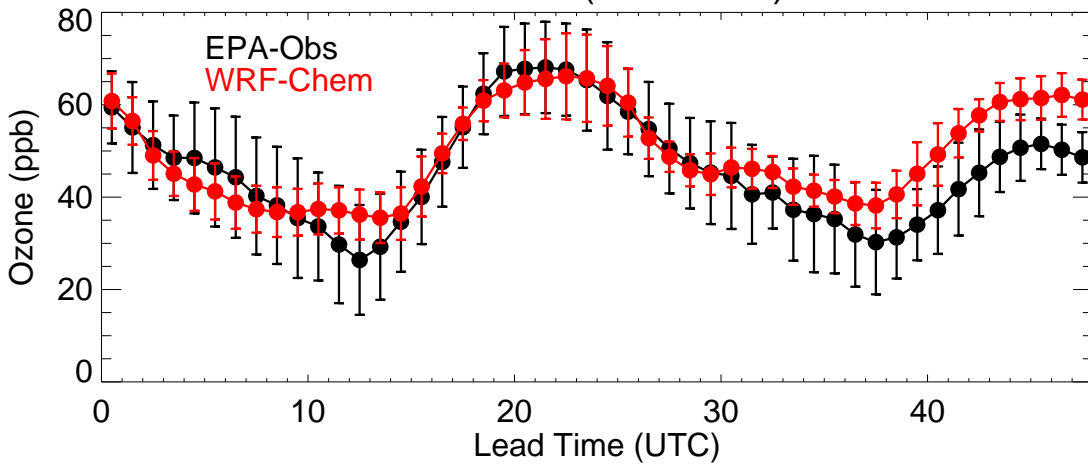
Colorado (20220727)
