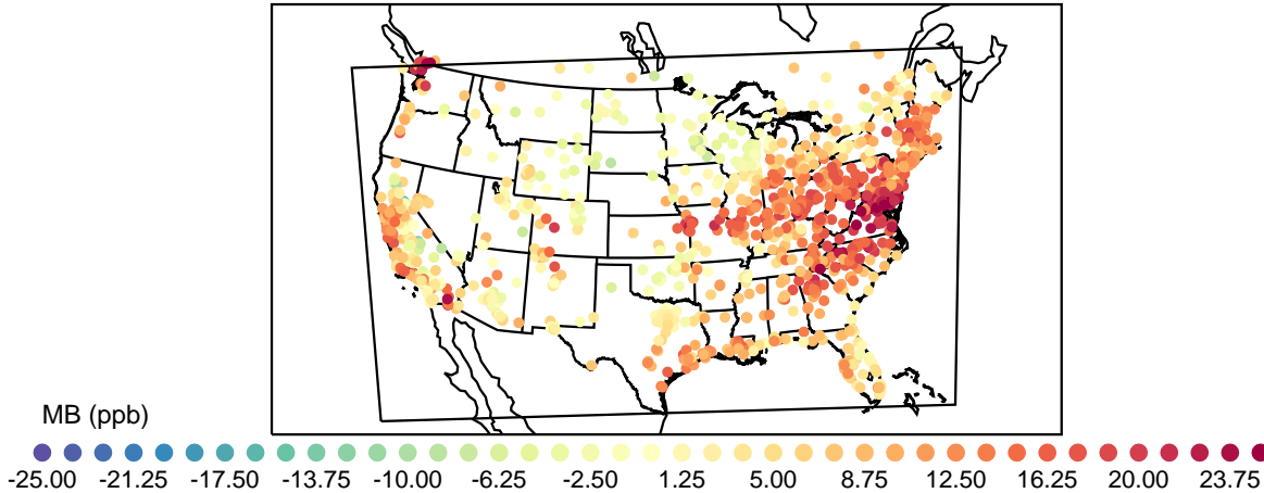
Mean Bias (20220727)
