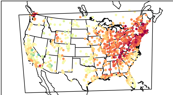
Mean Bias (20220806)
