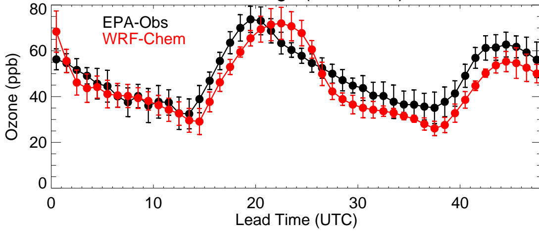
Front Range (20220806)
