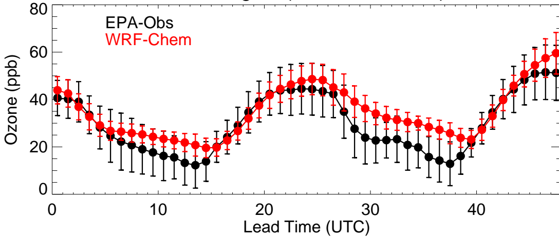
Colorado (20220806)
