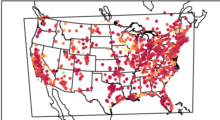
Correlation Coefficient (20220806)
