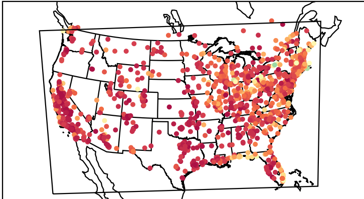
Correlation Coefficient (20220811)
