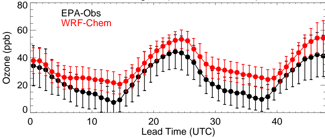
Colorado (20220811)
