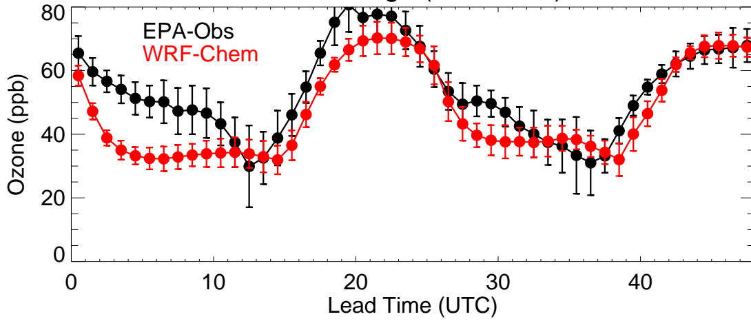
Front Range (20220811)
