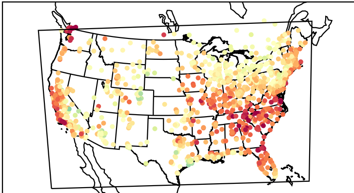
Mean Bias (20220811)
