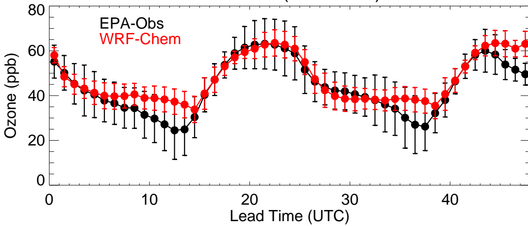
Colorado (20220824)
