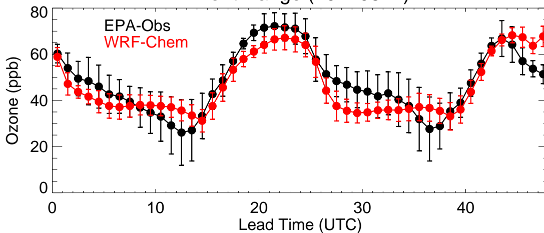
Front Range (20220824)
