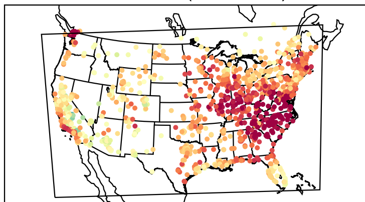
Mean Bias (20220824)
