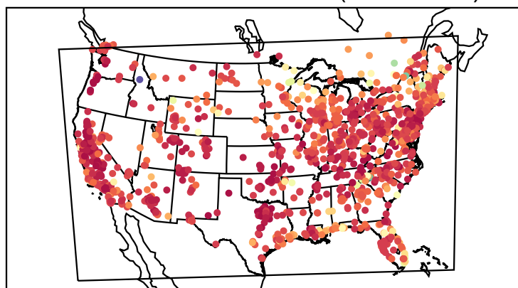
Correlation Coefficient (20220824)
