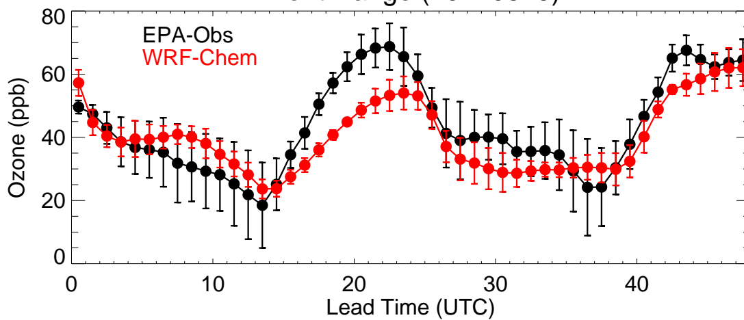
Front Range (20220829)
