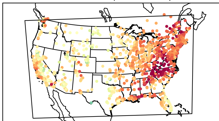
Mean Bias (20220829)
