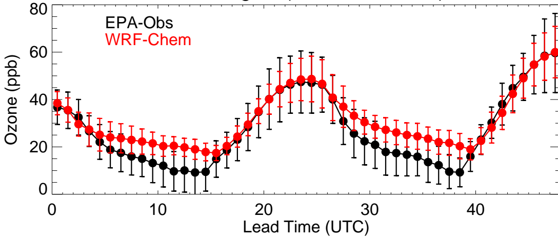
Colorado (20220829)
