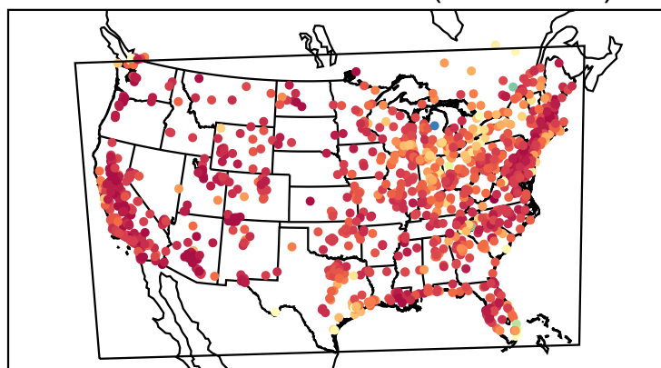
Correlation Coefficient (20220829)
