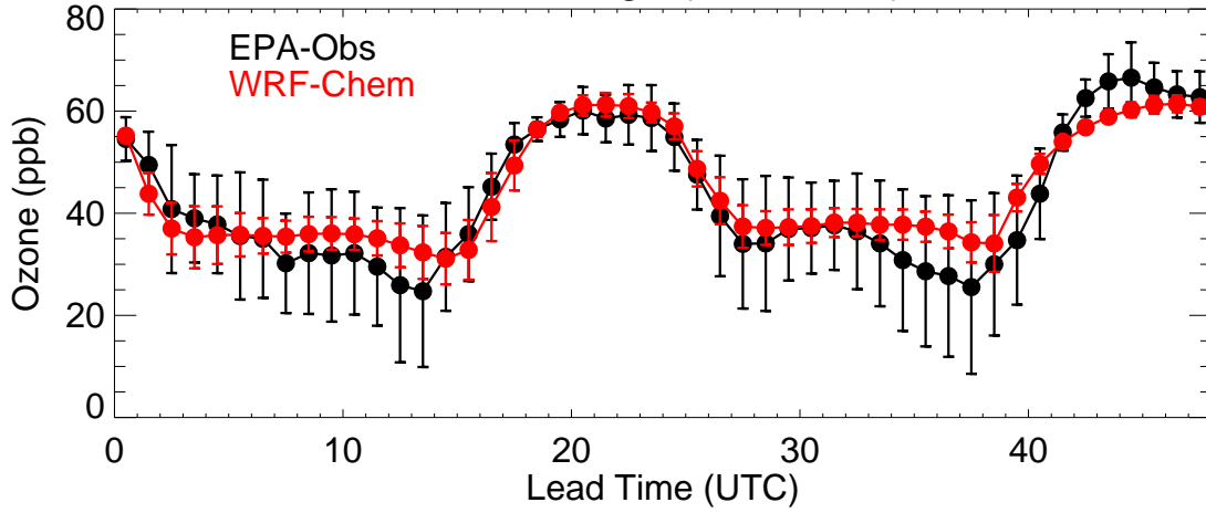
Front Range (20220901)
