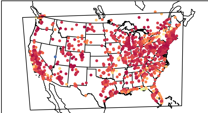
Correlation Coefficient (20220901)
