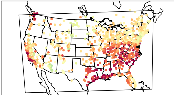
Mean Bias (20220901)
