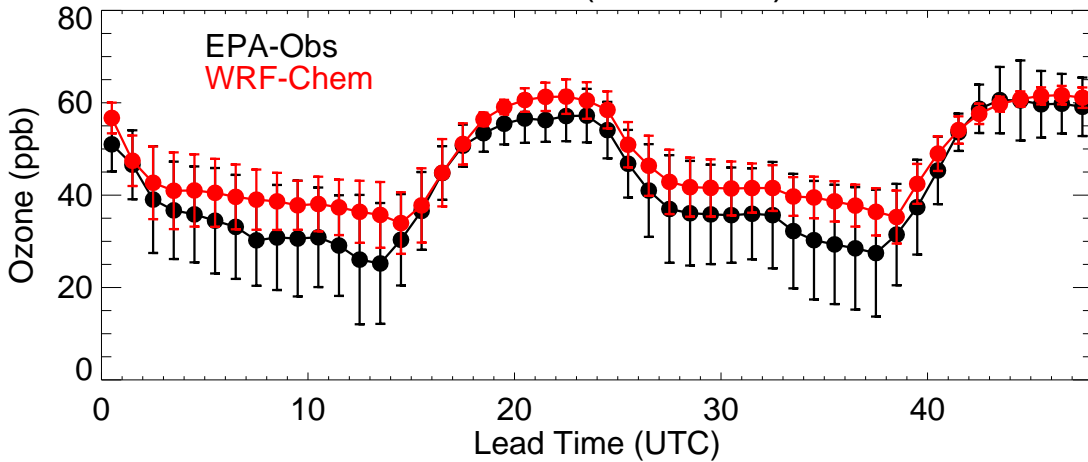
Colorado (20220901)
