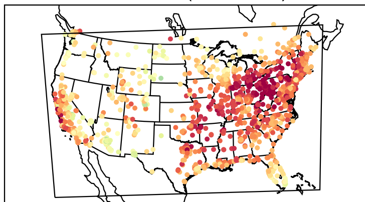
Mean Bias (20220904)
