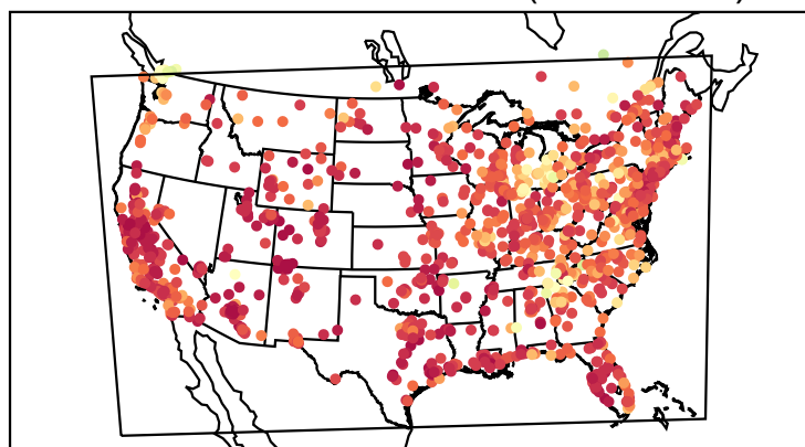
Correlation Coefficient (20220904)
