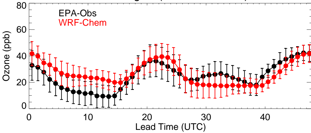
Colorado (20220904)
