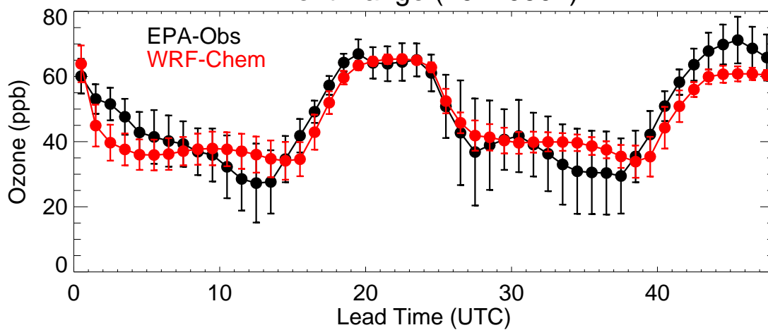
Front Range (20220904)
