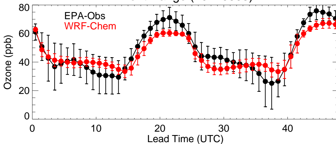
Front Range (20220905)
