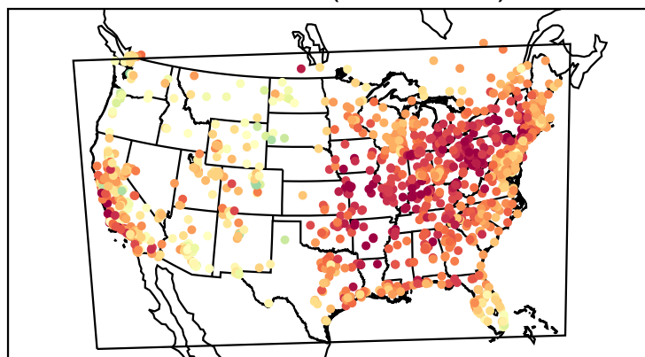
Mean Bias (20220905)
