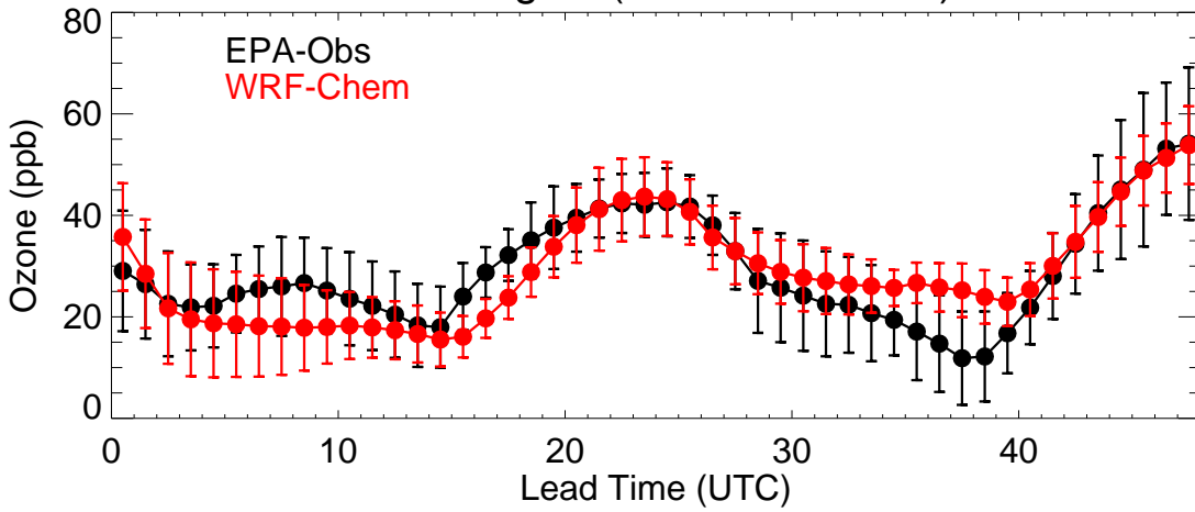
Colorado (20220905)
