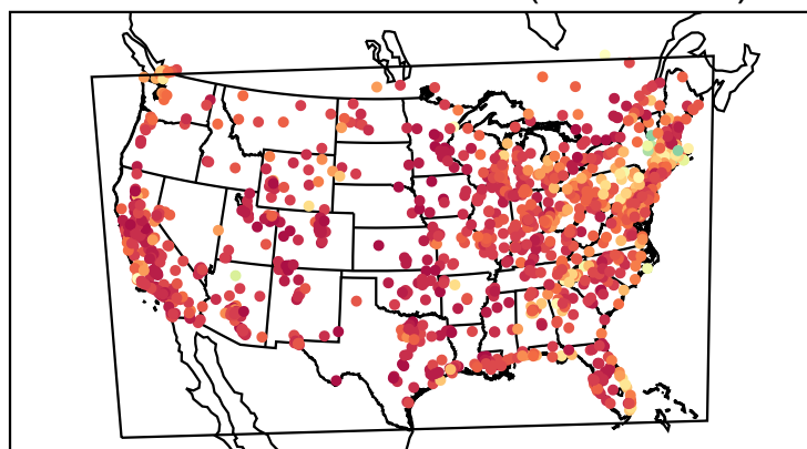
Correlation Coefficient (20220905)
