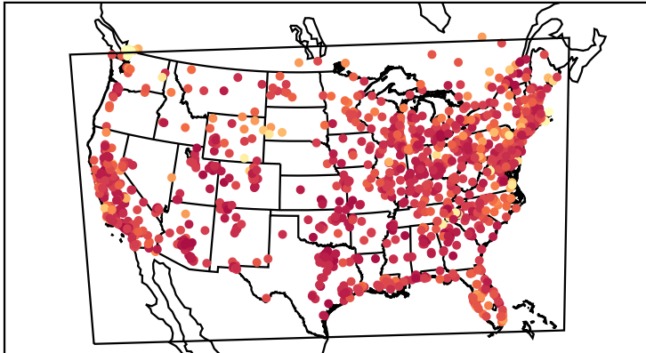
Correlation Coefficient (20220907)
