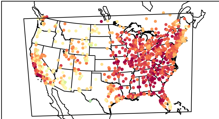
Mean Bias (20220907)
