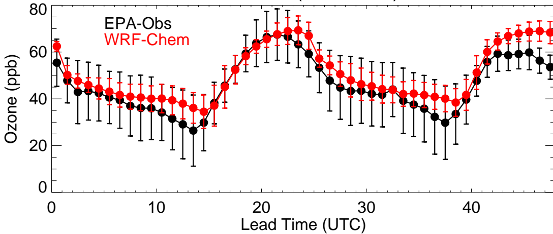
Colorado (20220907)
