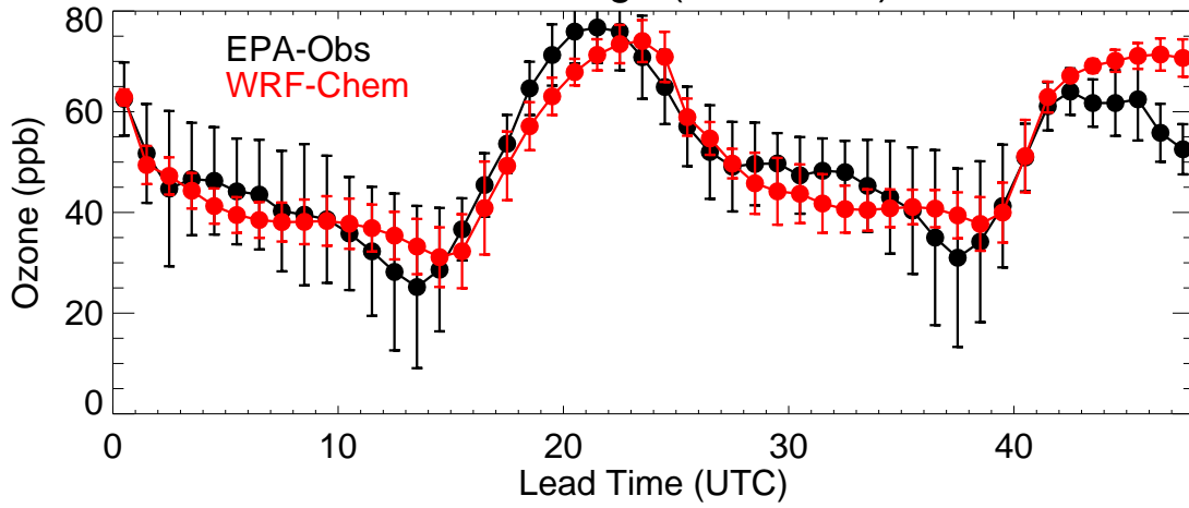
Front Range (20220907)
