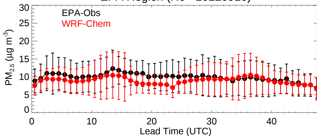
EPA Region (R7 - 20220910)
