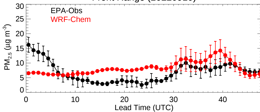
Front Range (20220910)
