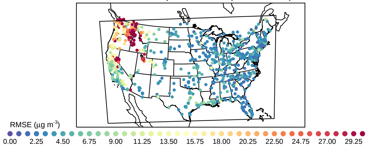
Root Mean Square Error (20220910)
