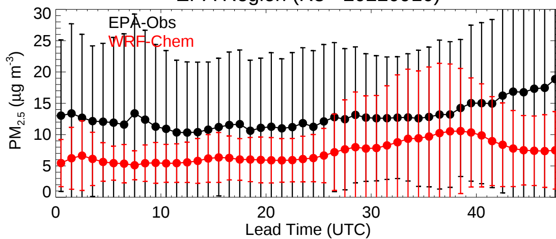
EPA Region (R8 - 20220910)
