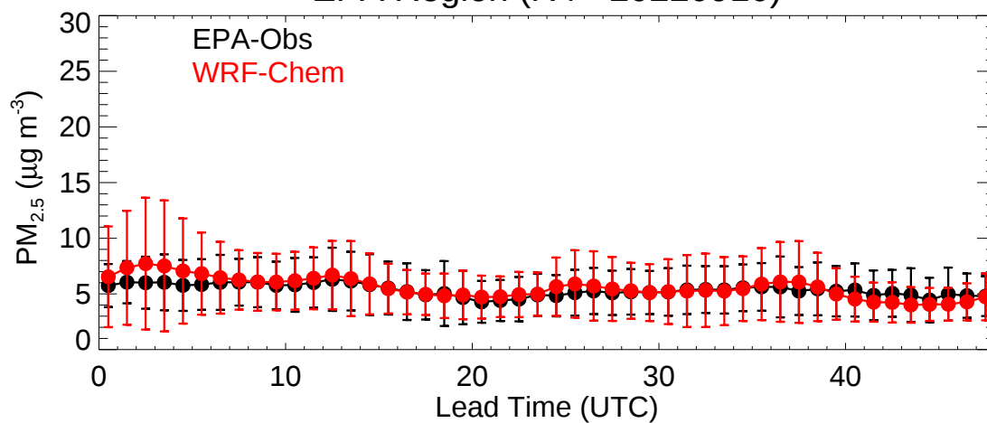
EPA Region (R5 - 20220910)
