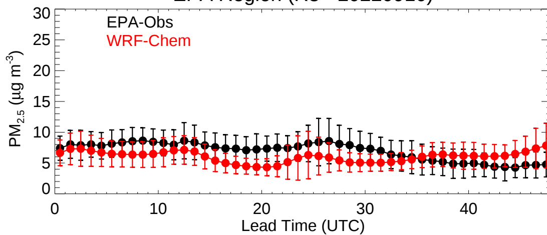
EPA Region (R4 - 20220910)
