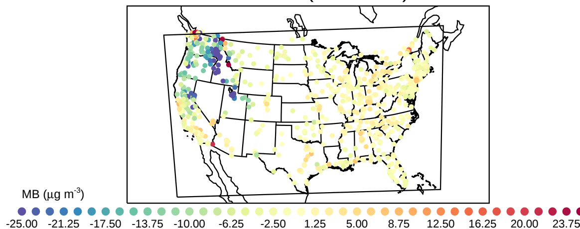
Mean Bias (20220910)
