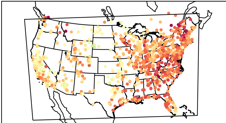
Mean Bias (20220913)
