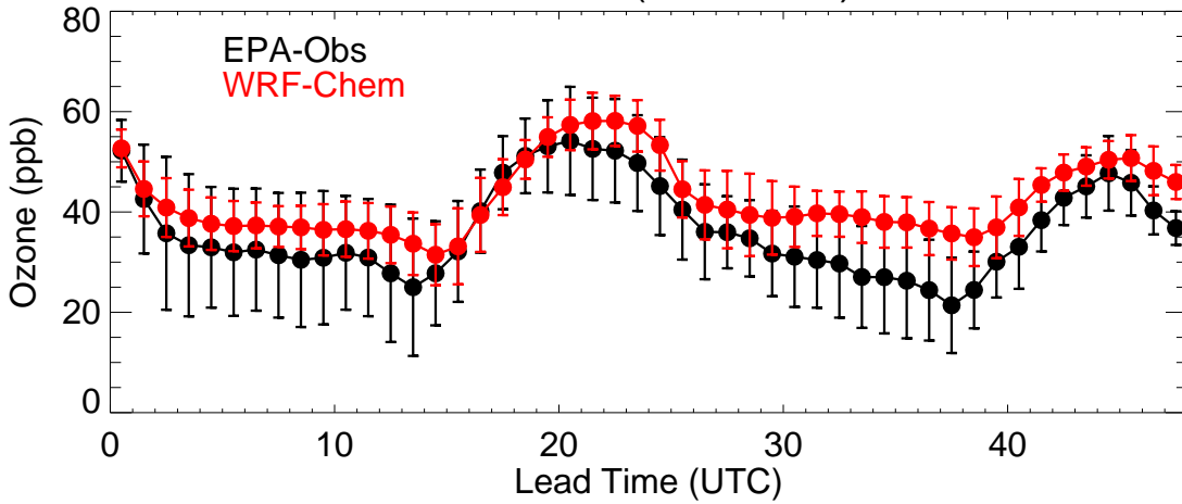
Colorado (20220913)
