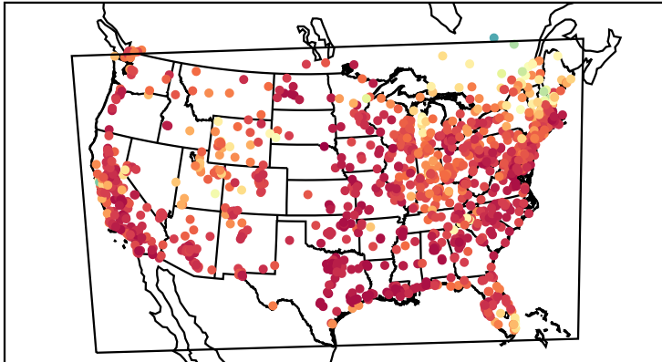
Correlation Coefficient (20220913)
