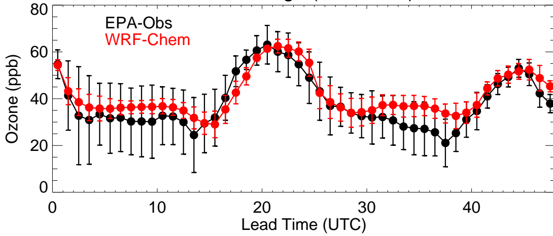
Front Range (20220913)
