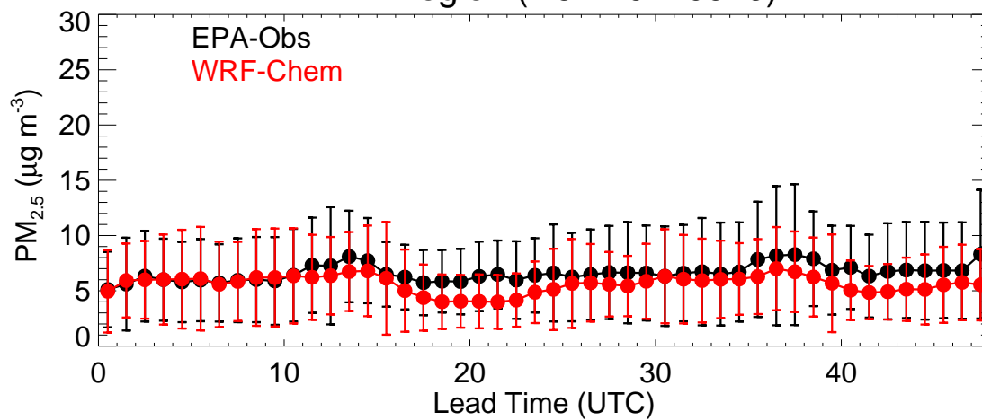
EPA Region (R7 - 20220919)
