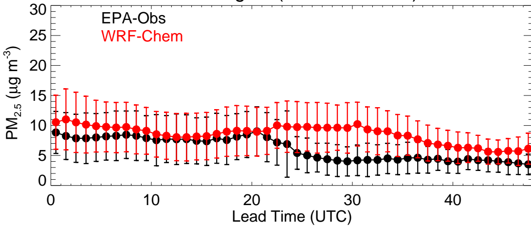
EPA Region (R2 - 20220919)
