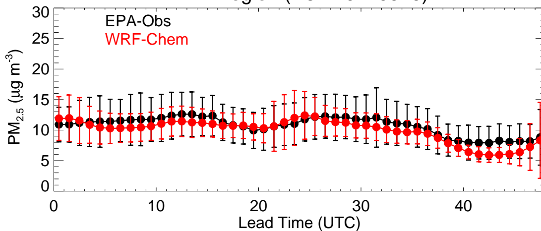
EPA Region (R4 - 20220919)
