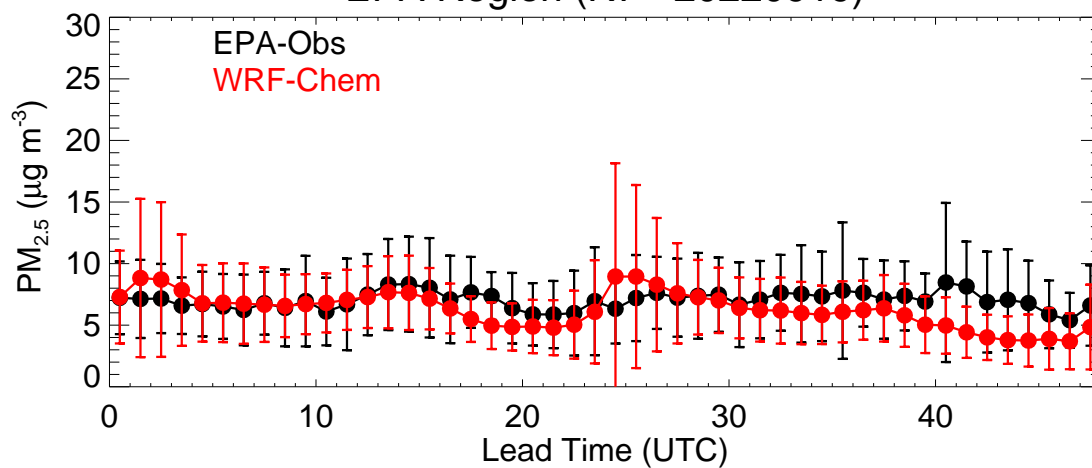
EPA Region (R8 - 20220919)
