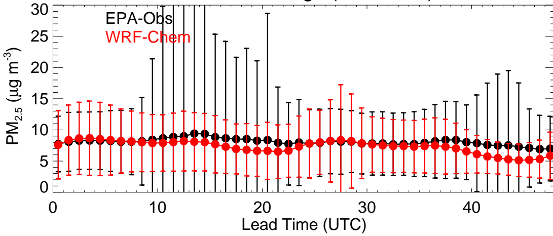
EPA Region (R1 - 20220919)
