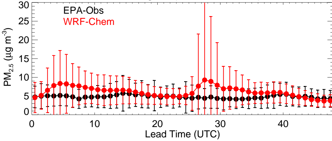
EPA Region (R10 - 20220919)
