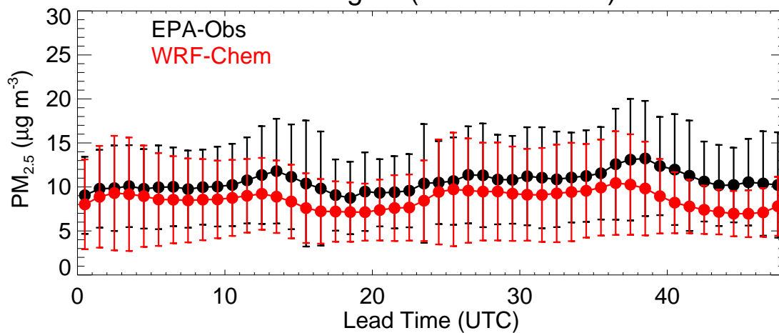
EPA Region (R5 - 20220919)
