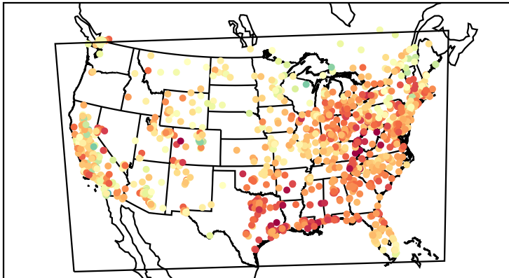
Mean Bias (20221030)
