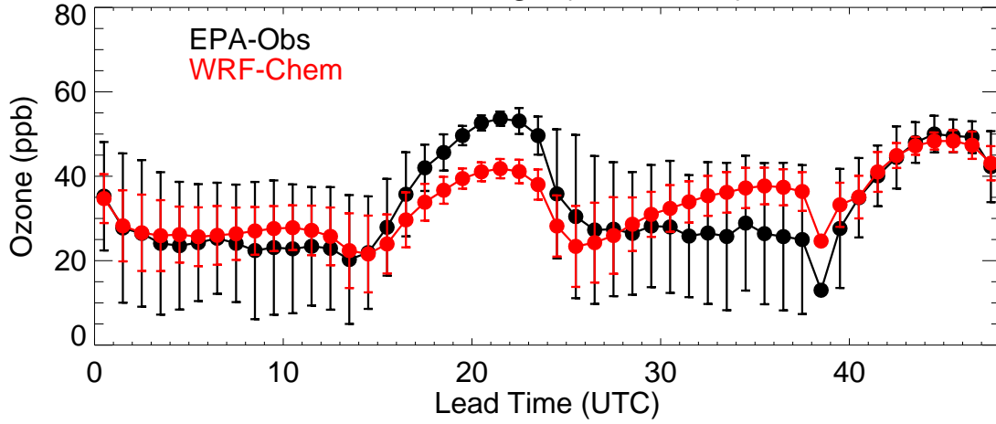
Front Range (20221030)
