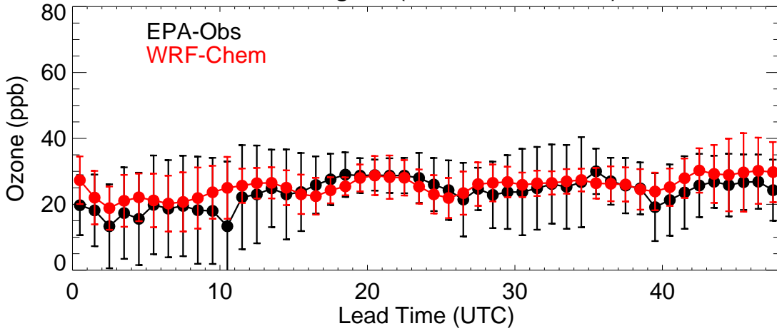
Colorado (20221030)
