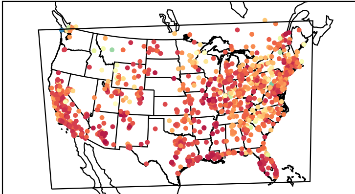
Correlation Coefficient (20221030)
