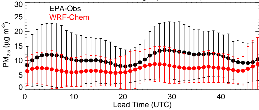
EPA Region (R1 - 20221121)
