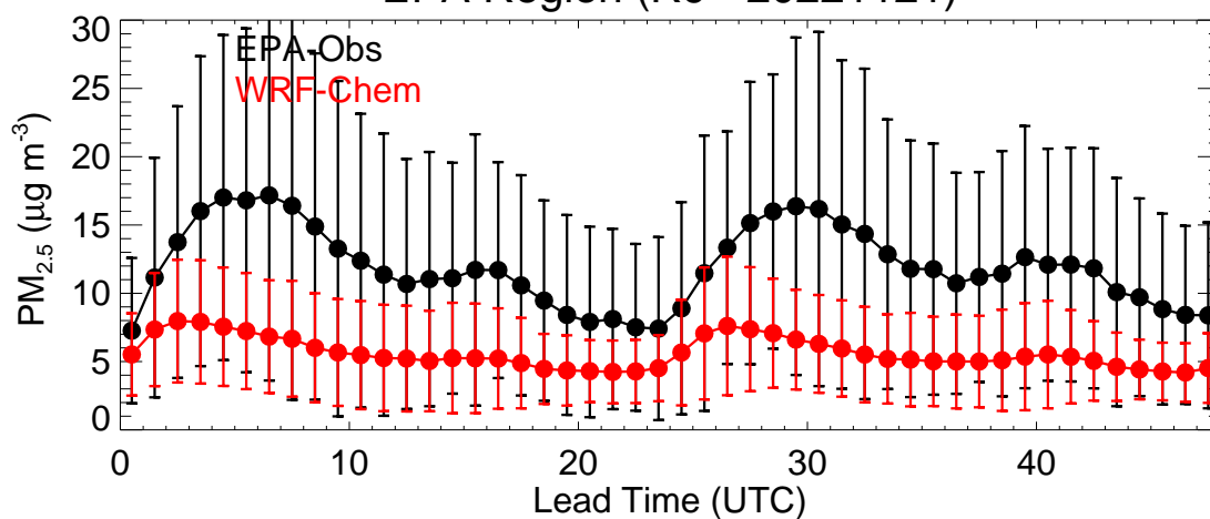
EPA Region (R10 - 20221121)
