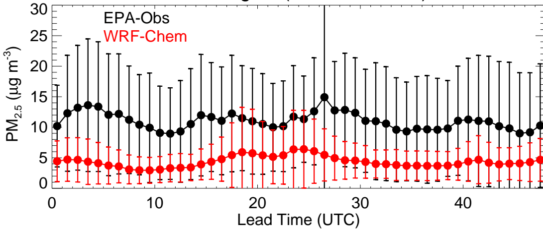
EPA Region (R8 - 20221121)
