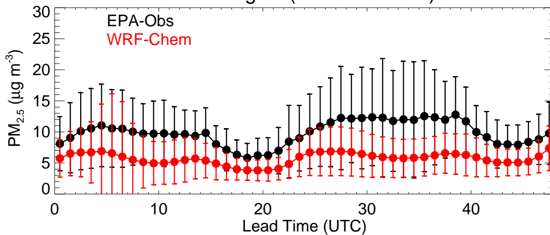
EPA Region (R5 - 20221121)
