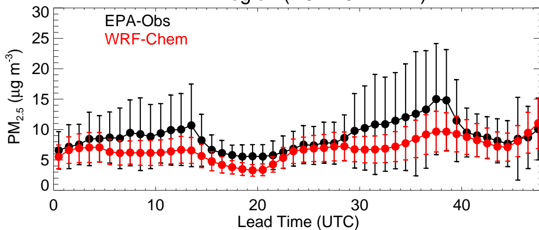
EPA Region (R4 - 20221121)
