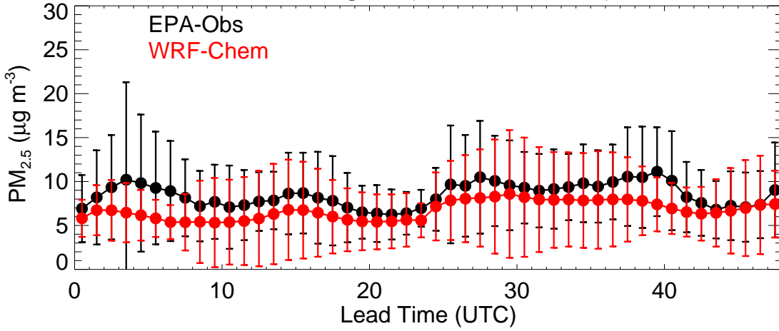
EPA Region (R7 - 20221121)
