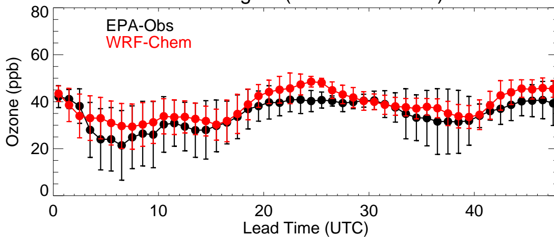
Colorado (20230330)
