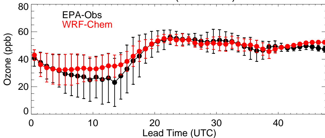
Colorado (20230330)
