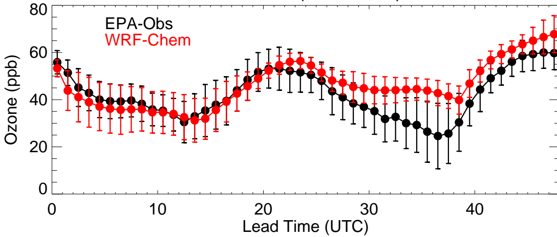
Colorado (20230502)
