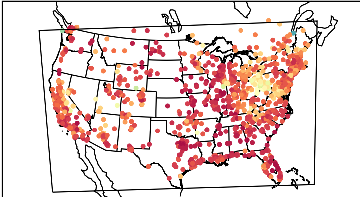
Correlation Coefficient (20230502)
