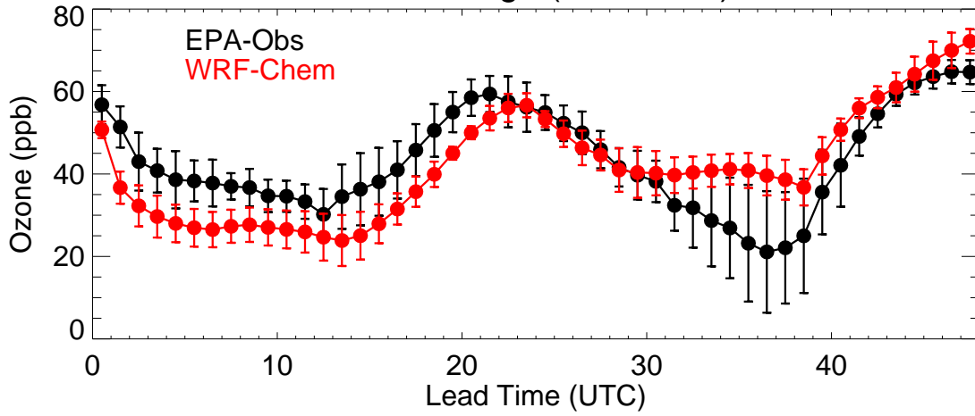
Front Range (20230502)
