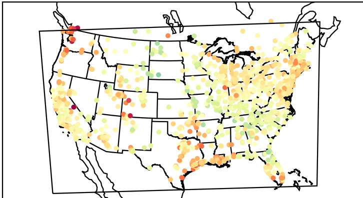
Mean Bias (20230502)
