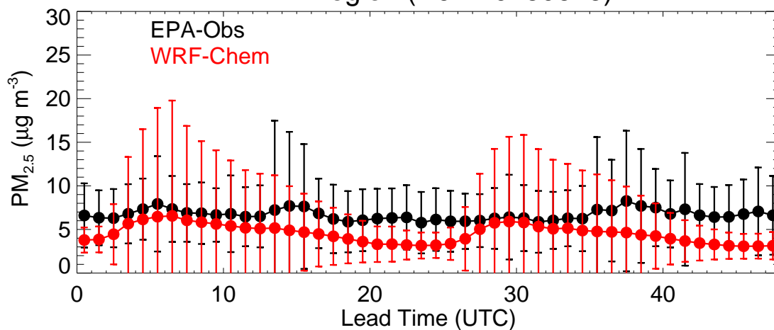
EPA Region (R10 - 20230625)
