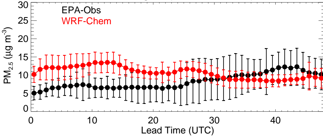
EPA Region (R4 - 20230625)
