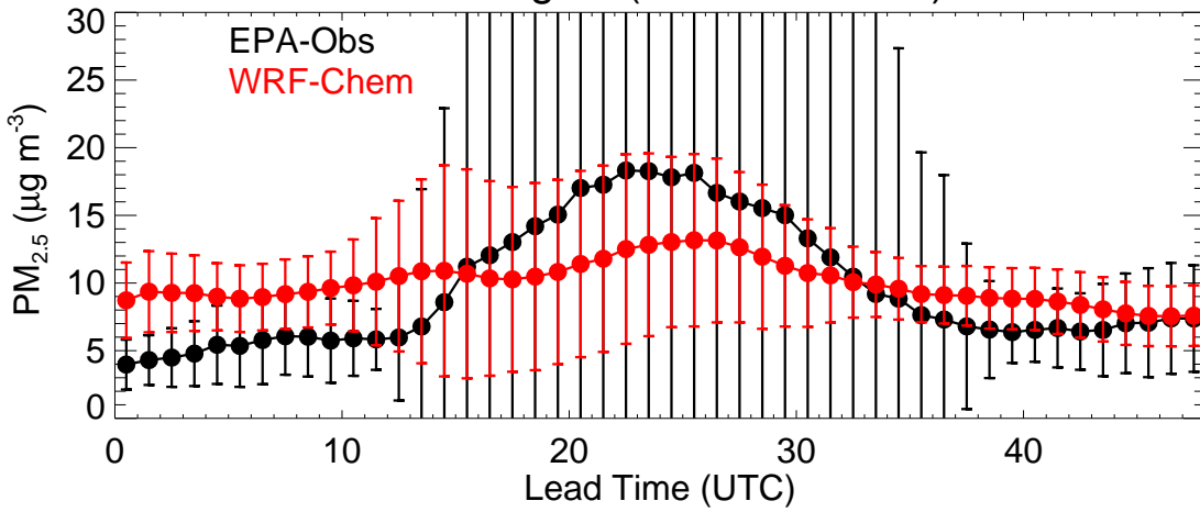
EPA Region (R2 - 20230625)
