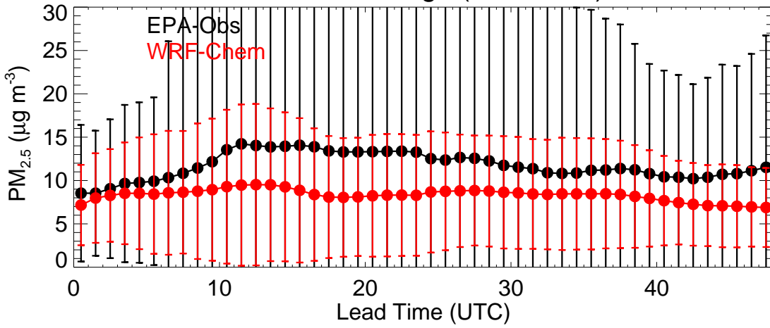
EPA Region (R1 - 20230625)
