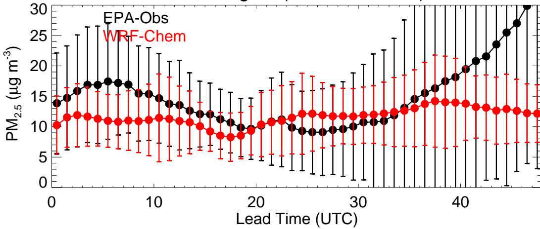
EPA Region (R5 - 20230625)
