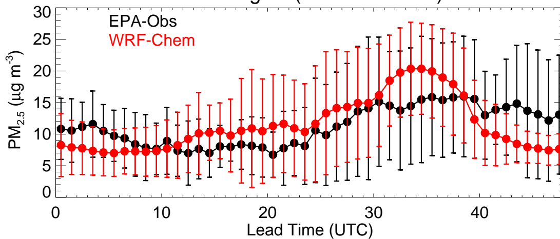
EPA Region (R8 - 20230625)
