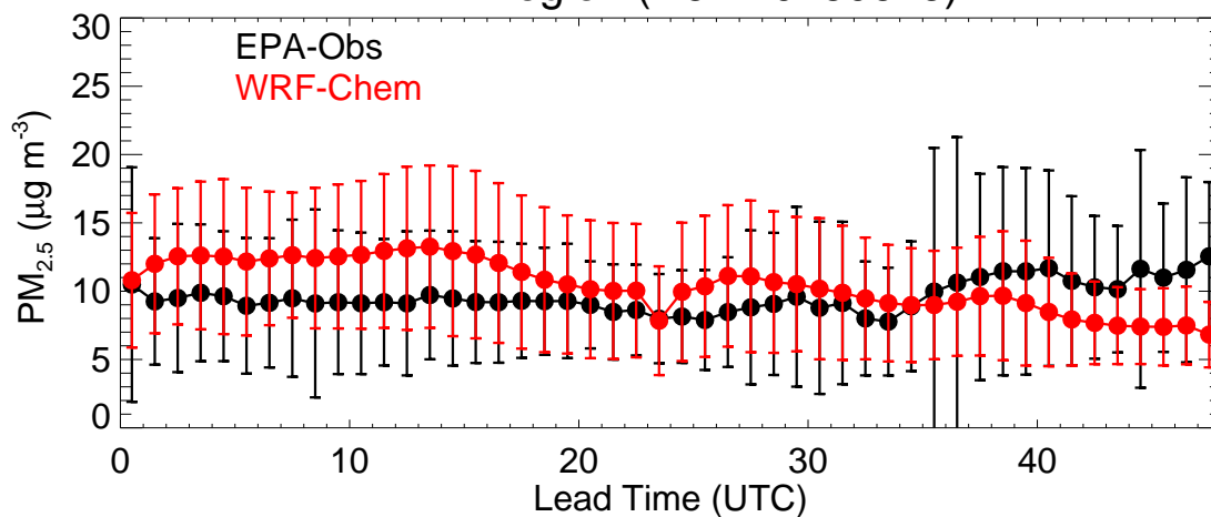
EPA Region (R7 - 20230625)
