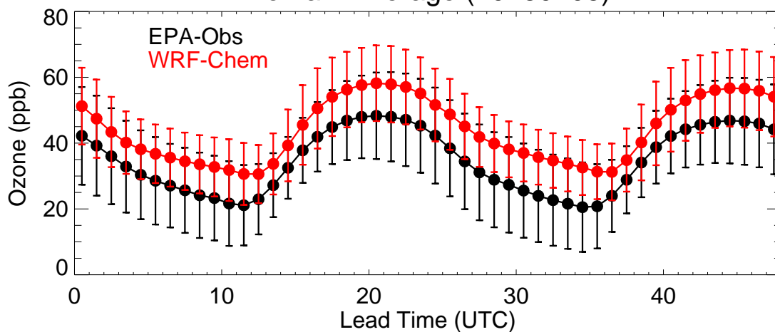
EPA Region (R1 - 20230703)
