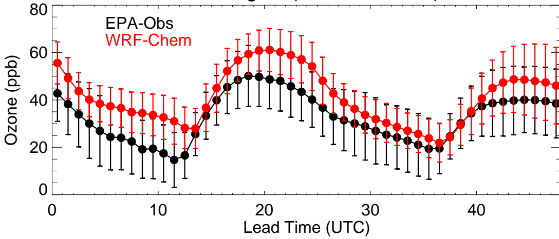
EPA Region (R7 - 20230703)
