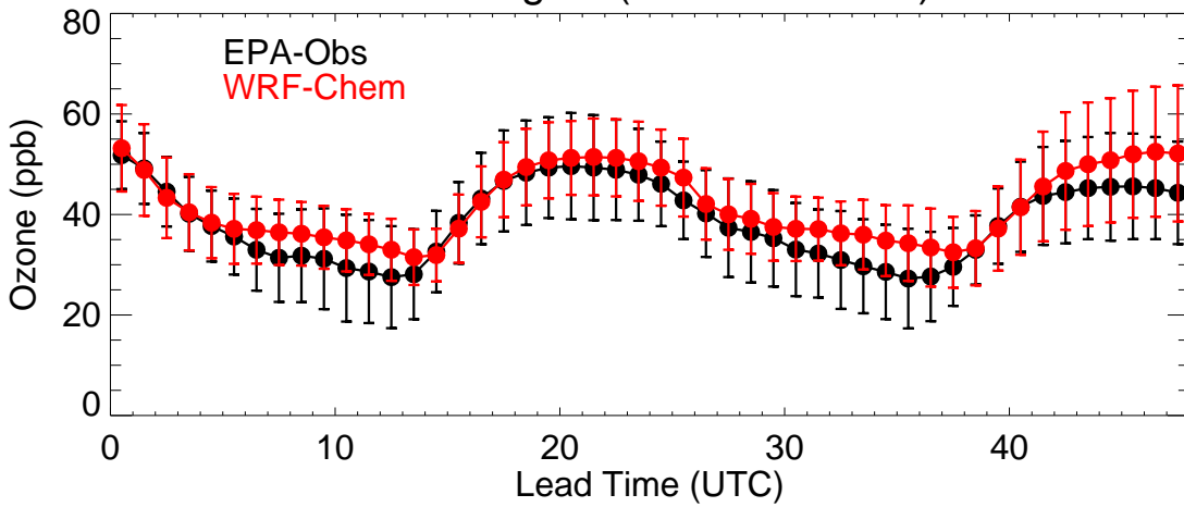
EPA Region (R8 - 20230703)
