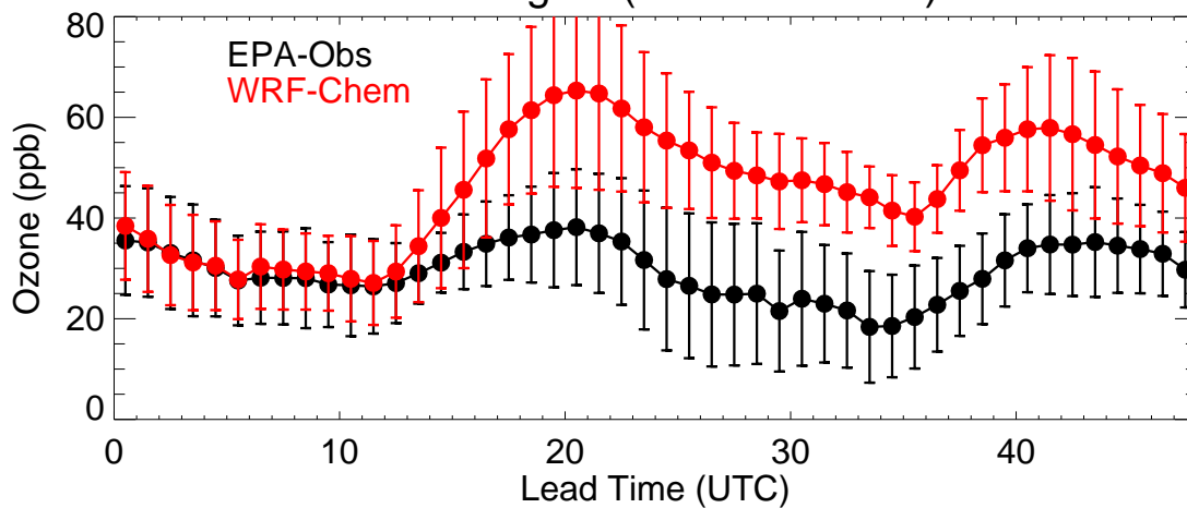
EPA Region (R2 - 20230703)
