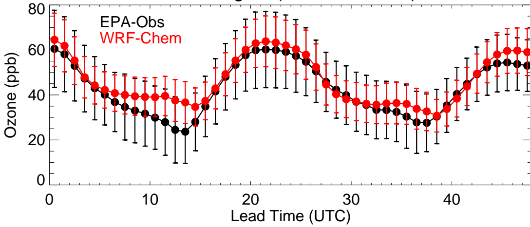
EPA Region (R10 - 20230703)
