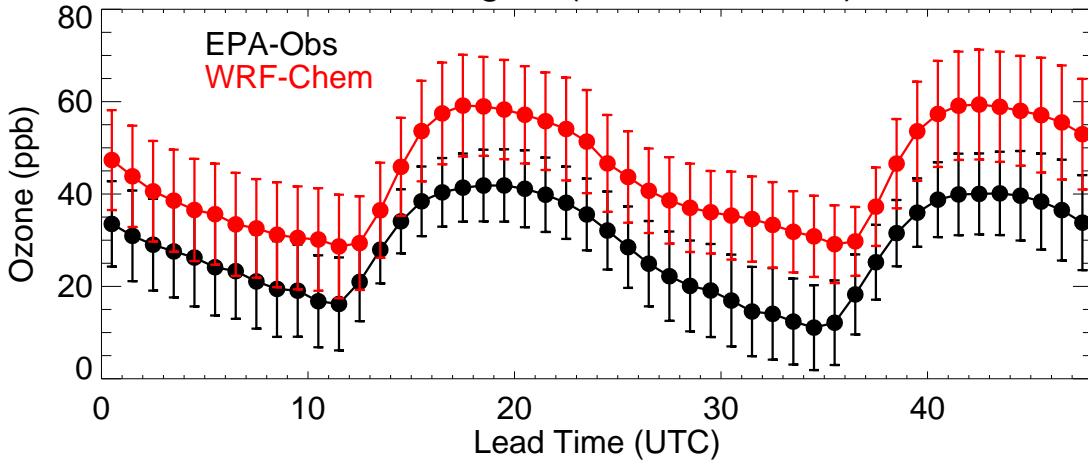
EPA Region (R5 - 20230703)
