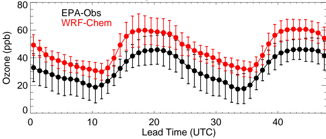
EPA Region (R4 - 20230703)
