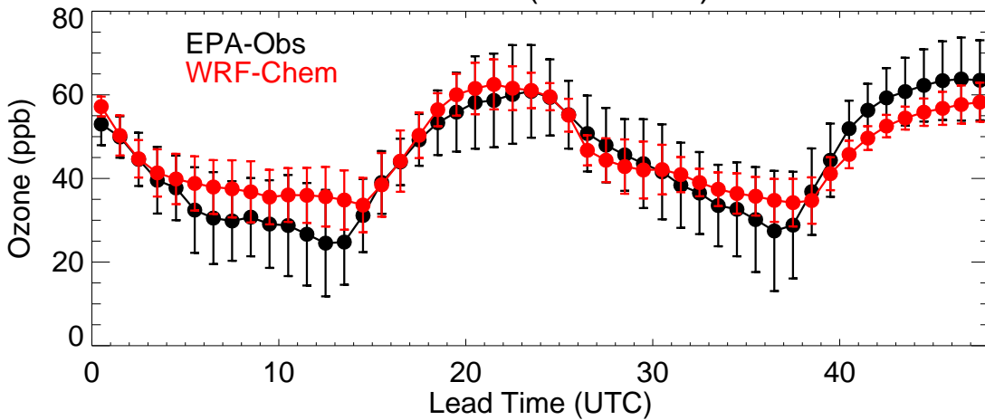
Colorado (20230808)
