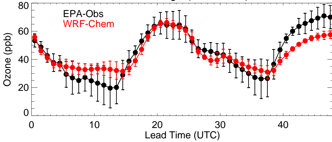
Front Range (20230808)
