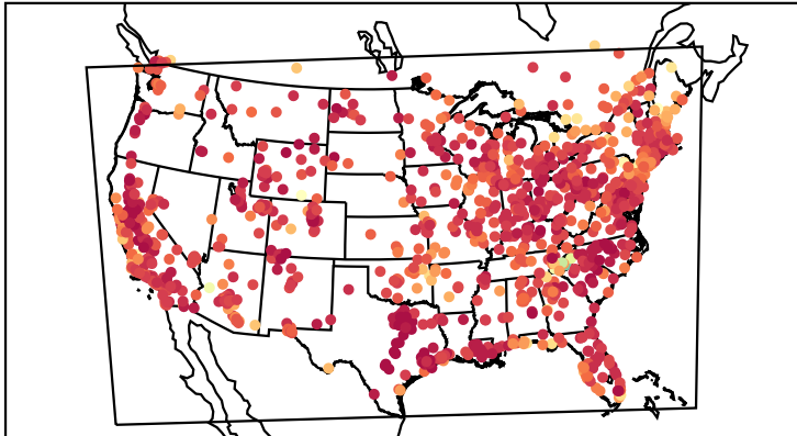
Correlation Coefficient (20230808)
