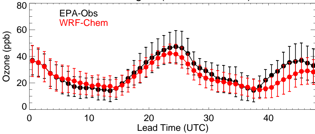
Colorado (20230808)
