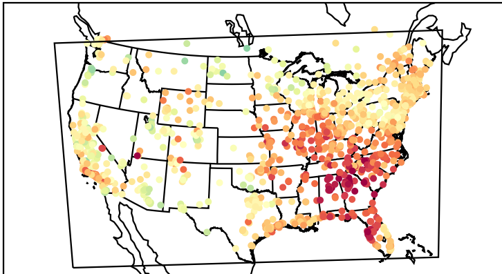
Mean Bias (20230808)
