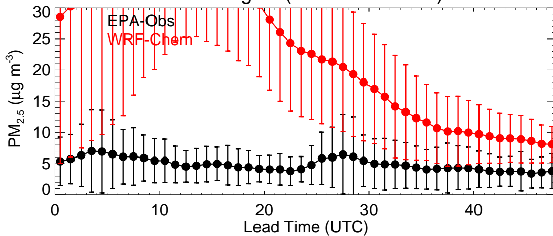
Colorado (20231105)
