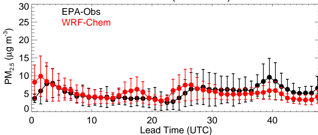
Colorado (20231105)
