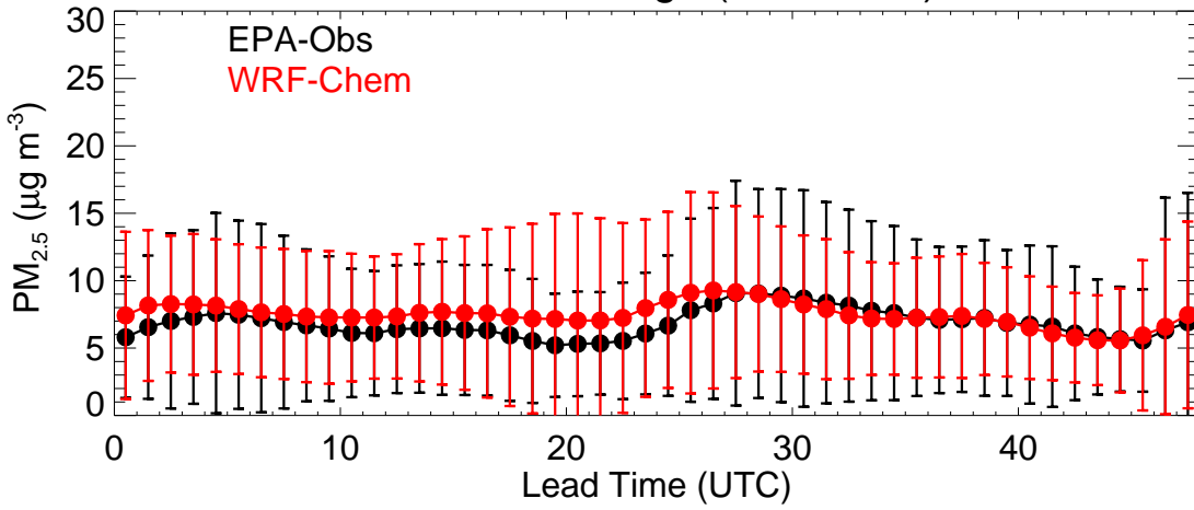
EPA Region (R1 - 20231122)
