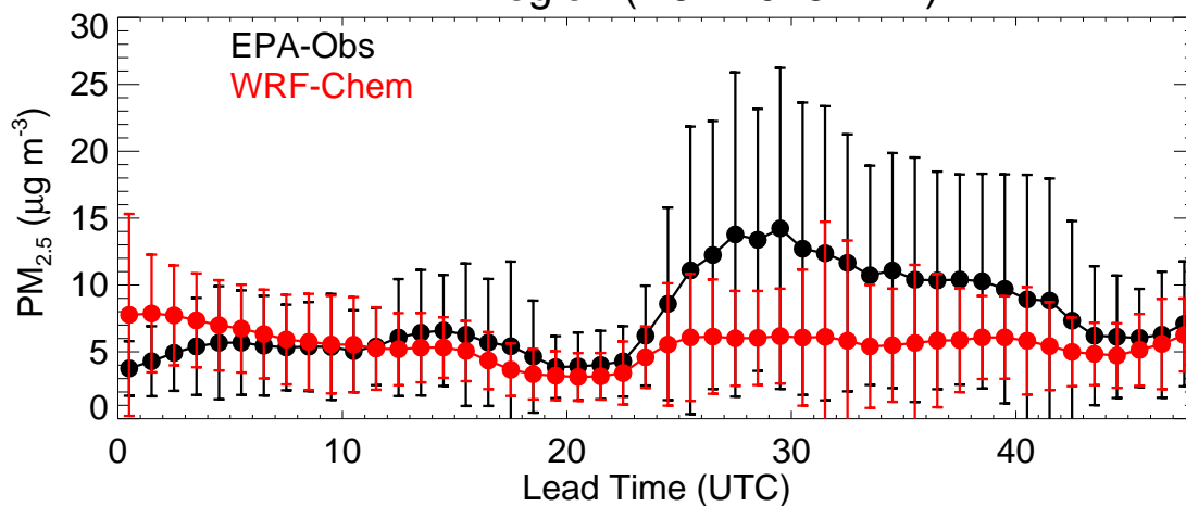
EPA Region (R7 - 20231122)
