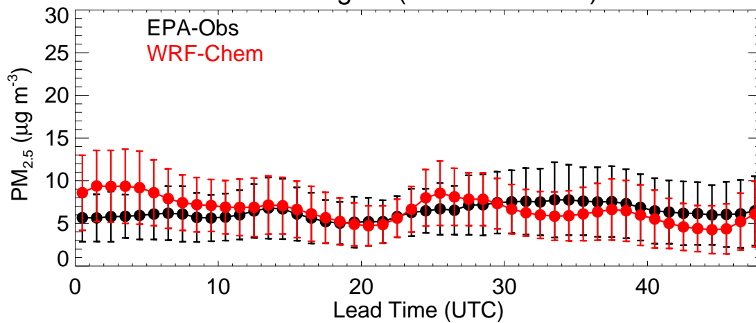
EPA Region (R5 - 20231122)
