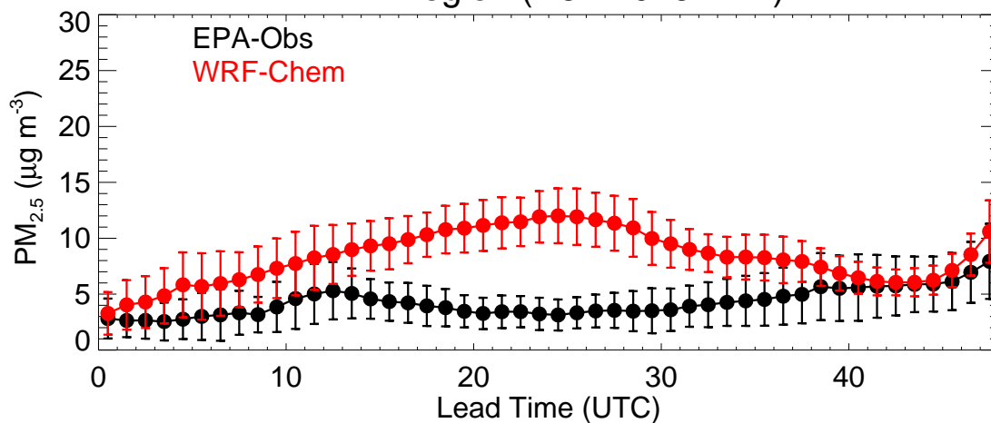
EPA Region (R4 - 20231122)
