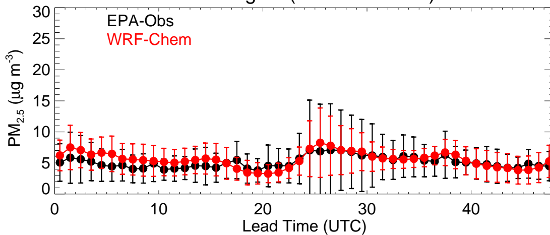
EPA Region (R8 - 20231122)
