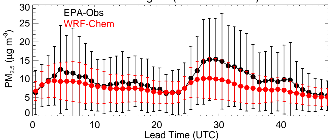
EPA Region (R10 - 20231122)
