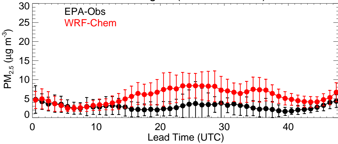
EPA Region (R2 - 20231122)
