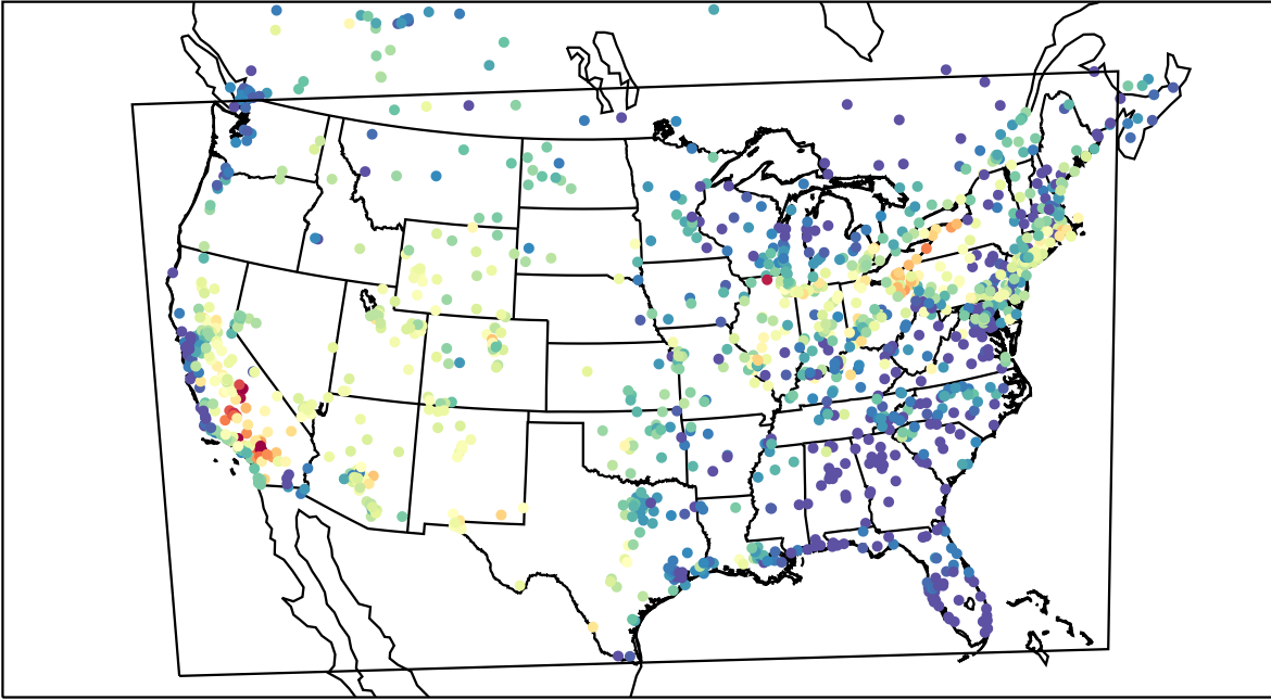
AirNOW (2019-07-14_02:00:00)
