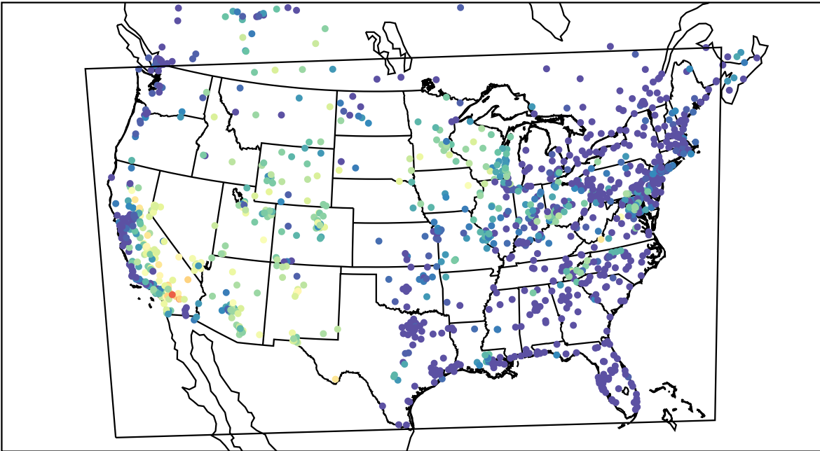
AirNOW (2019-07-15_05:00:00)
