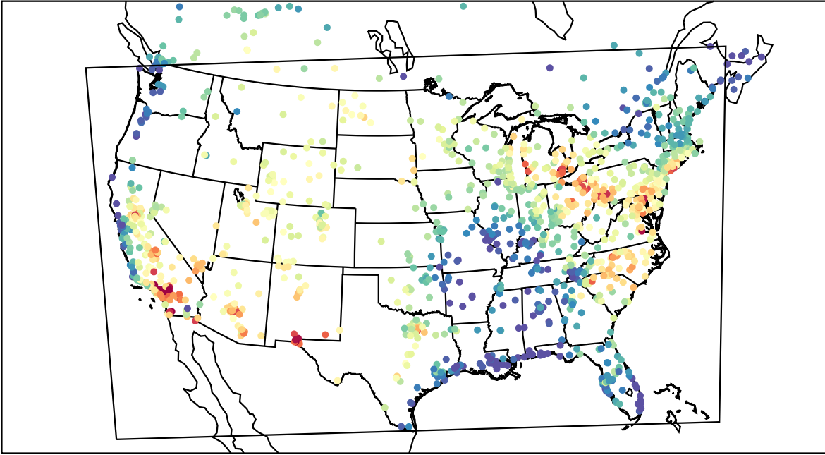
AirNOW (2019-07-15_21:00:00)
