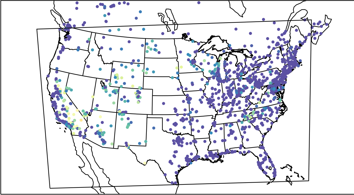
AirNOW (2019-07-15_11:00:00)
