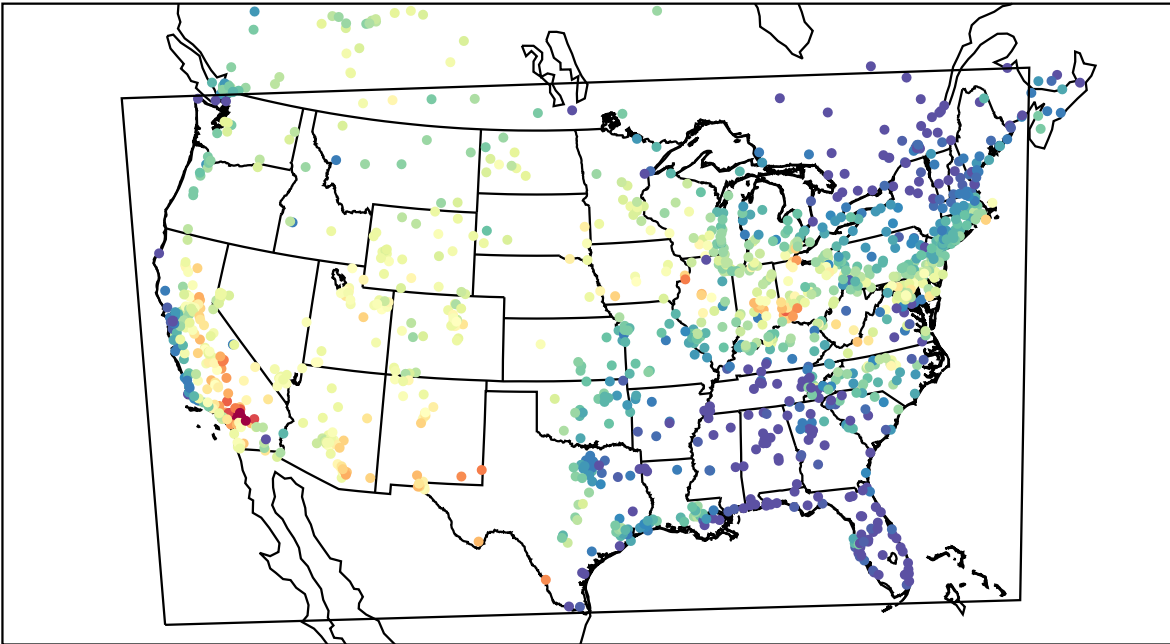
AirNOW (2019-07-15_00:00:00)
