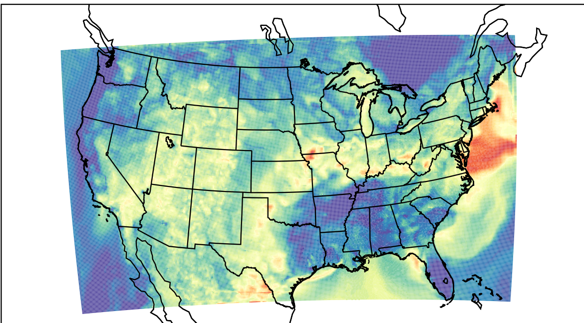
WRF (2019-07-14_05:00:00)
