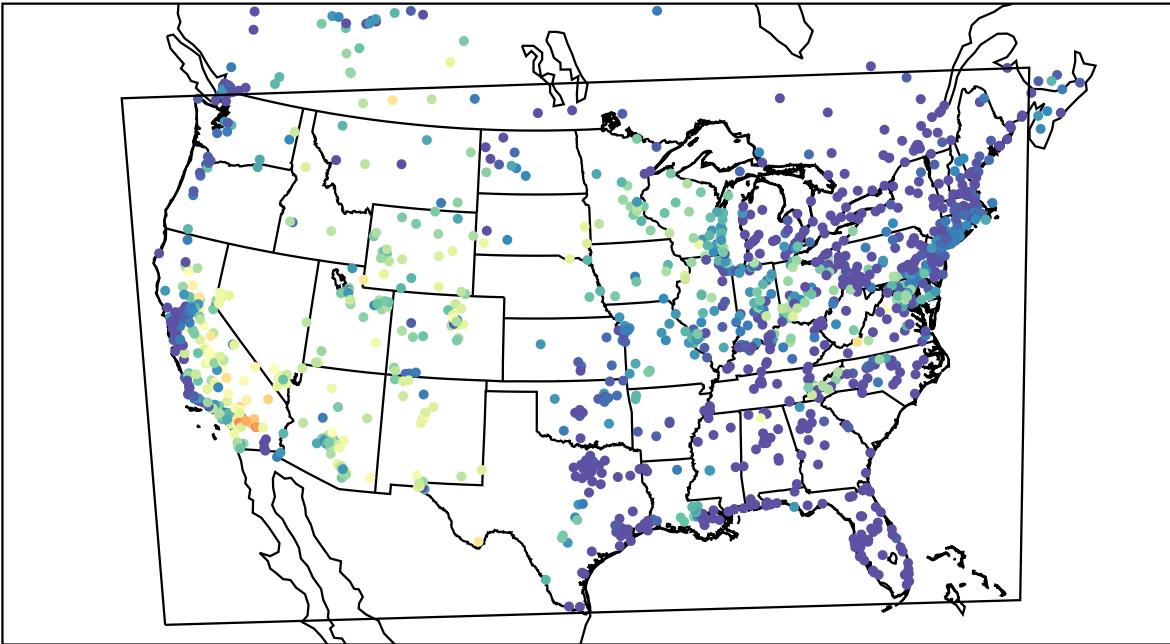
AirNOW (2019-07-15_04:00:00)
