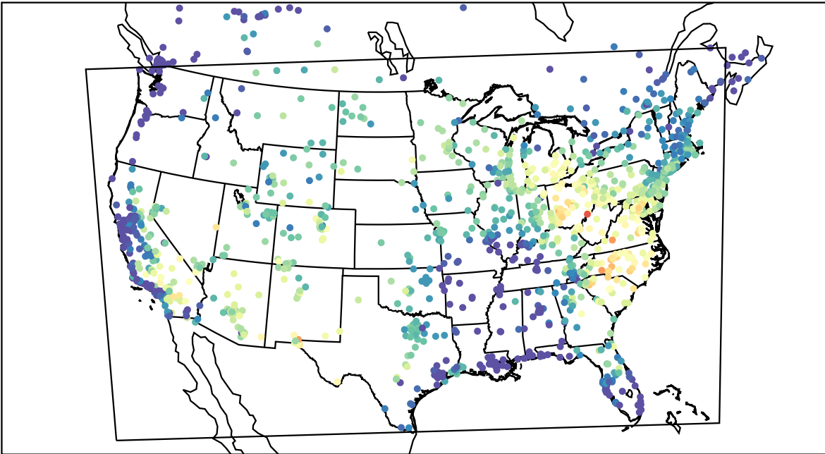
AirNOW (2019-07-15_15:00:00)
