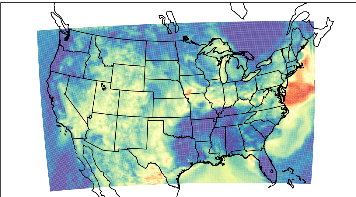
WRF (2019-07-14_07:00:00)
