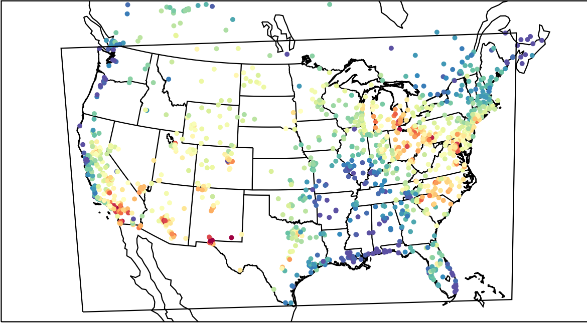
AirNOW (2019-07-15_19:00:00)
