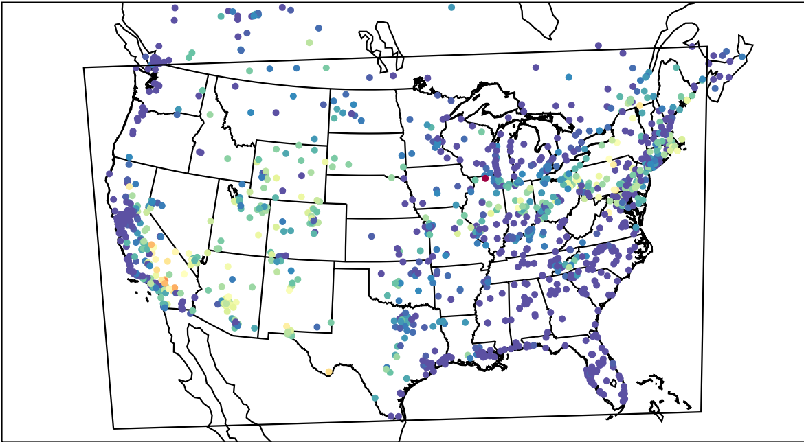
AirNOW (2019-07-14_07:00:00)
