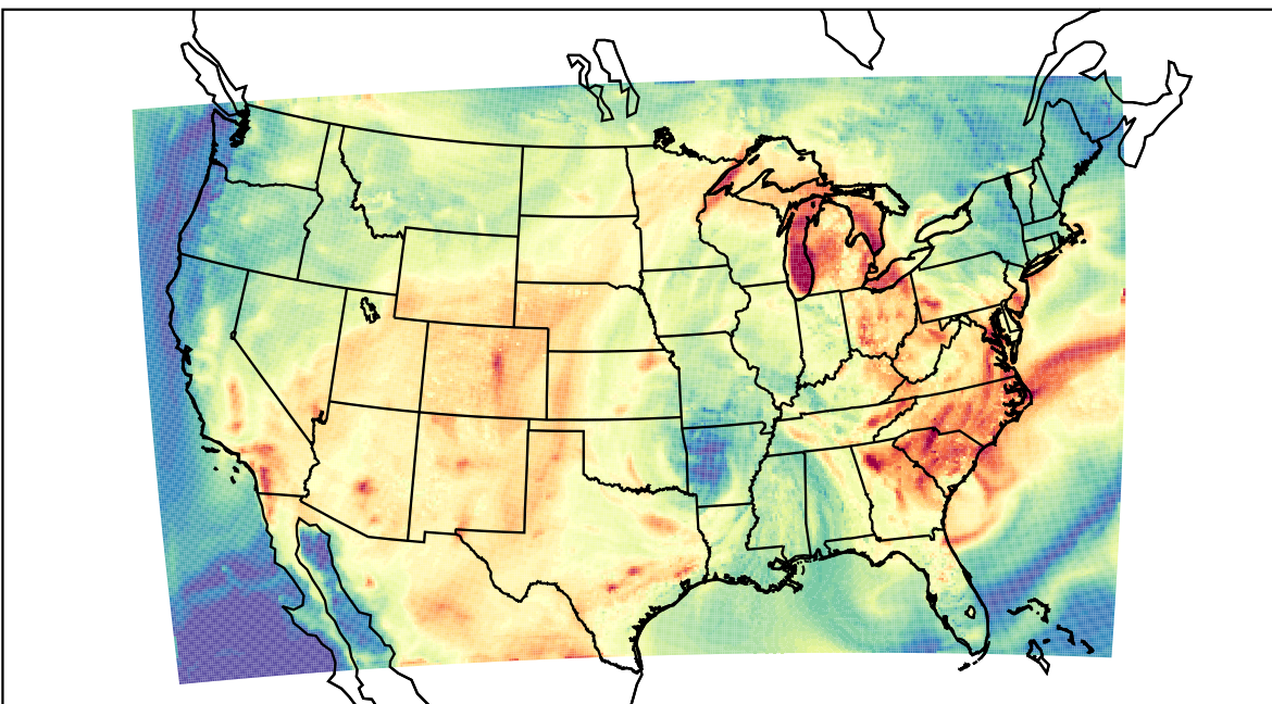
WRF (2019-07-15_21:00:00)
