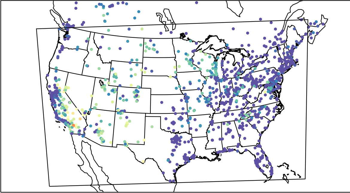
AirNOW (2019-07-15_07:00:00)
