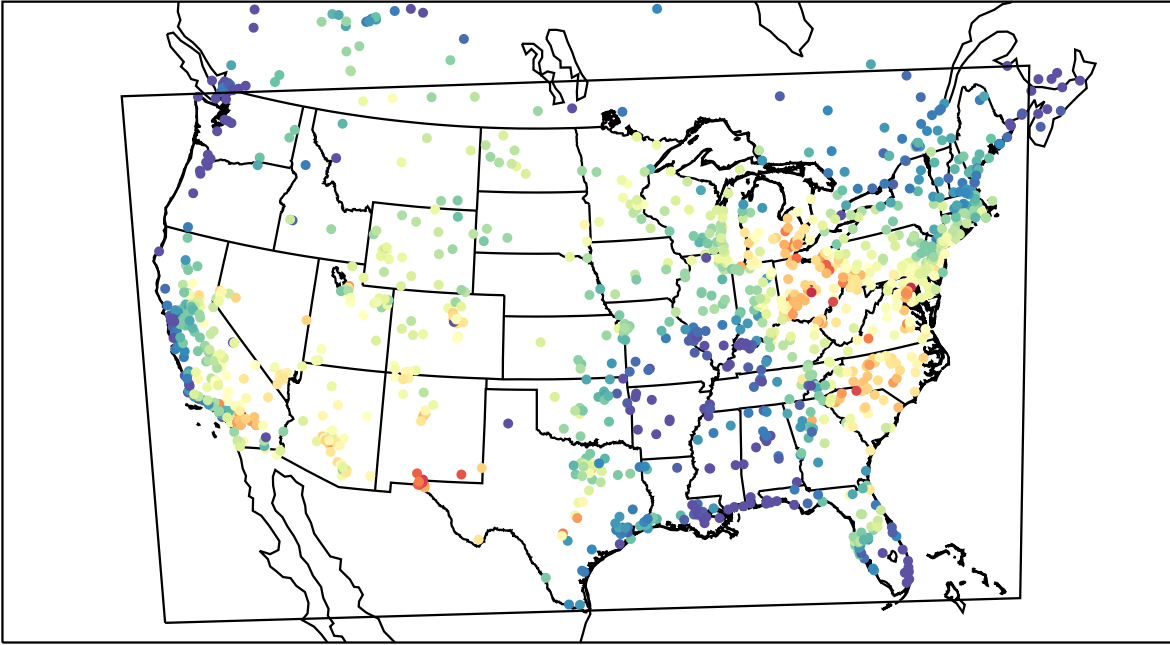
AirNOW (2019-07-15_17:00:00)
