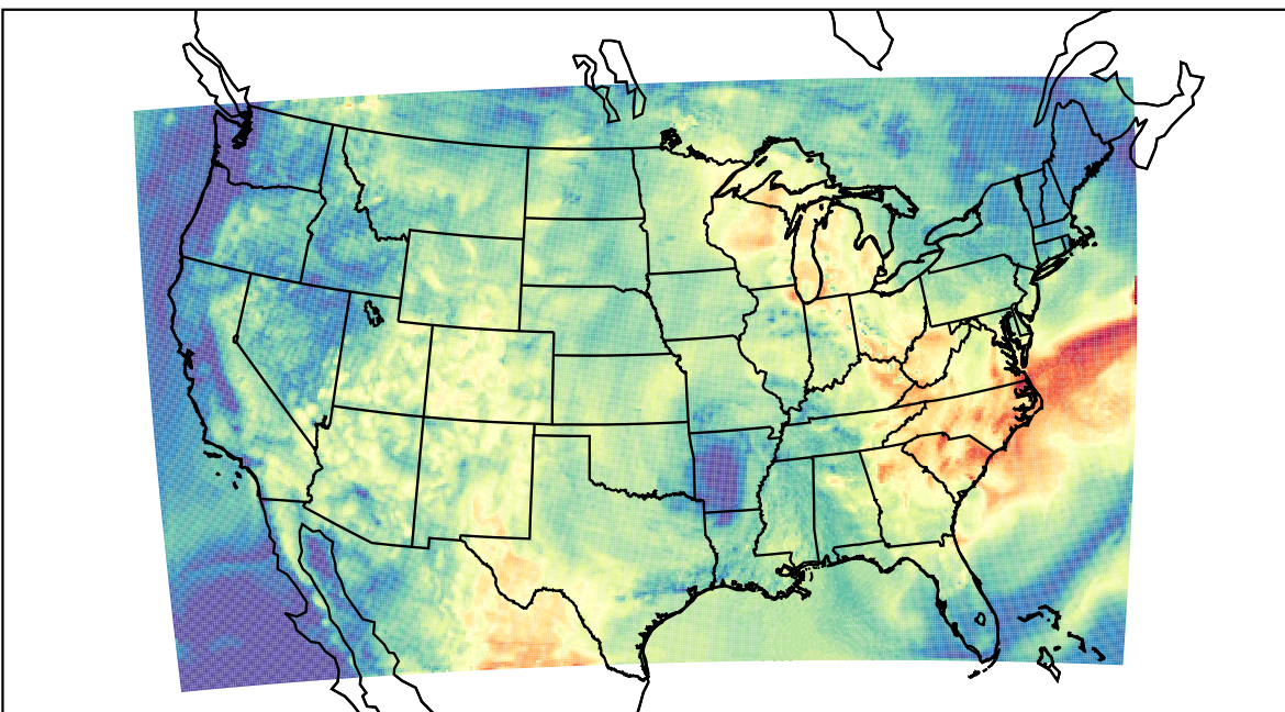
WRF (2019-07-15_15:00:00)
