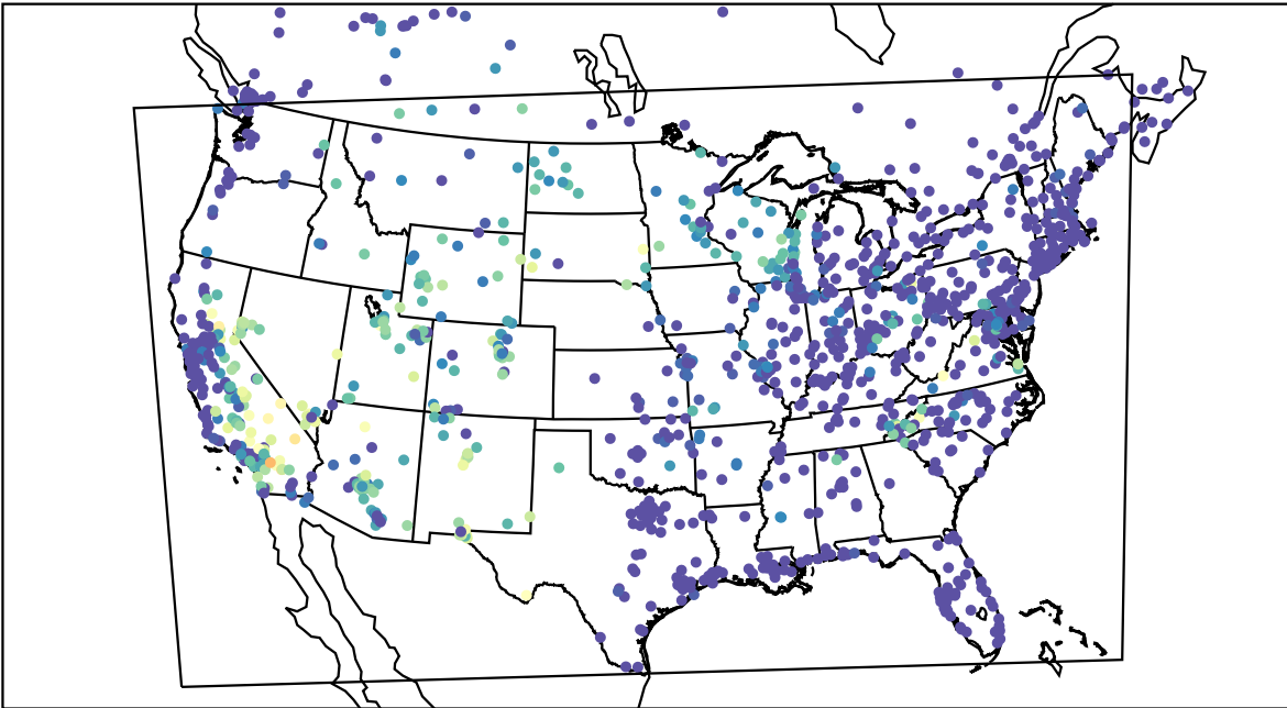
AirNOW (2019-07-15_09:00:00)
