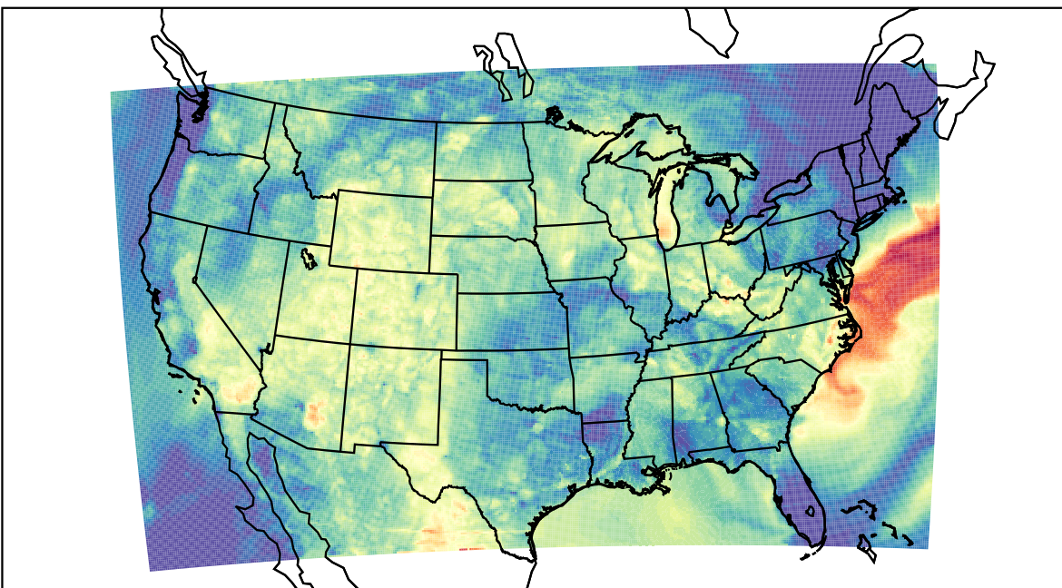
WRF (2019-07-15_05:00:00)
