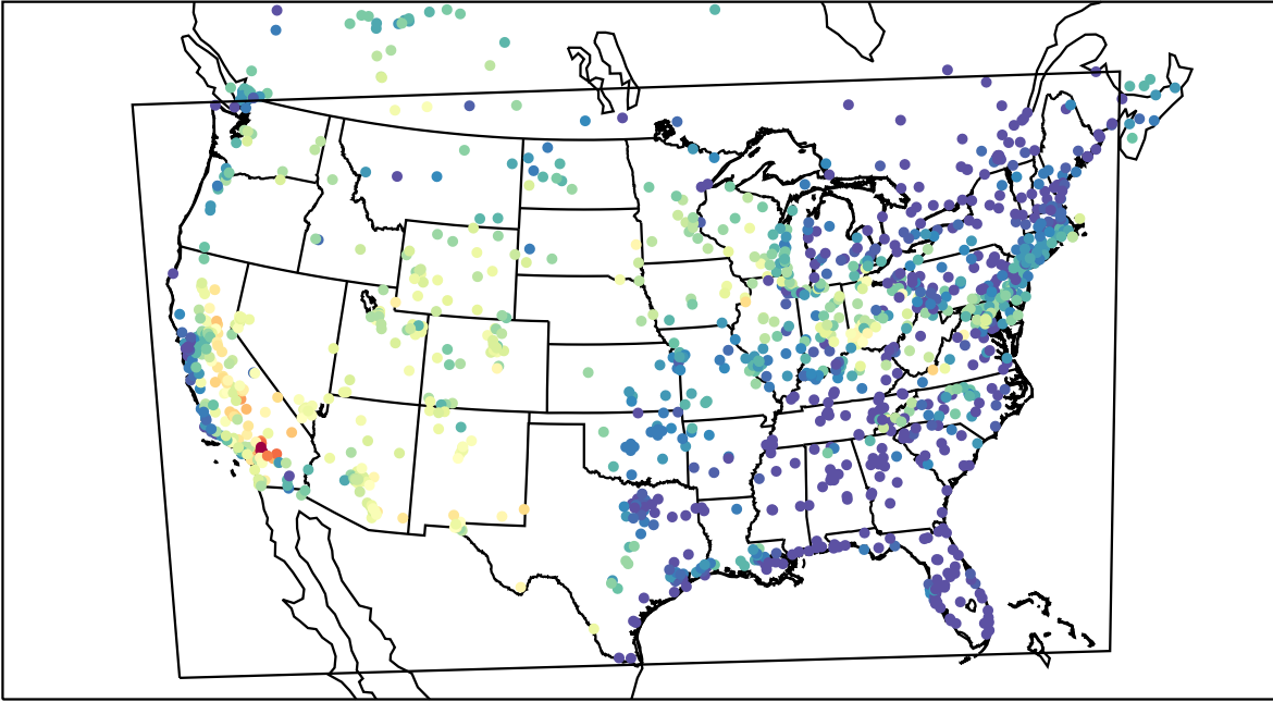
AirNOW (2019-07-15_02:00:00)
