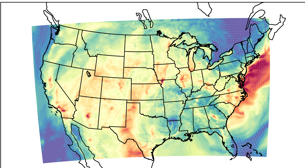
WRF (2019-07-15_00:00:00)
