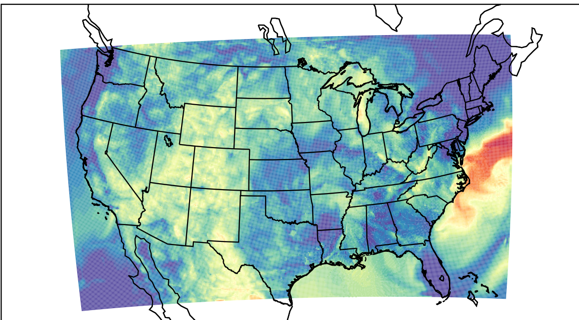
WRF (2019-07-15_09:00:00)
