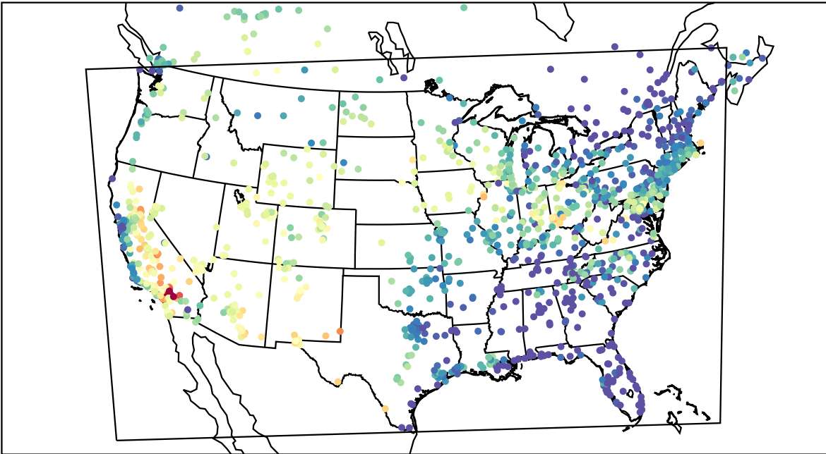
AirNOW (2019-07-15_01:00:00)
