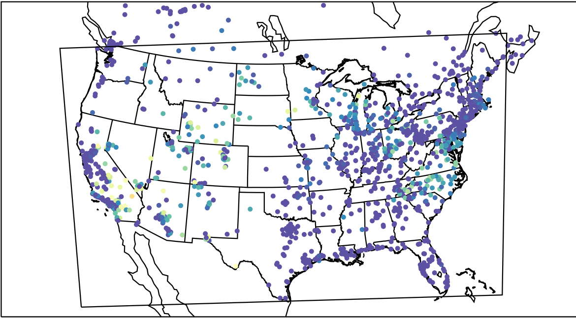
AirNOW (2019-07-15_12:00:00)
