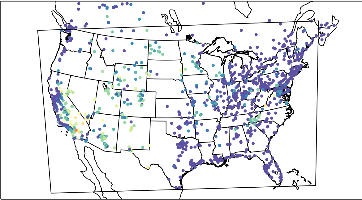
AirNOW (2019-07-15_08:00:00)
