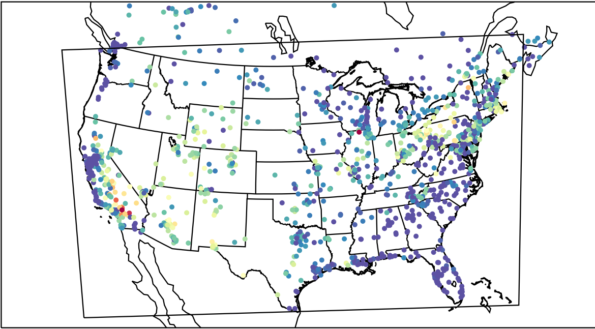
AirNOW (2019-07-14_05:00:00)
