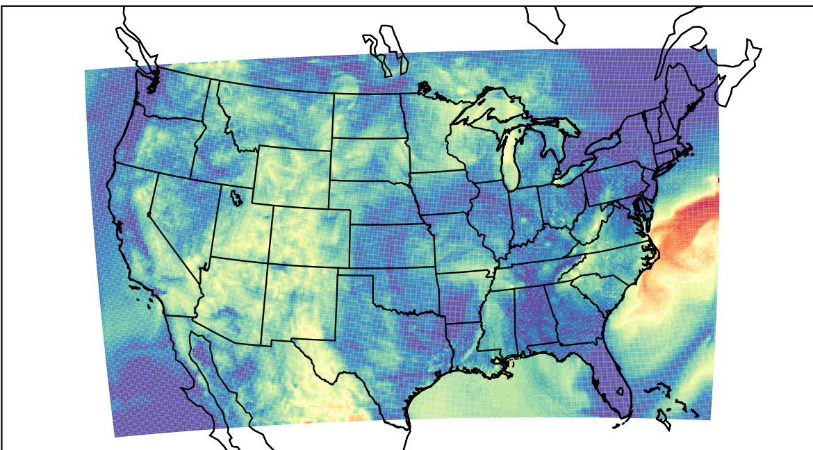
WRF (2019-07-15_12:00:00)
