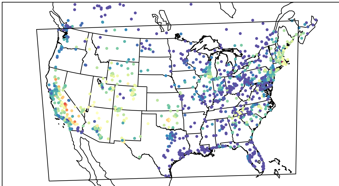
AirNOW (2019-08-08_05:00:00)
