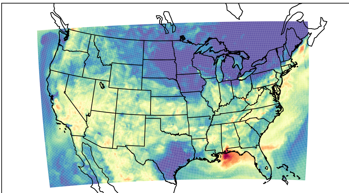
WRF (2019-08-14_07:00:00)
