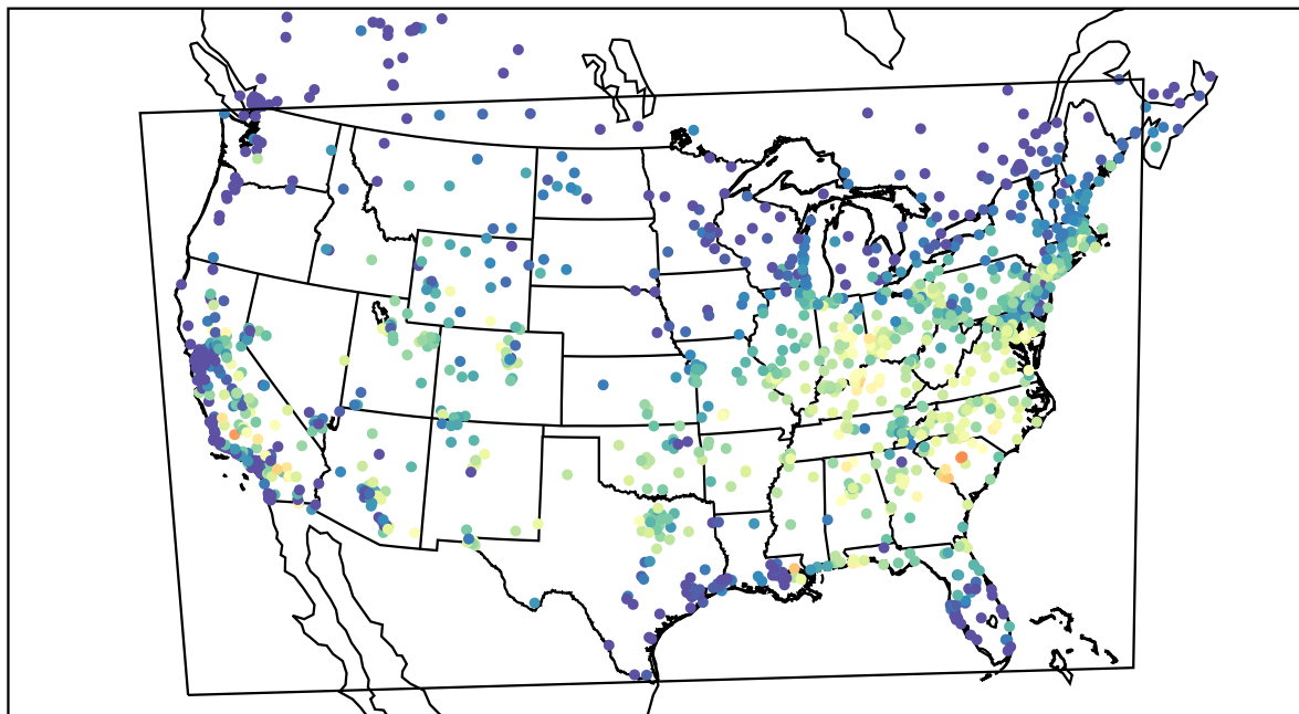
AirNOW (2019-08-14_15:00:00)
