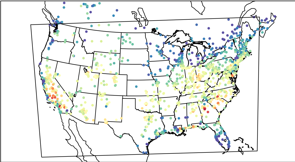
AirNOW (2019-08-14_17:00:00)
