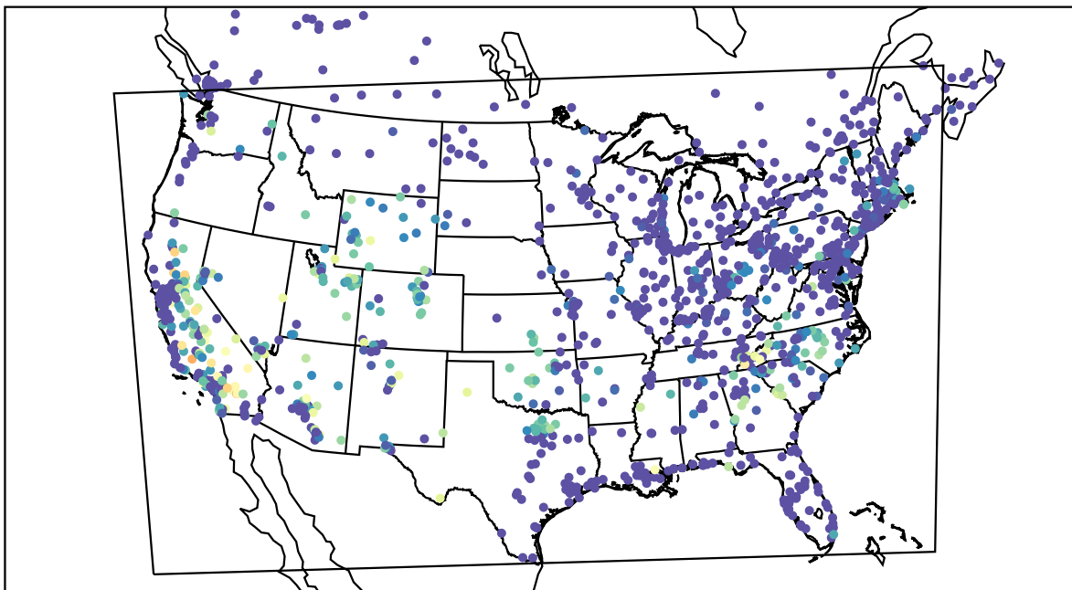
AirNOW (2019-08-14_09:00:00)
