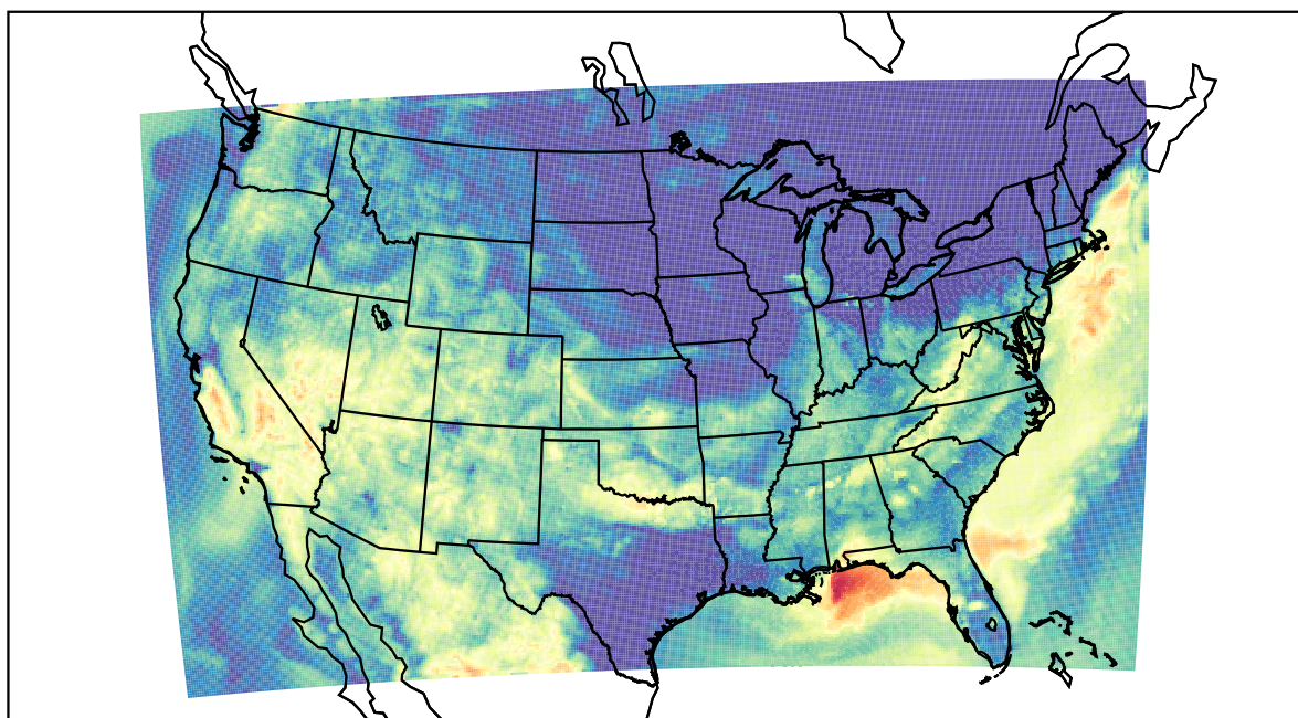
WRF (2019-08-14_12:00:00)
