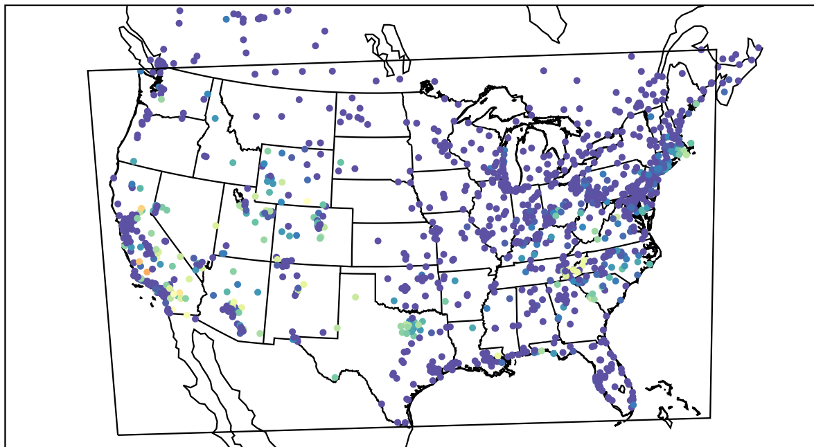
AirNOW (2019-08-14_12:00:00)
