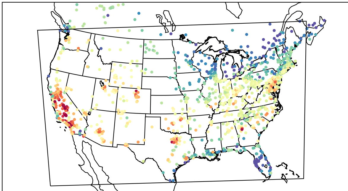
AirNOW (2019-08-14_21:00:00)
