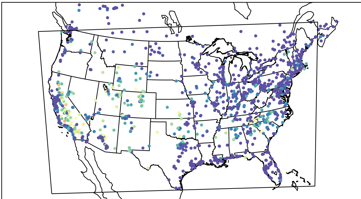
AirNOW (2019-08-14_07:00:00)
