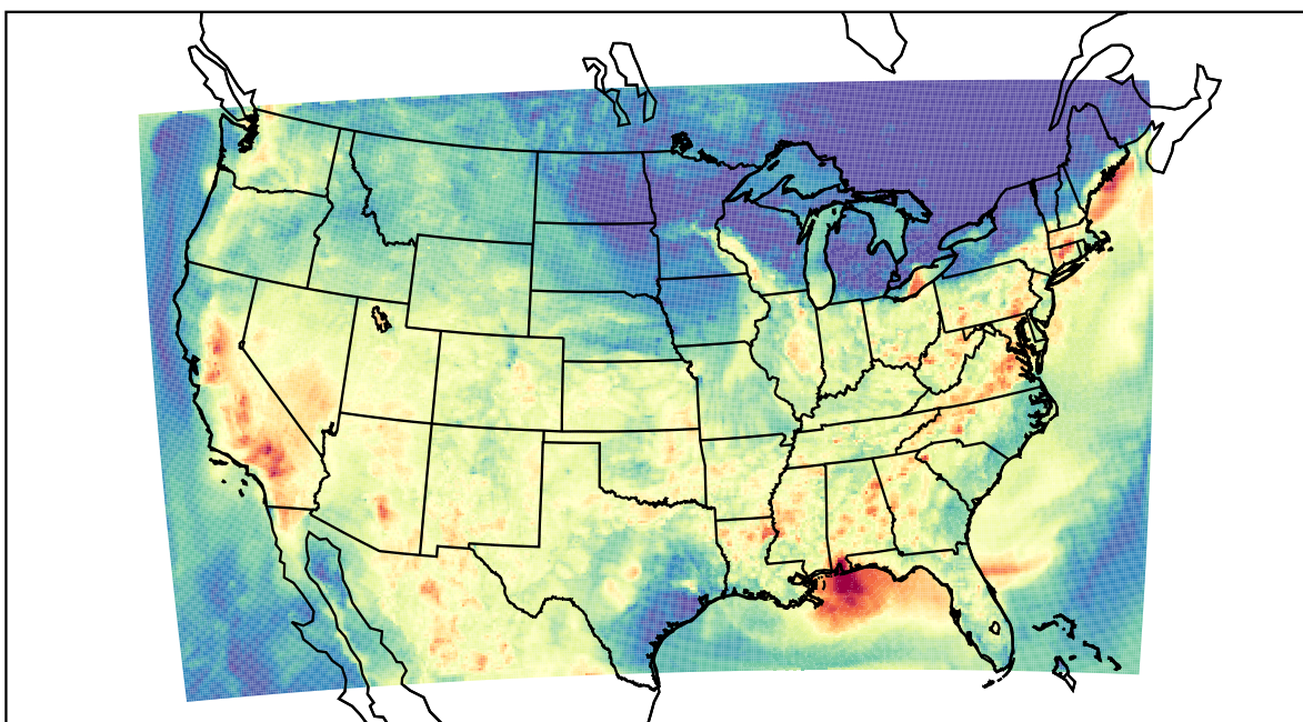
WRF (2019-08-14_02:00:00)
