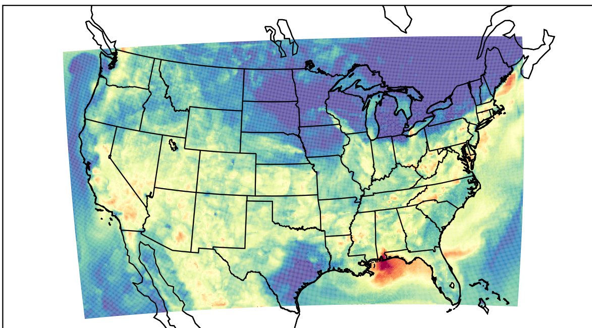
WRF (2019-08-14_05:00:00)
