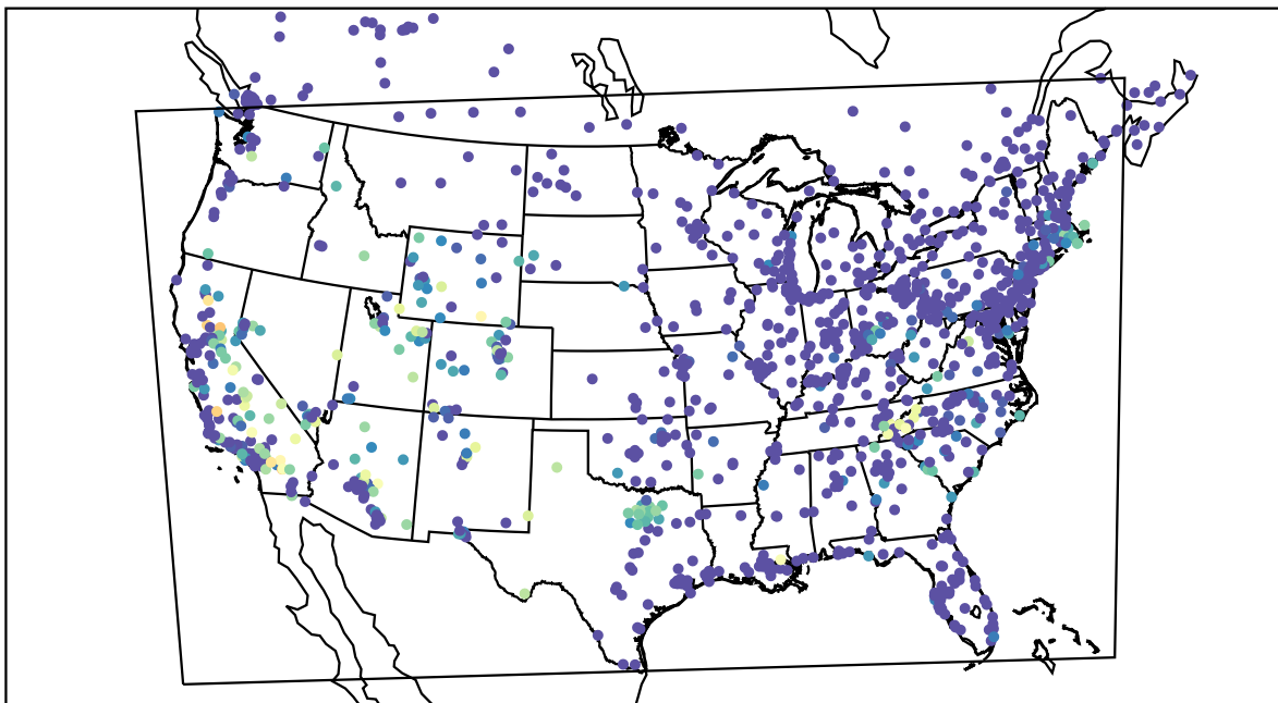
AirNOW (2019-08-14_11:00:00)
