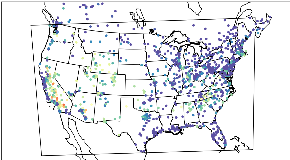
AirNOW (2019-08-14_05:00:00)
