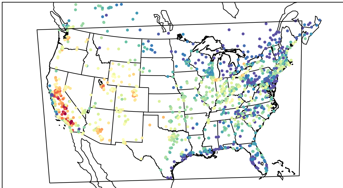
AirNOW (2019-08-14_00:00:00)
