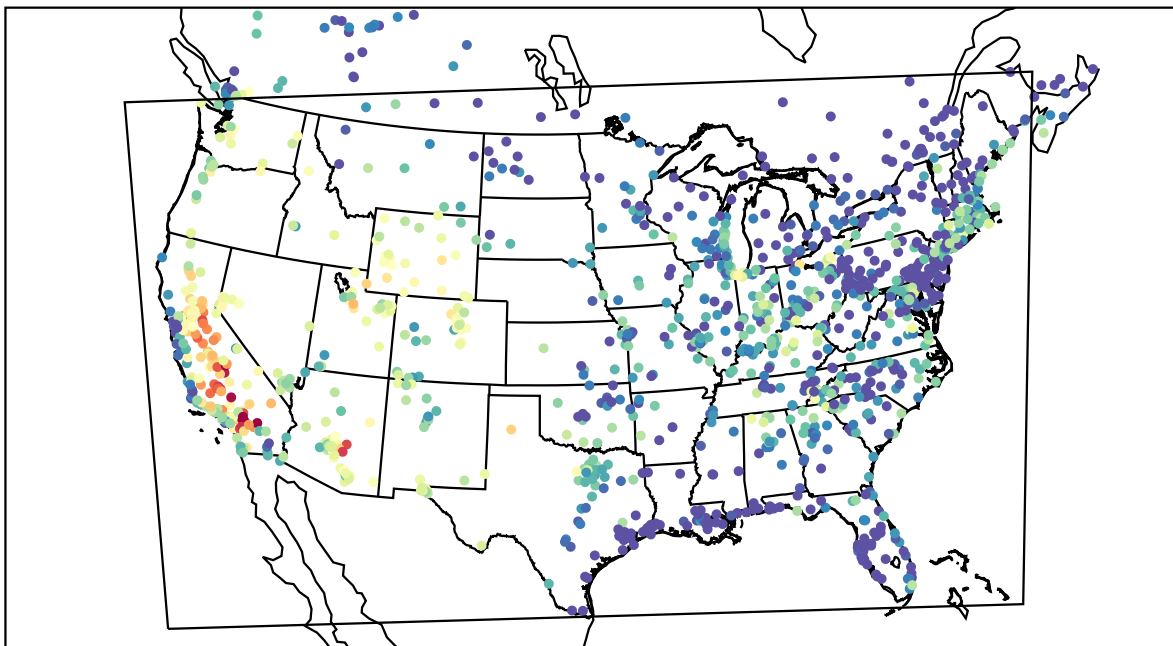
AirNOW (2019-08-14_02:00:00)
