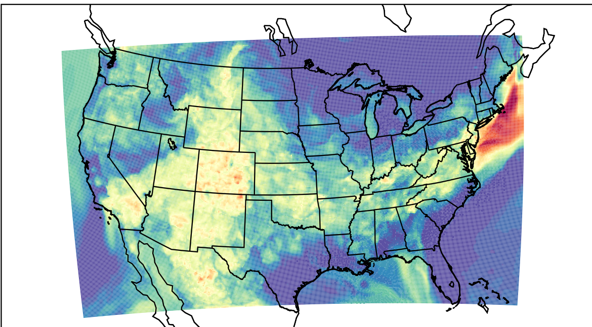
WRF (2019-08-23_05:00:00)
