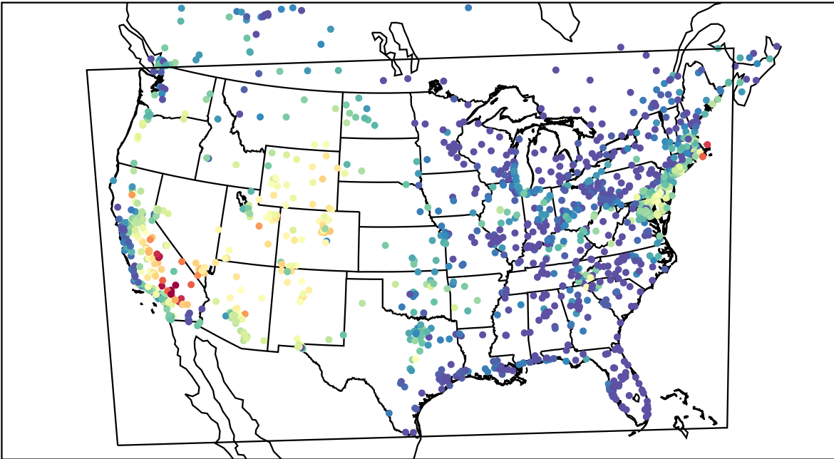
AirNOW (2019-08-23_02:00:00)
