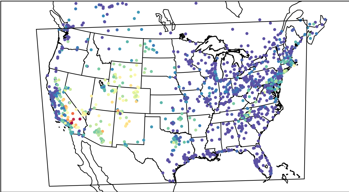
AirNOW (2019-08-23_05:00:00)
