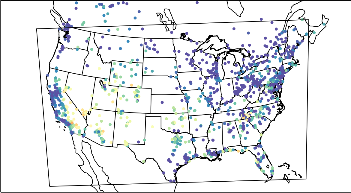
AirNOW (2019-09-08_05:00:00)
