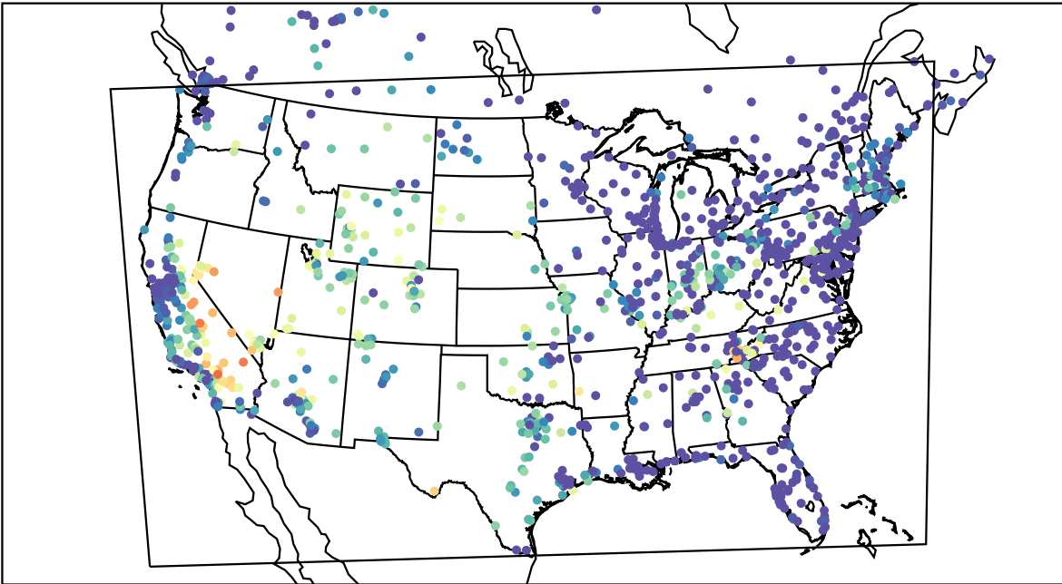
AirNOW (2019-09-16_05:00:00)
