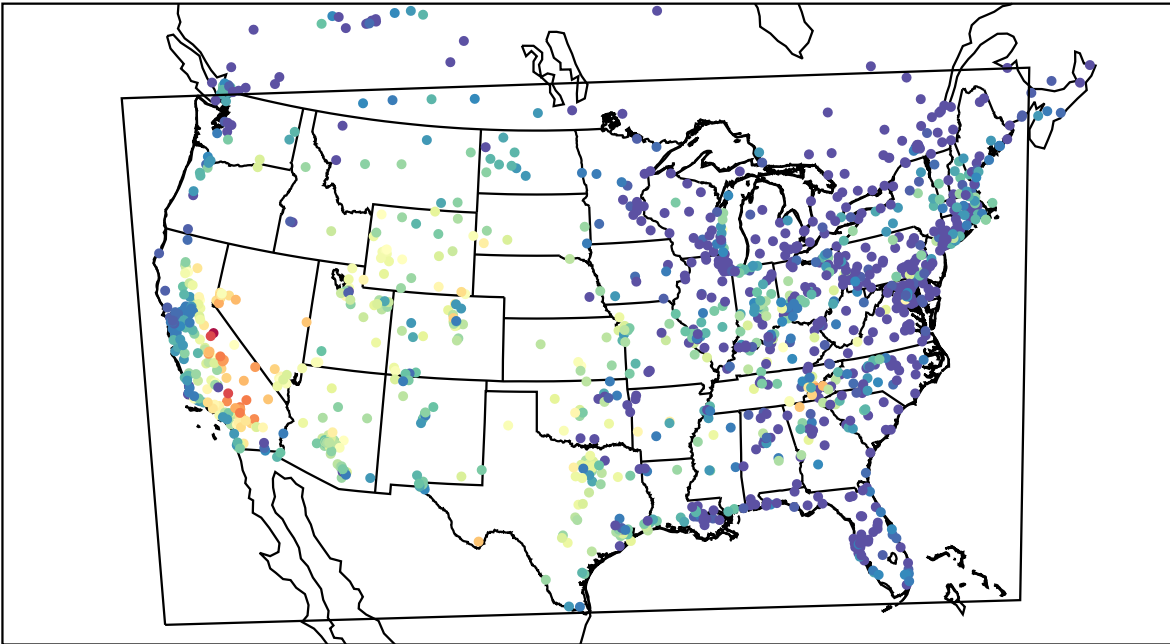
AirNOW (2019-09-16_02:00:00)
