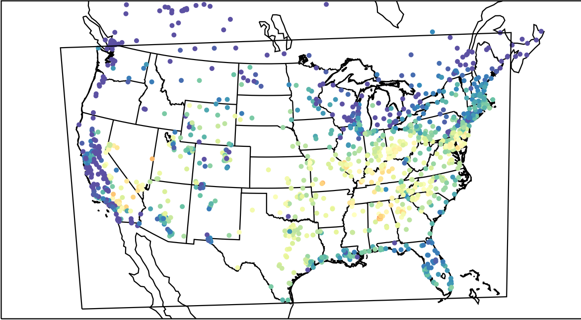
AirNOW (2019-09-16_15:00:00)
