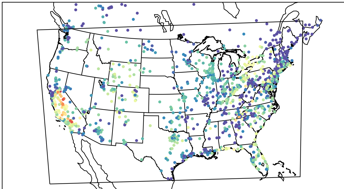
AirNOW (2019-09-26_02:00:00)
