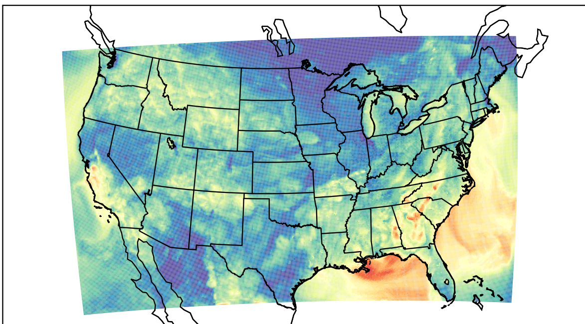
WRF (2019-09-26_05:00:00)
