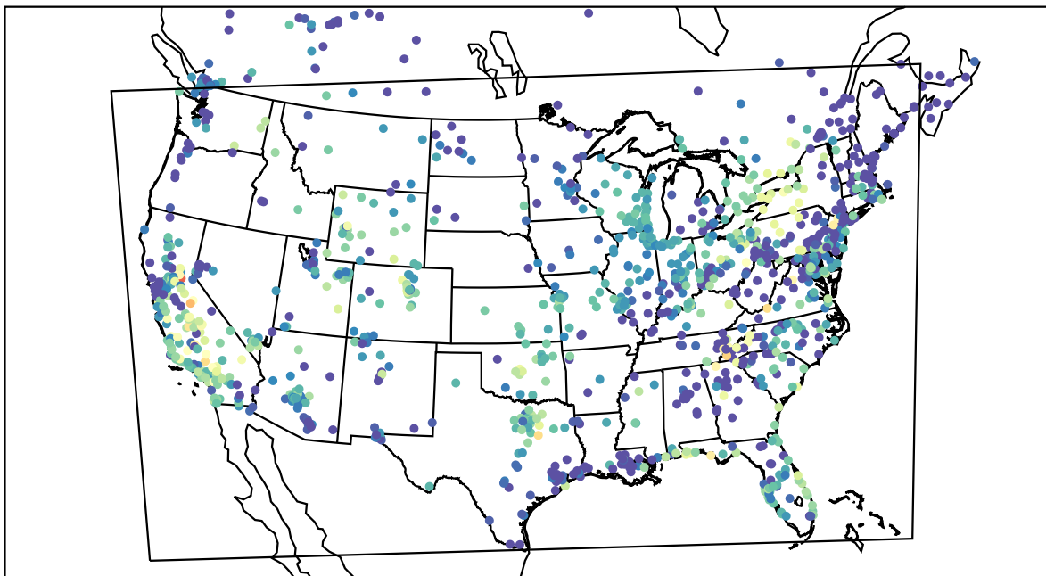
AirNOW (2019-09-26_05:00:00)
