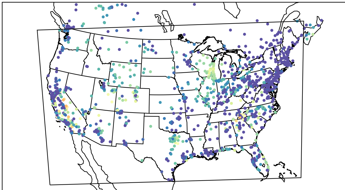
AirNOW (2019-09-25_05:00:00)
