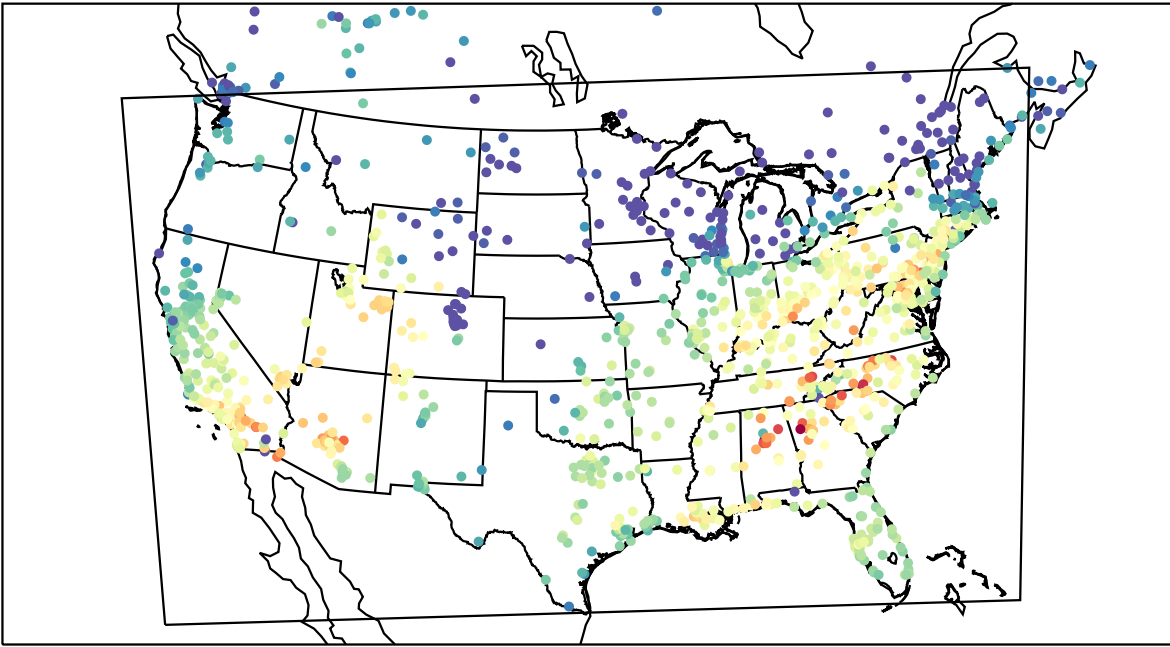
AirNOW (2019-10-01_21:00:00)
