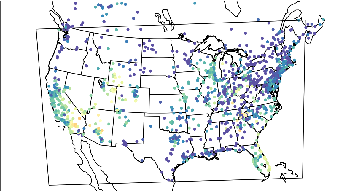
AirNOW (2019-10-01_02:00:00)
