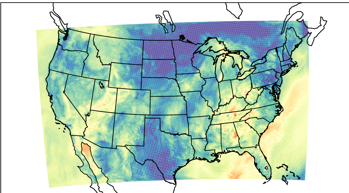
WRF (2019-10-01_05:00:00)
