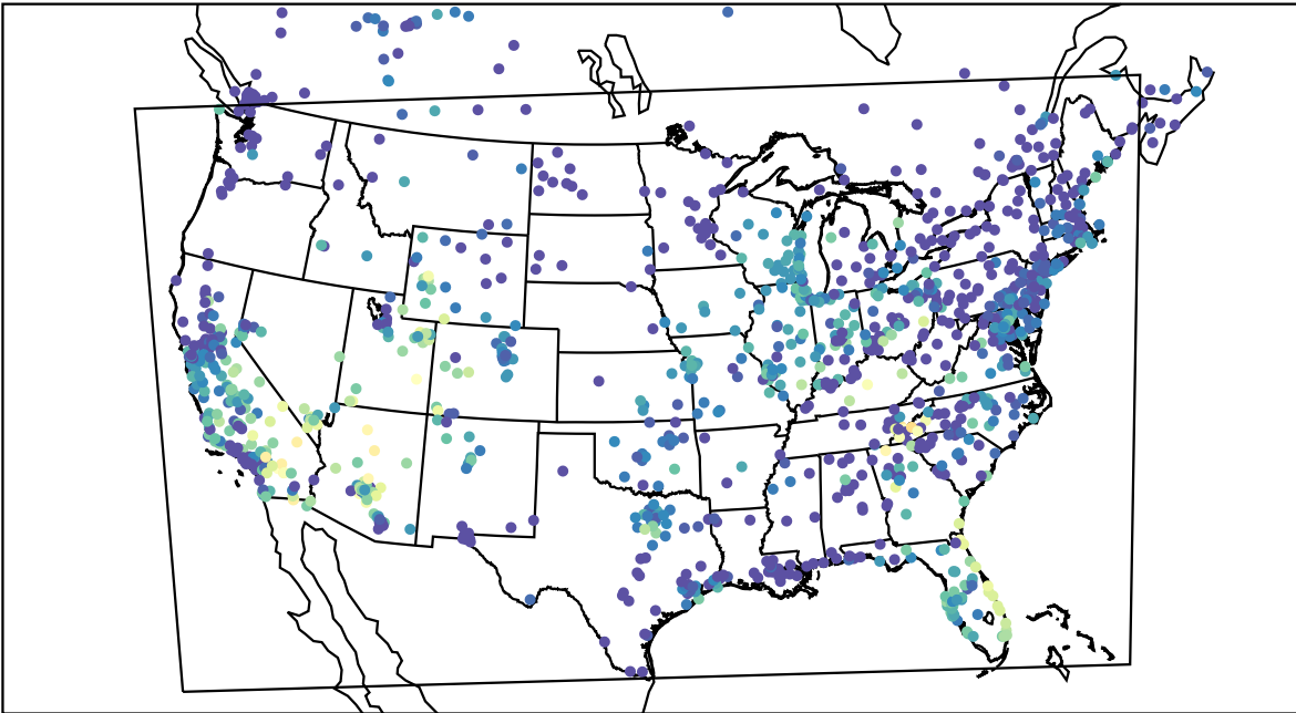
AirNOW (2019-10-01_05:00:00)
