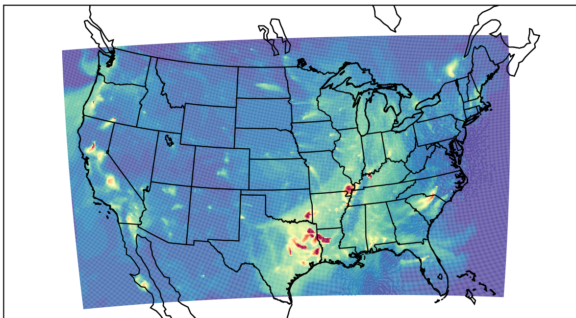
WRF 2019-10-06_05:00:00
