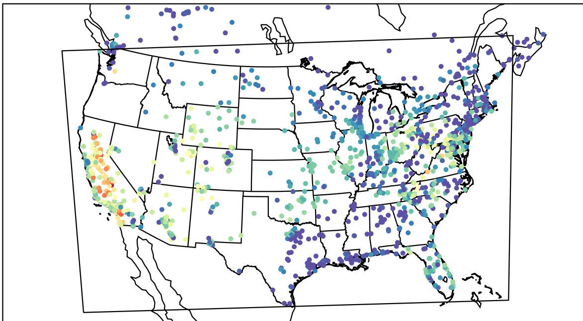
AirNOW (2019-10-16_01:00:00)
