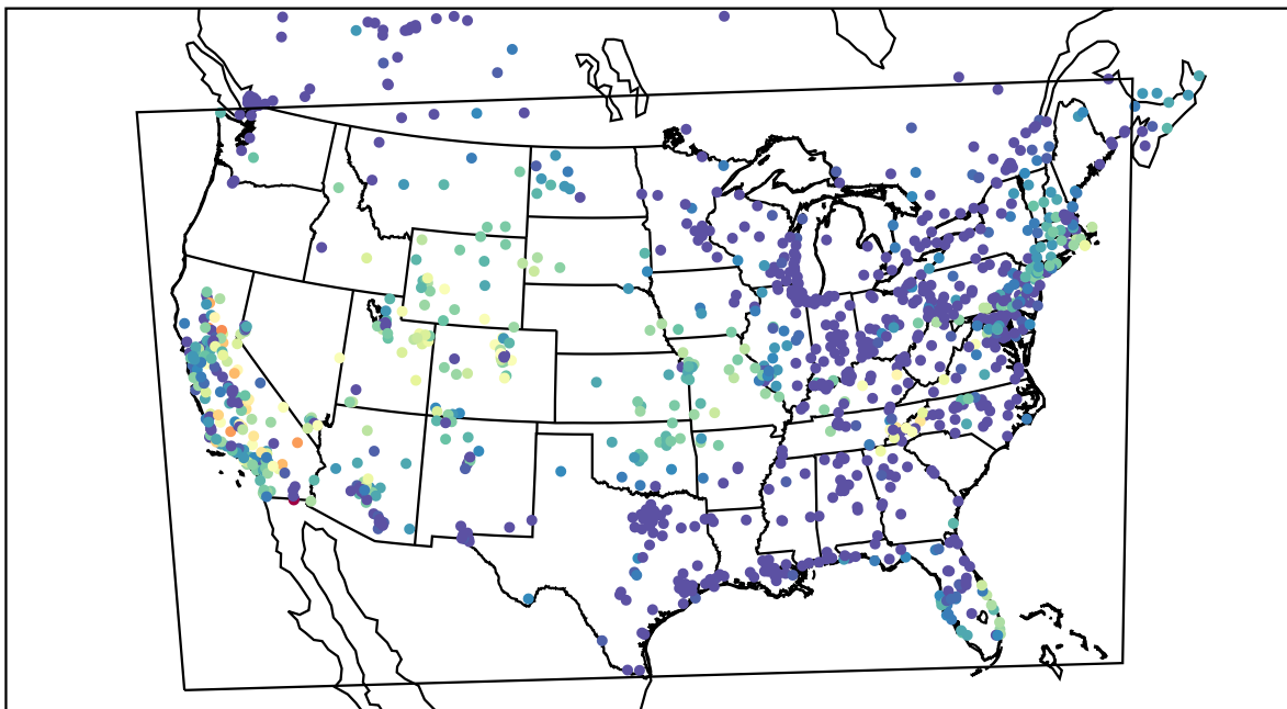
AirNOW (2019-10-15_04:00:00)
