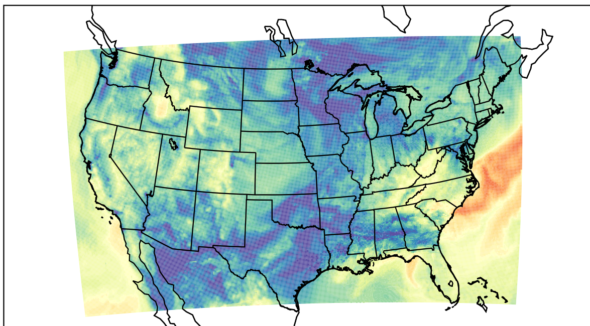
WRF (2019-10-15_15:00:00)
