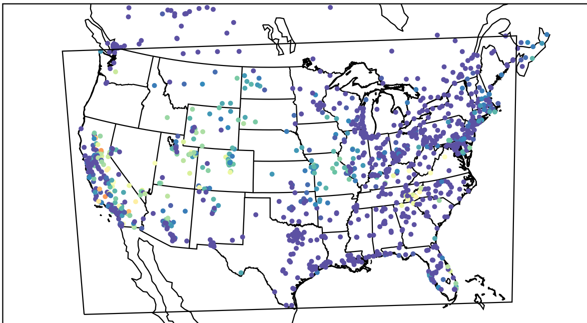
AirNOW (2019-10-15_09:00:00)
