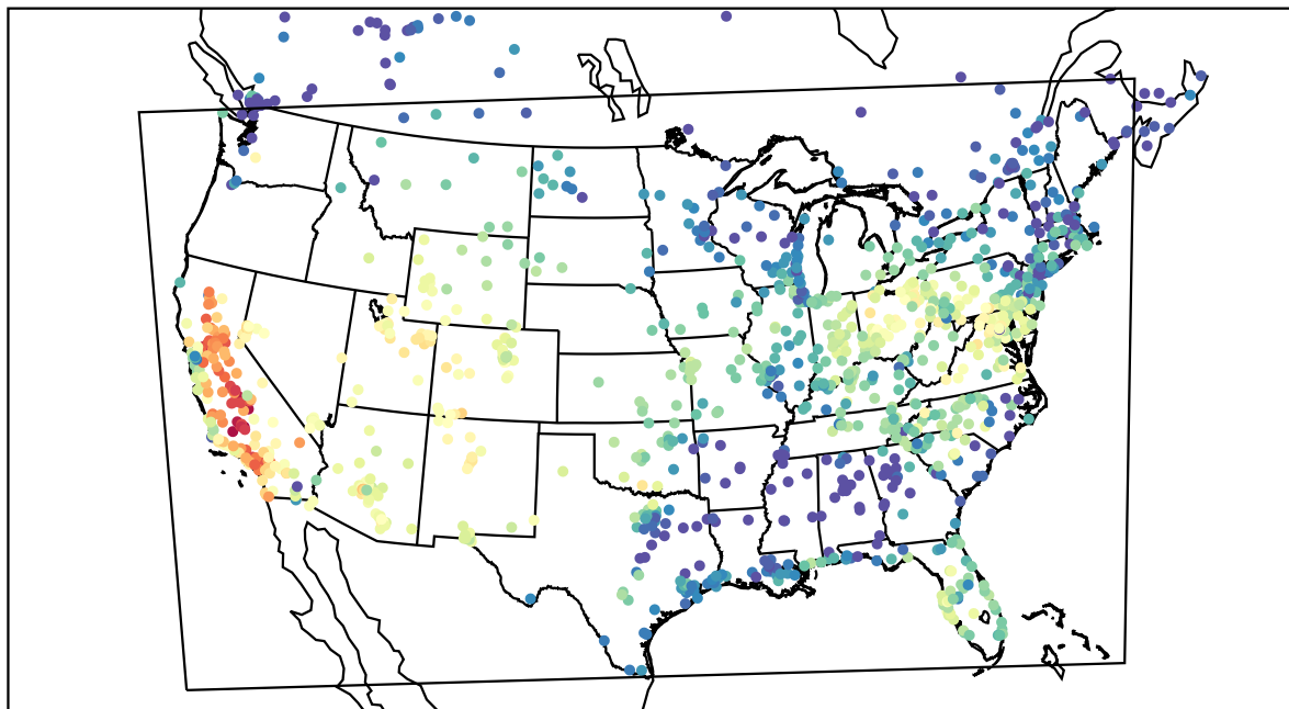
AirNOW (2019-10-15_22:00:00)
