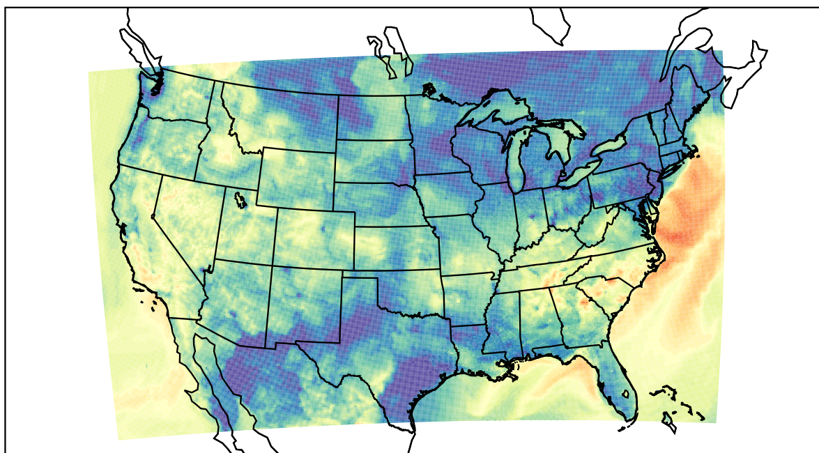
WRF (2019-10-15_05:00:00)
