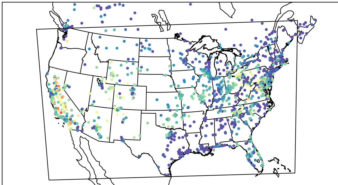
AirNOW (2019-10-16_02:00:00)
