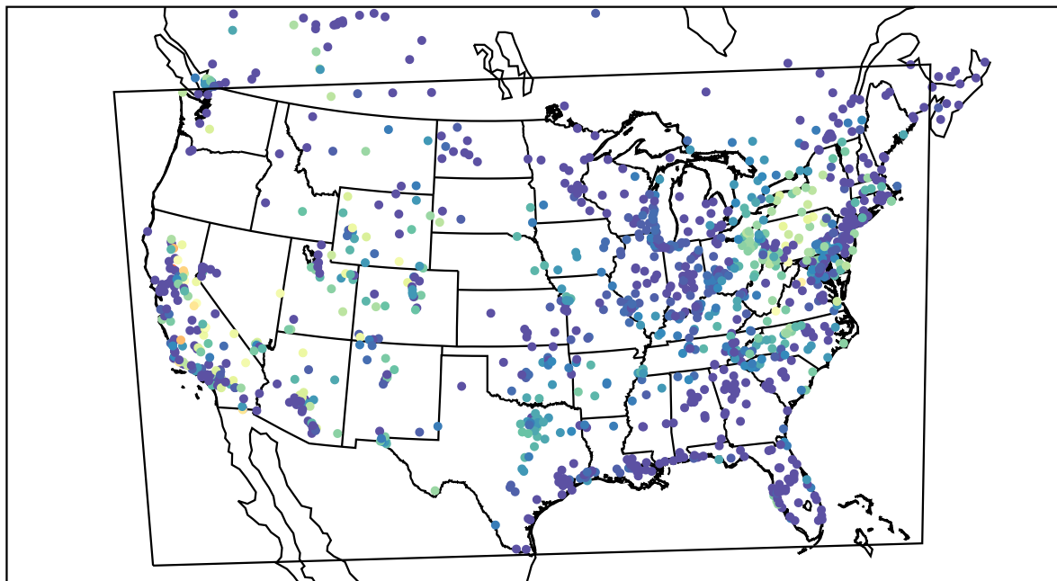
AirNOW (2019-10-16_11:00:00)
