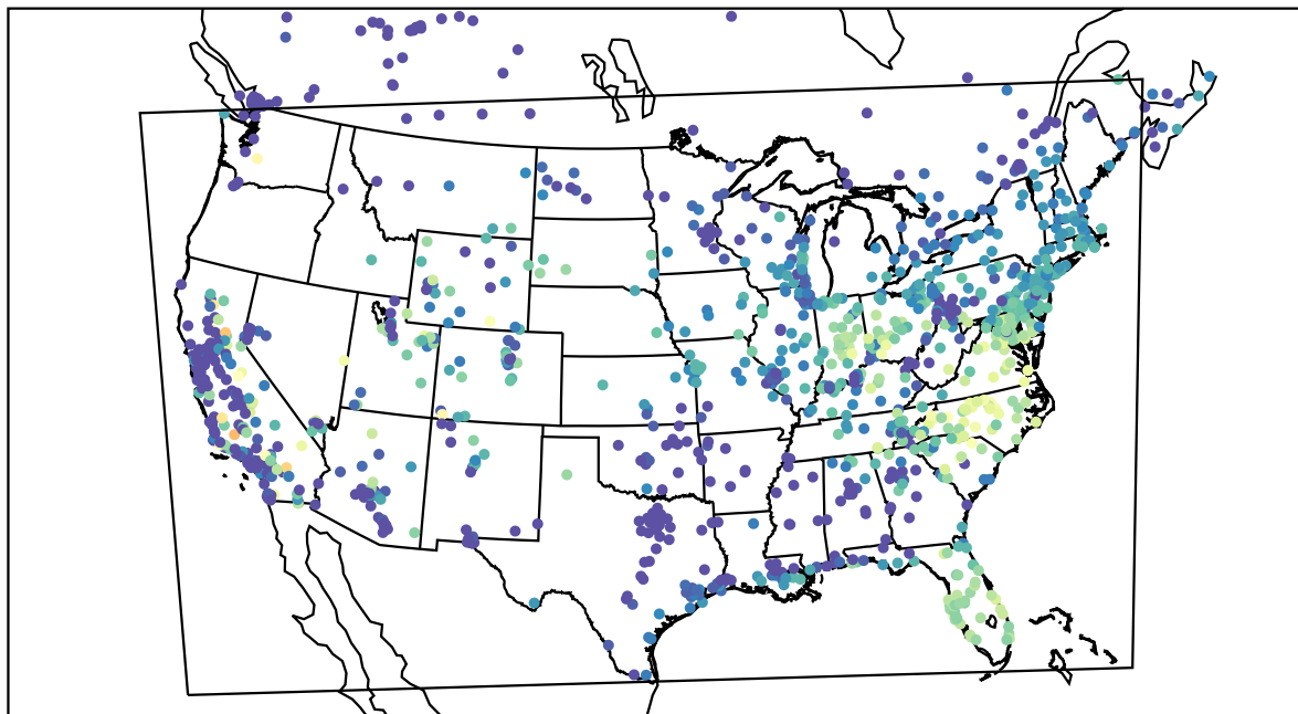
AirNOW (2019-10-15_15:00:00)
