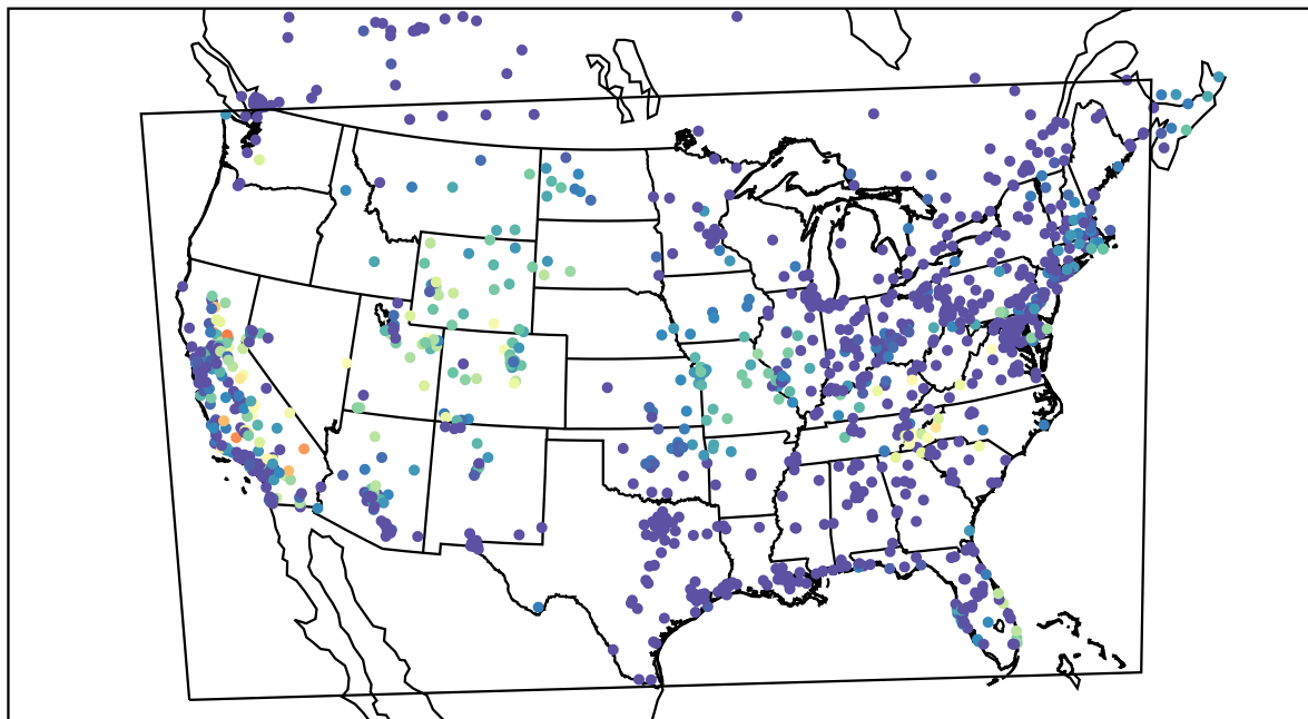
AirNOW (2019-10-15_08:00:00)
