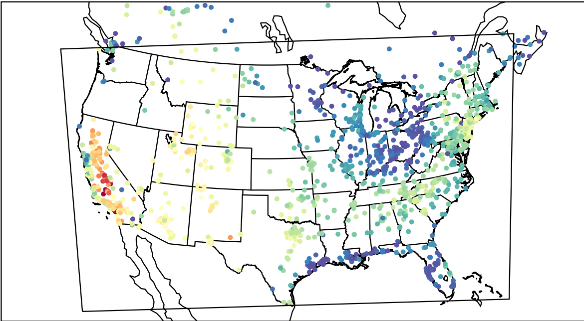
AirNOW (2019-10-16_21:00:00)
