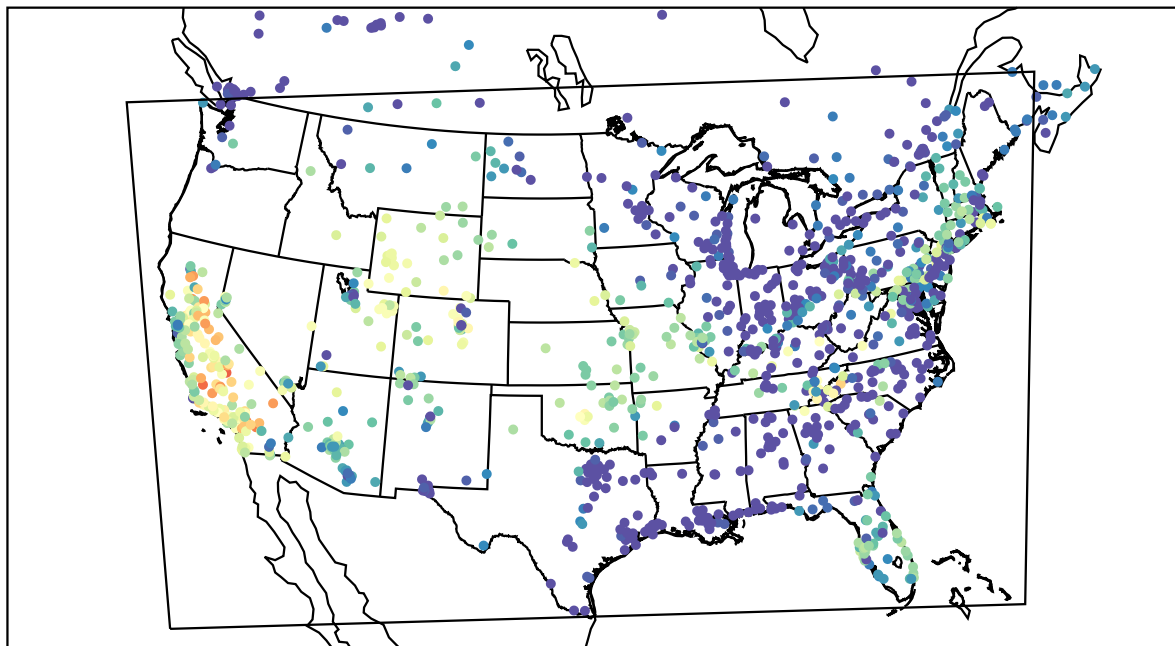
AirNOW (2019-10-15_01:00:00)
