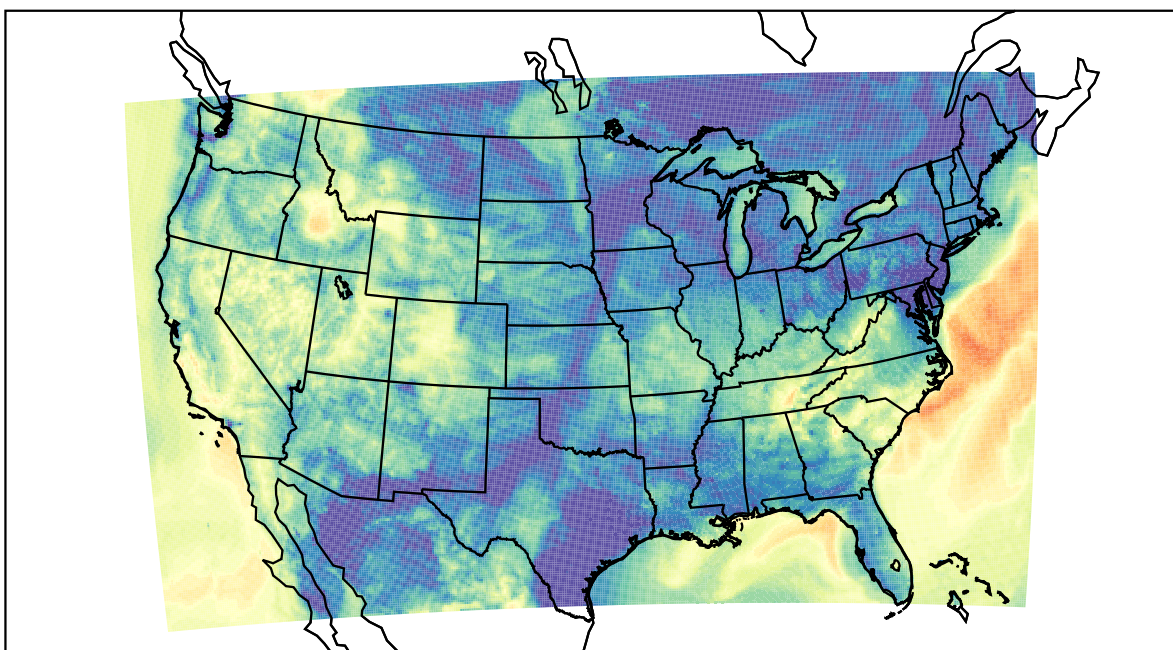
WRF (2019-10-15_09:00:00)
