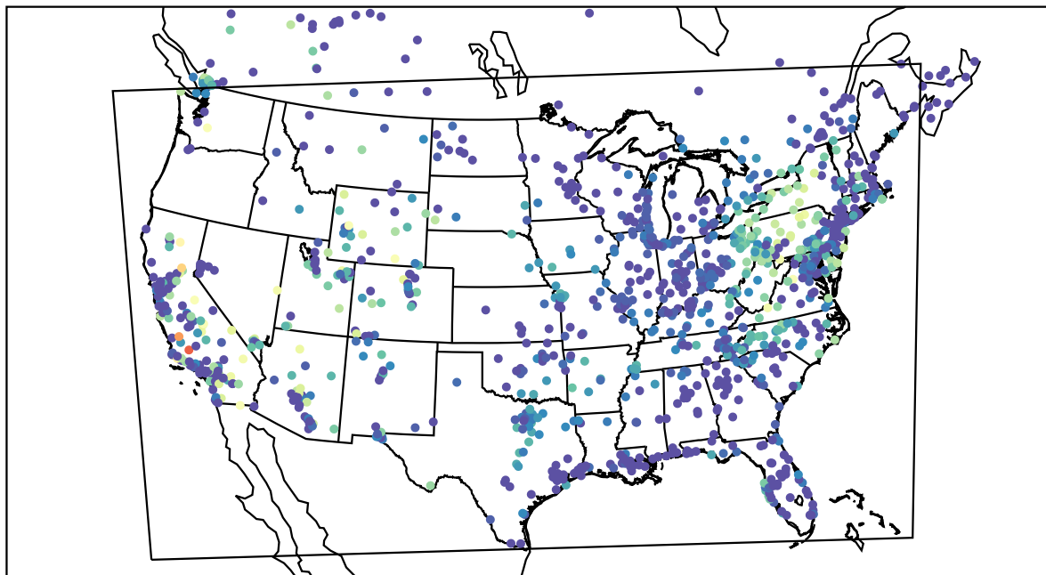
AirNOW (2019-10-16_12:00:00)
