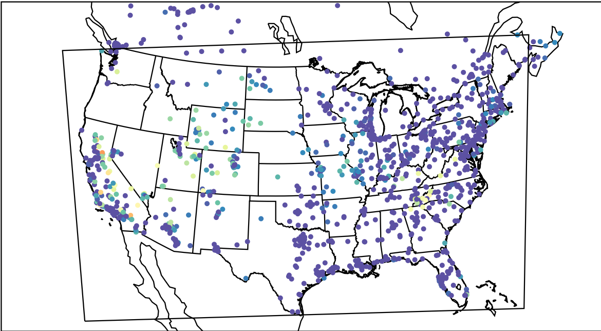
AirNOW (2019-10-15_11:00:00)
