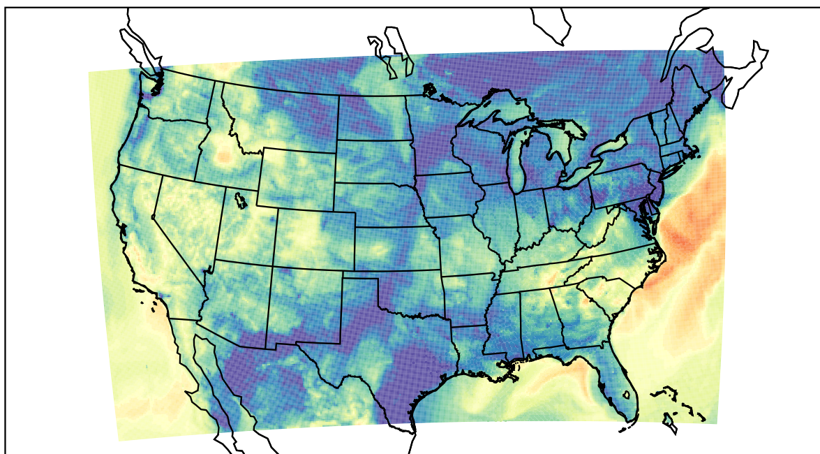
WRF (2019-10-15_08:00:00)
