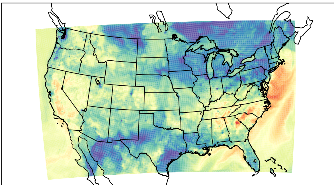
WRF (2019-10-15_02:00:00)
