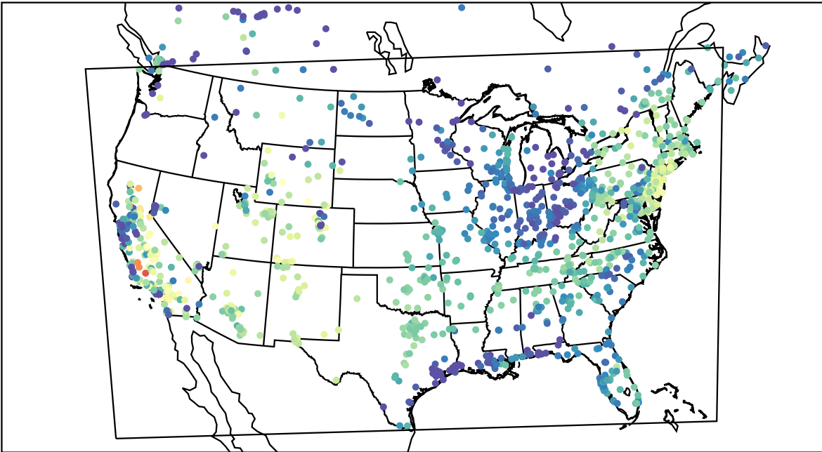
AirNOW (2019-10-16_17:00:00)
