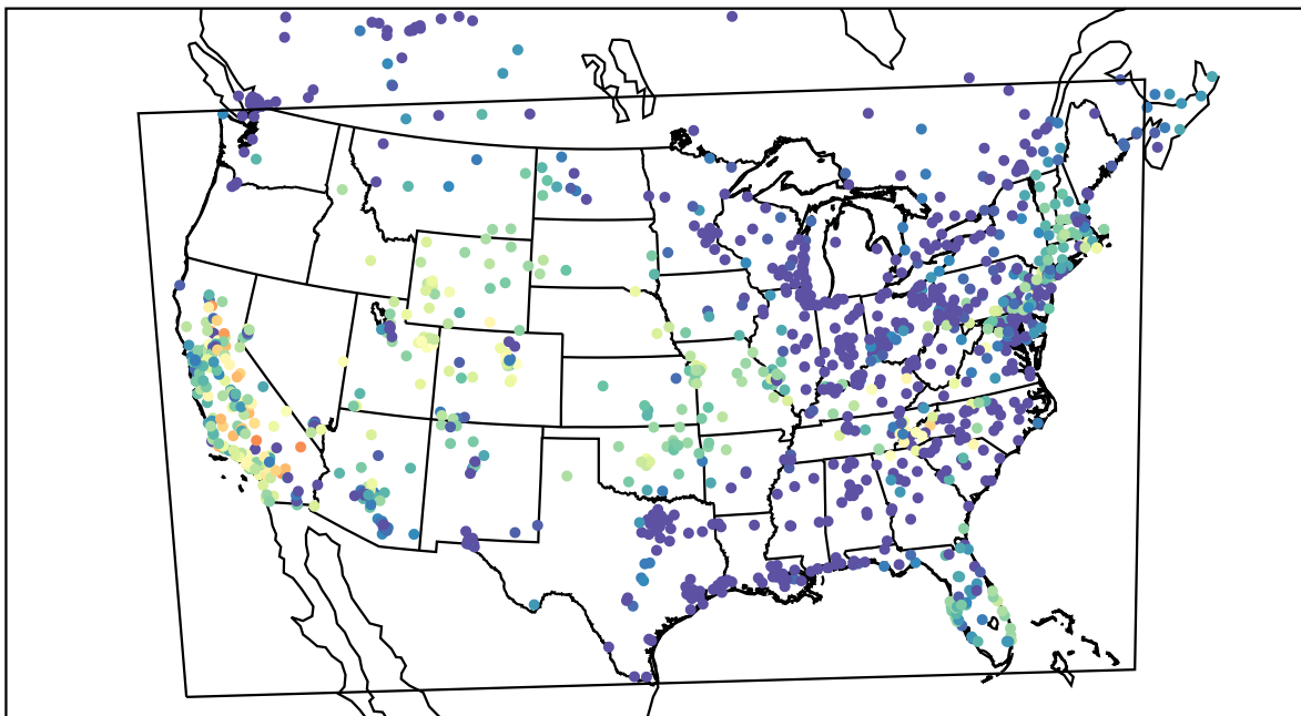
AirNOW (2019-10-15_02:00:00)
