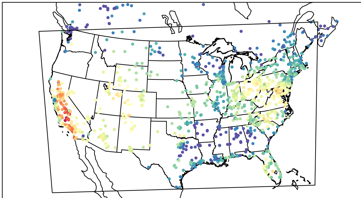
AirNOW (2019-10-15_21:00:00)
