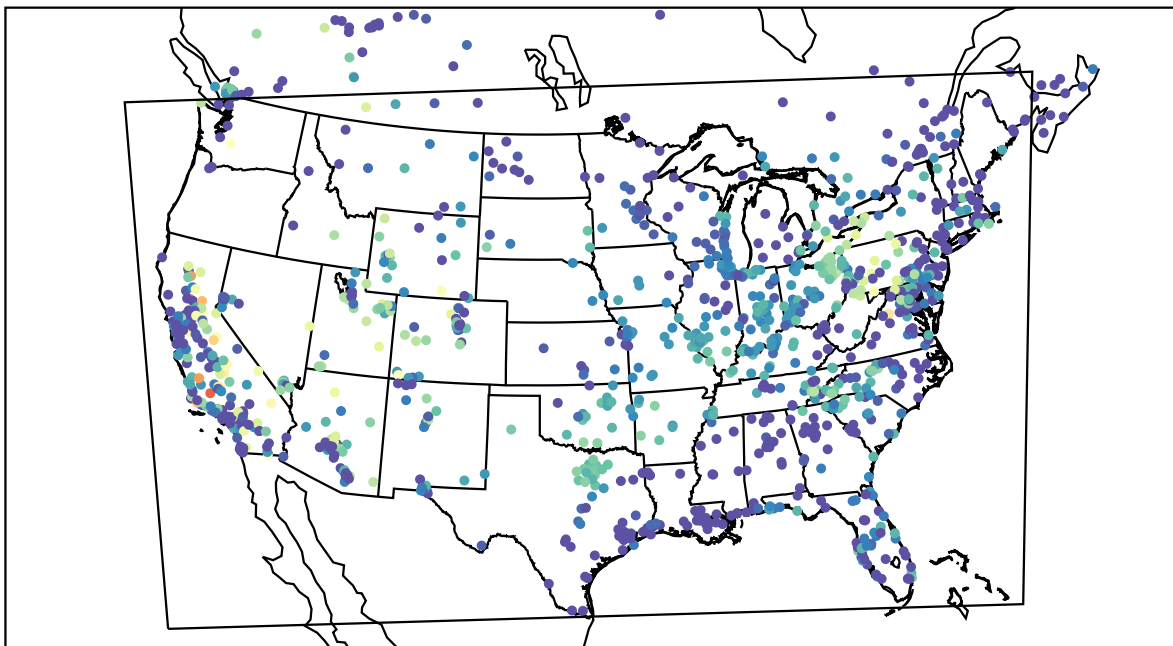
AirNOW (2019-10-16_07:00:00)
