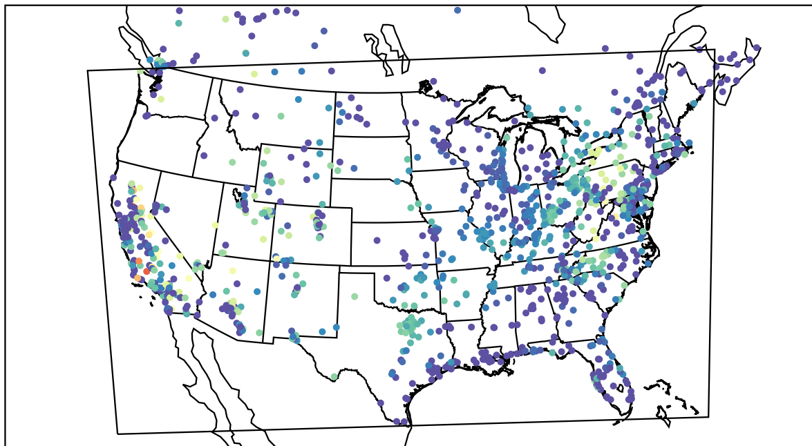
AirNOW (2019-10-16_09:00:00)
