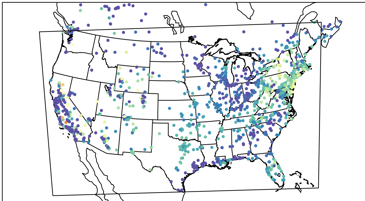
AirNOW (2019-10-16_15:00:00)
