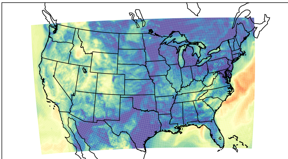
WRF (2019-10-15_12:00:00)
