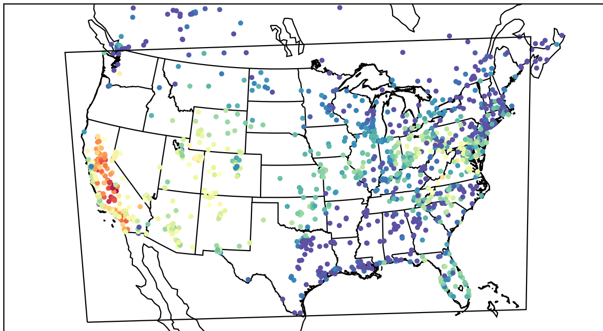
AirNOW (2019-10-16_00:00:00)
