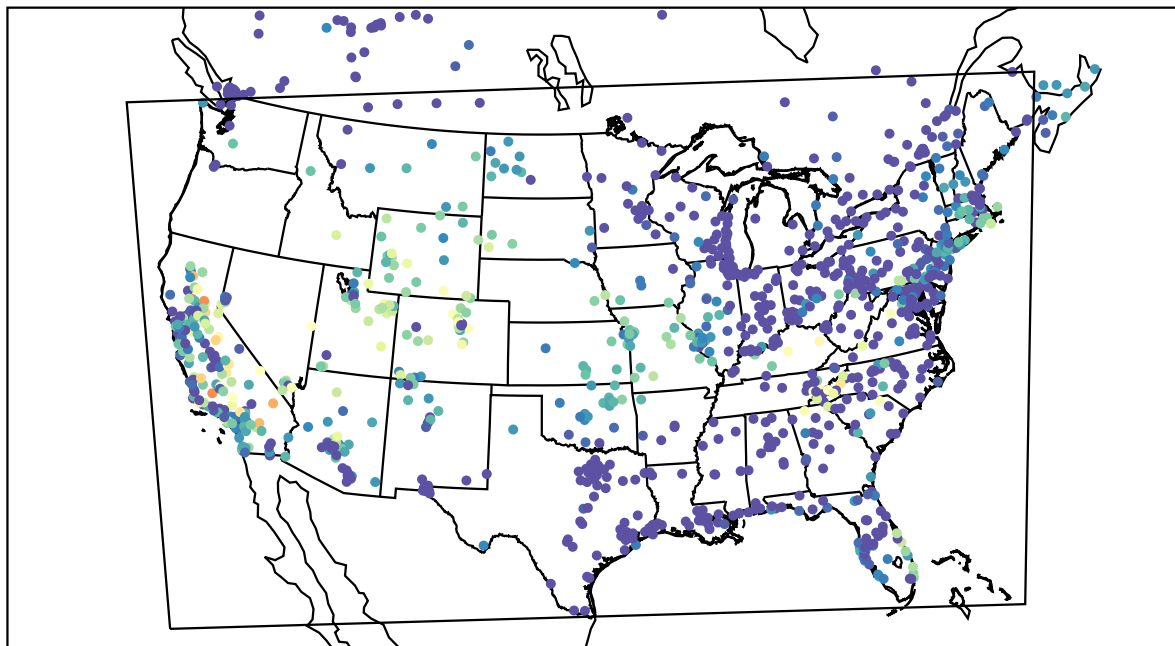
AirNOW (2019-10-15_05:00:00)
