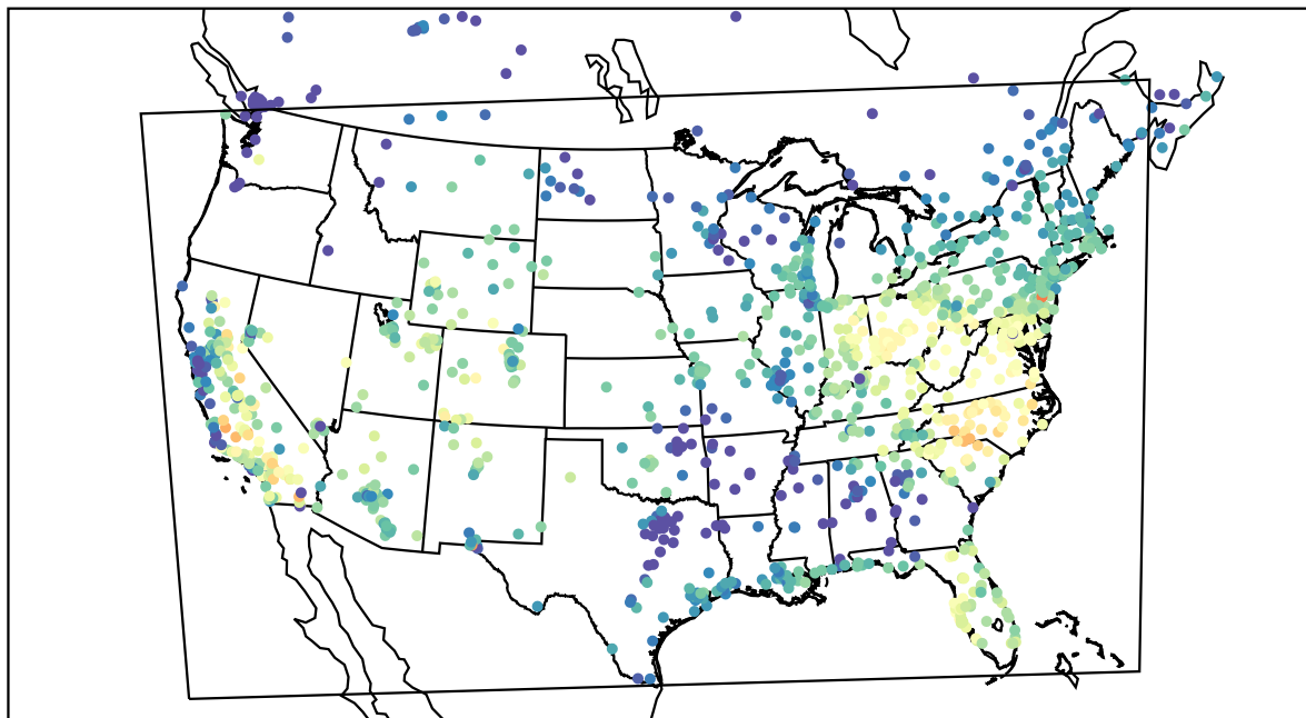
AirNOW (2019-10-15_17:00:00)
