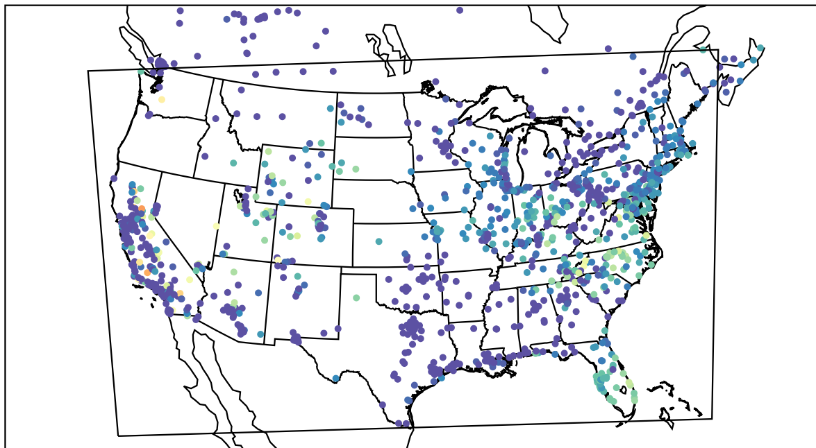
AirNOW (2019-10-15_14:00:00)
