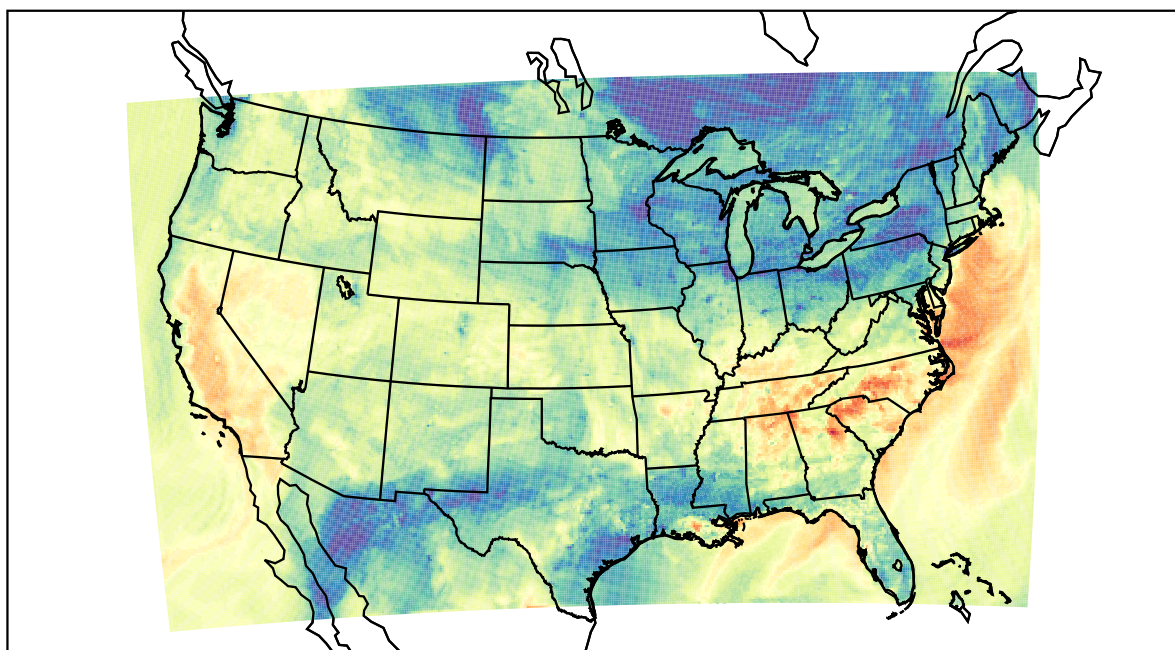
WRF (2019-10-15_00:00:00)
