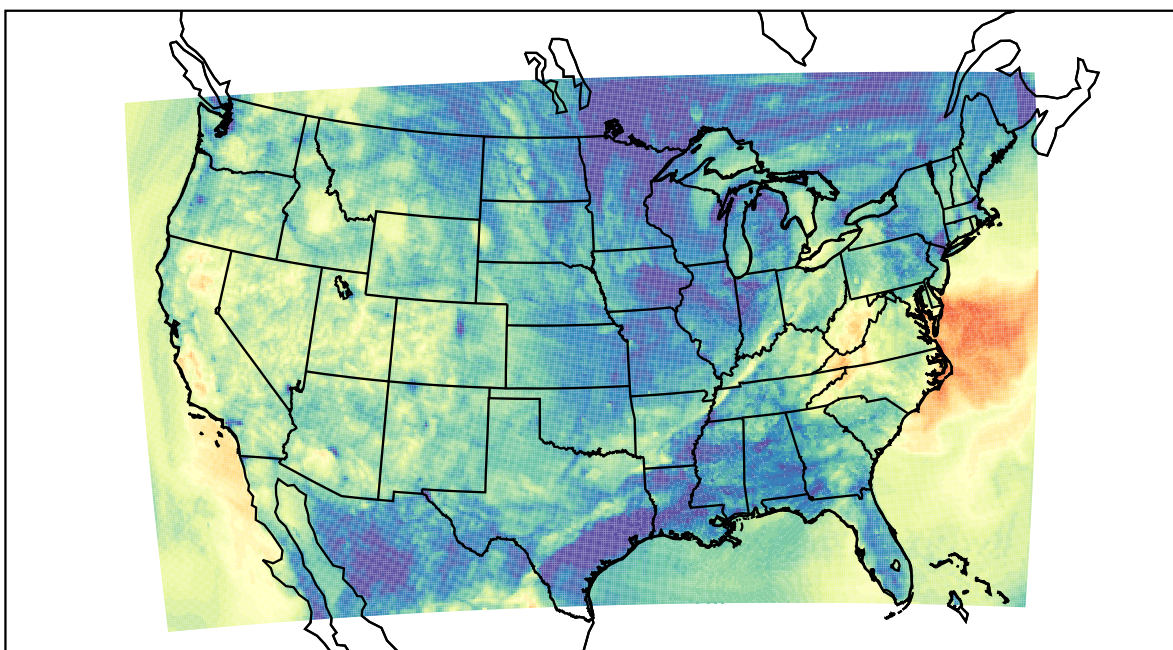
WRF (2019-10-16_05:00:00)
