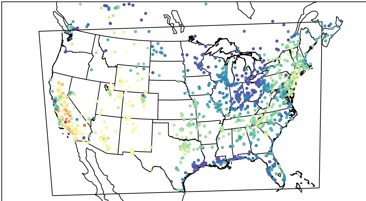
AirNOW (2019-10-16_19:00:00)
