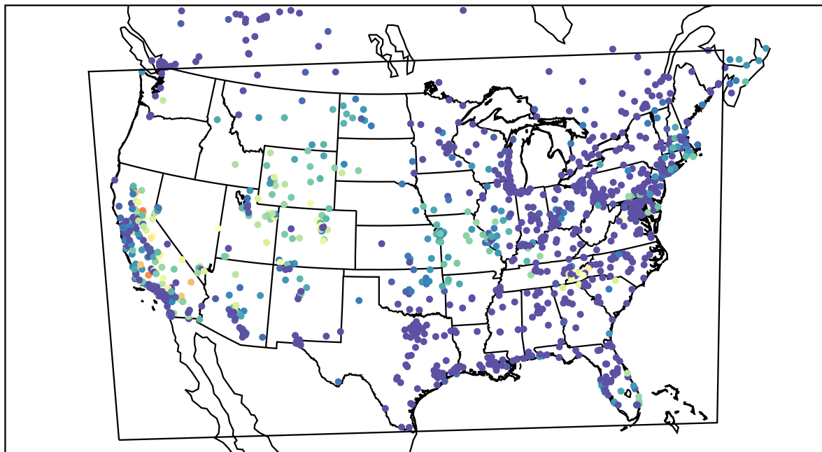
AirNOW (2019-10-15_07:00:00)
