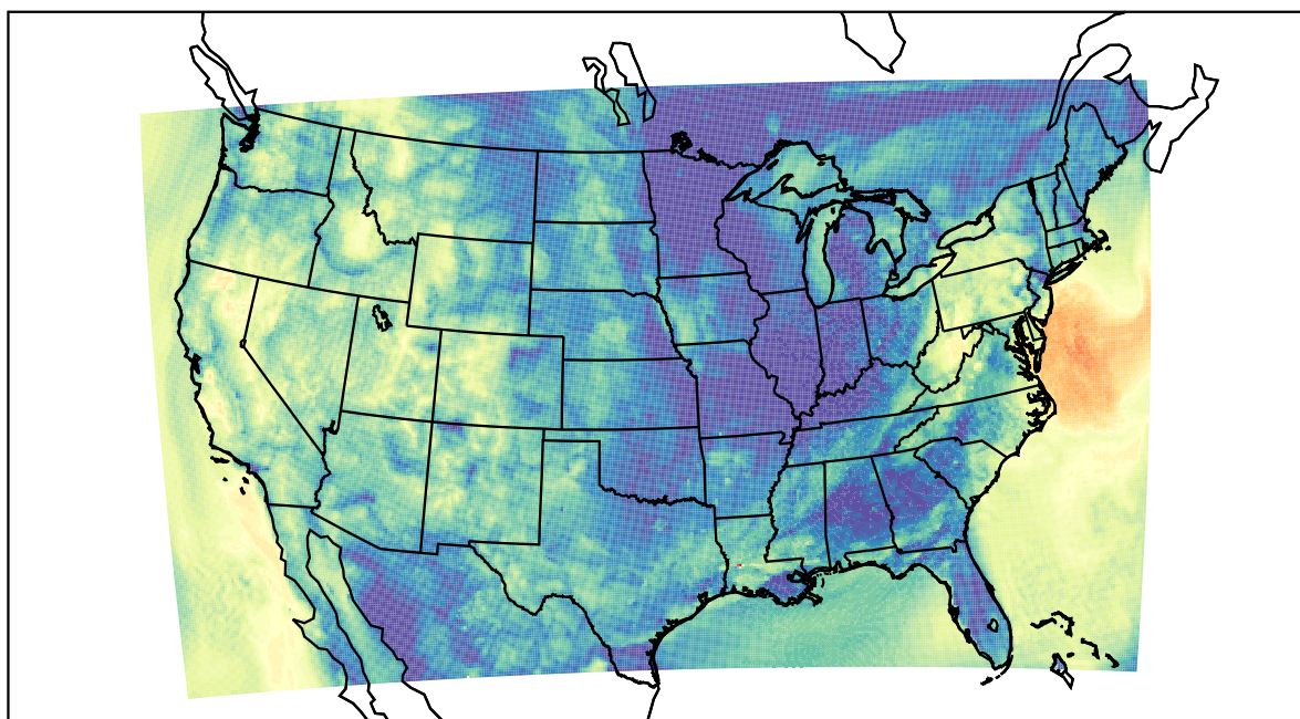
WRF (2019-10-16_12:00:00)
