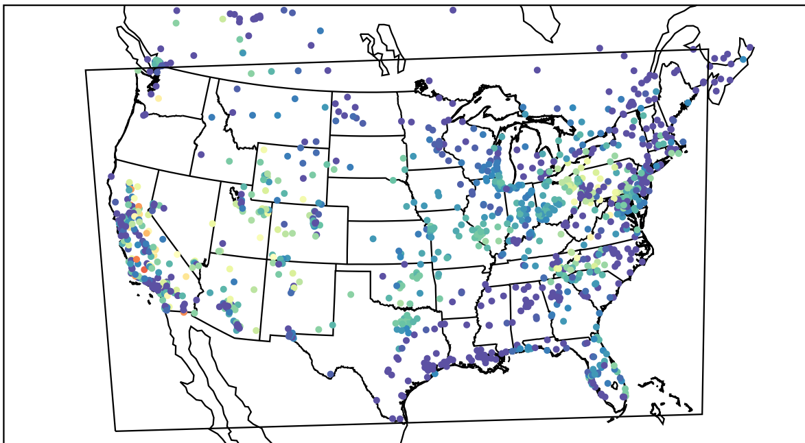
AirNOW (2019-10-16_05:00:00)
