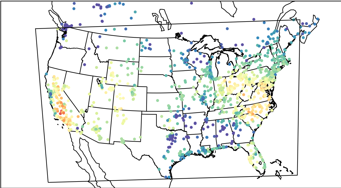
AirNOW (2019-10-15_19:00:00)
