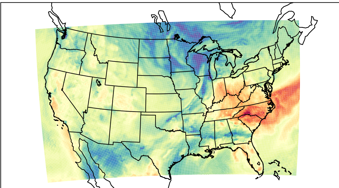
WRF (2019-10-15_19:00:00)
