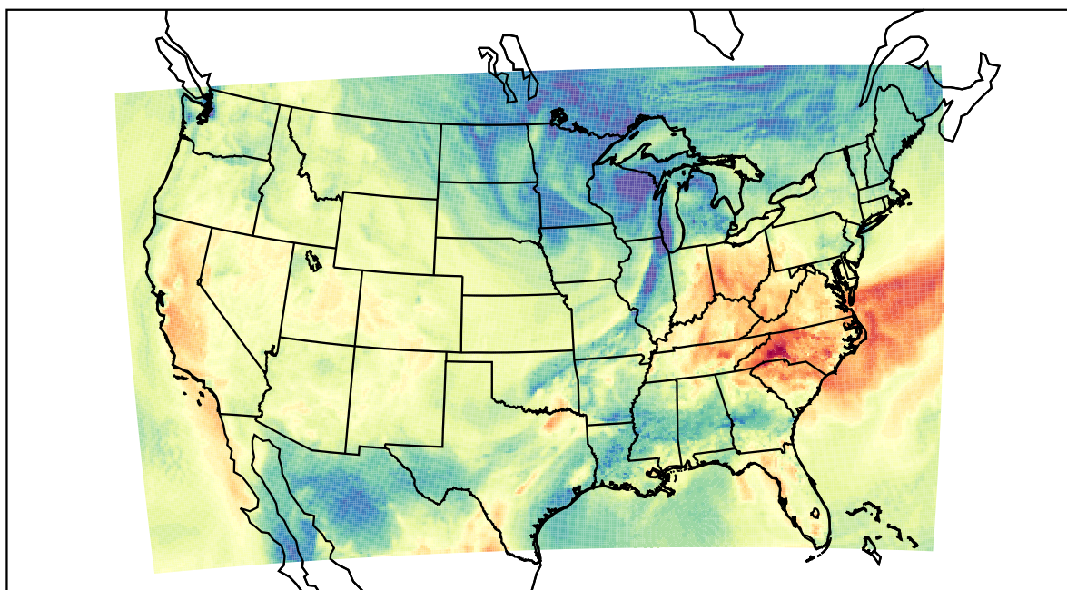
WRF (2019-10-15_21:00:00)
