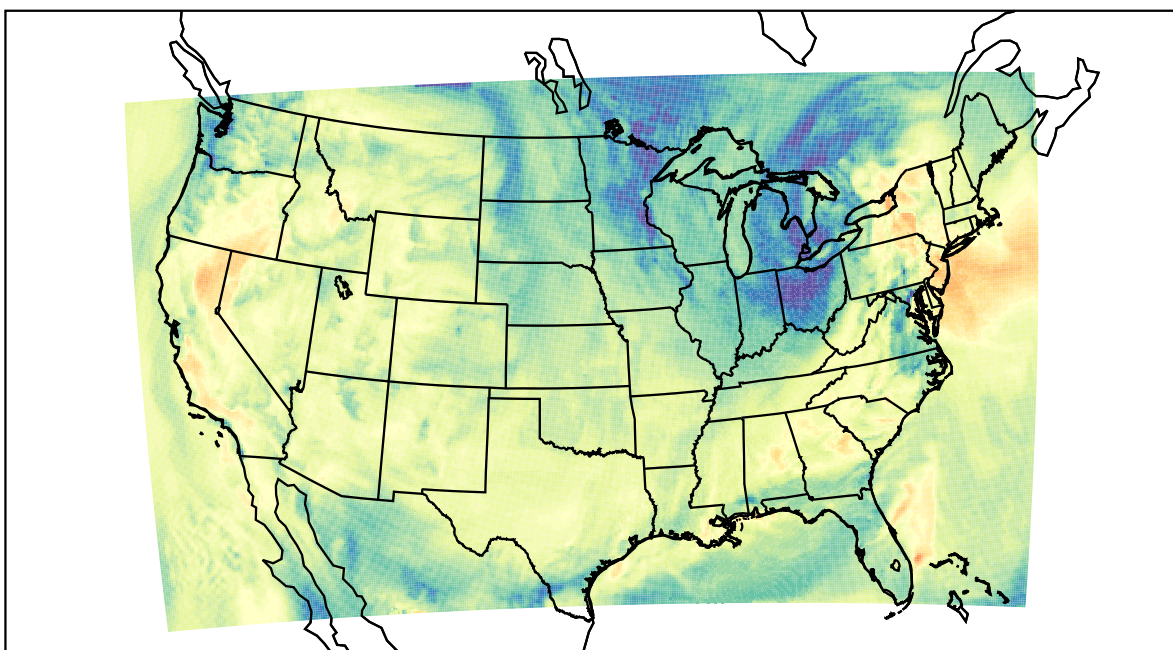
WRF (2019-10-16_19:00:00)
