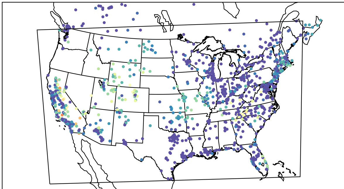
AirNOW (2019-10-15_06:00:00)
