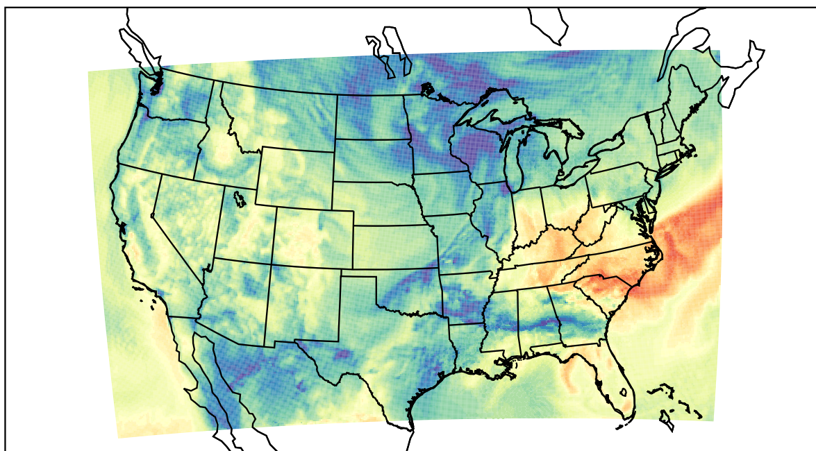
WRF (2019-10-15_17:00:00)
