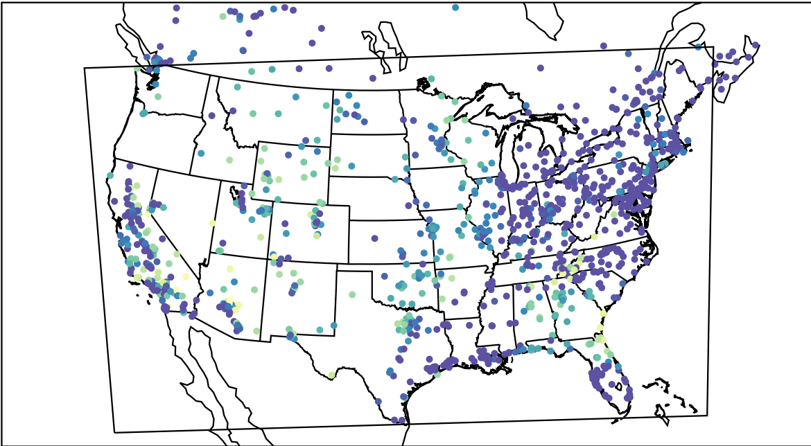
AirNOW (2019-10-19_09:00:00)
