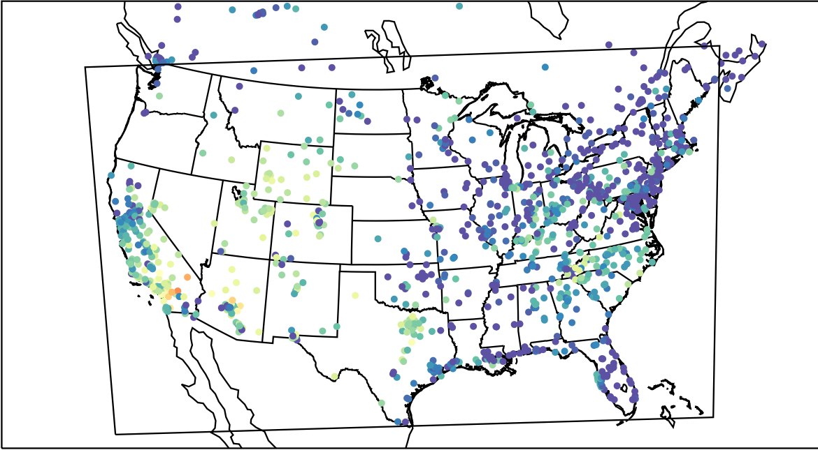
AirNOW (2019-10-20_02:00:00)
