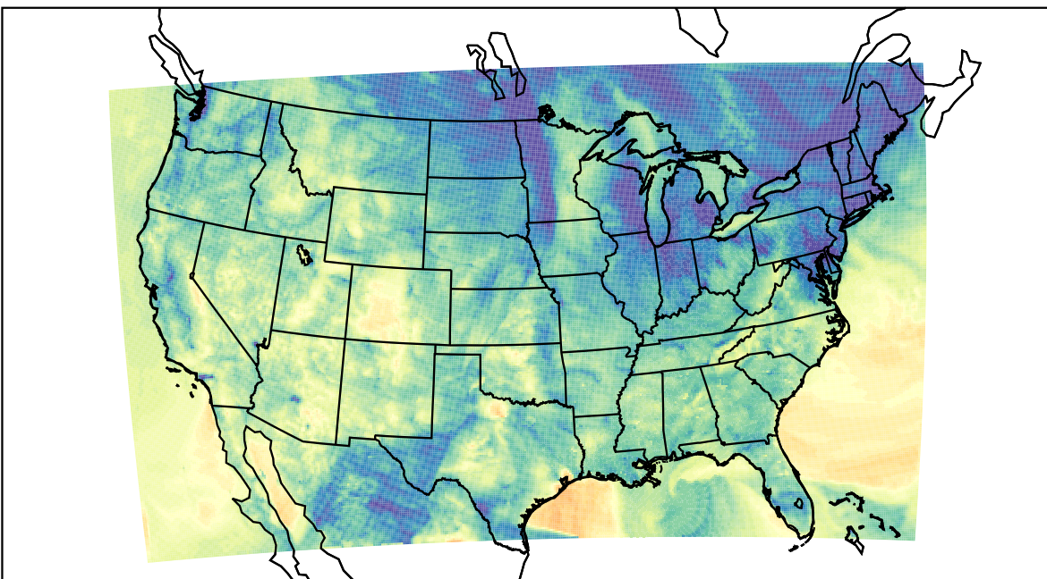
WRF (2019-10-19_05:00:00)
