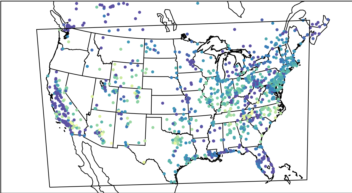
AirNOW (2019-10-19_15:00:00)
