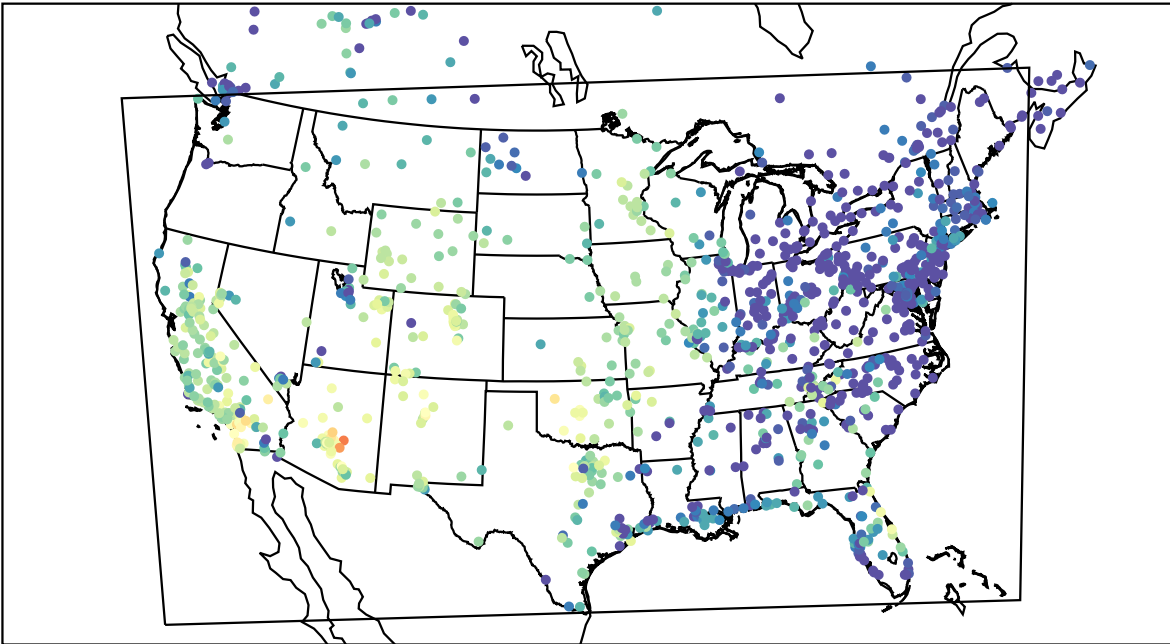
AirNOW (2019-10-19_01:00:00)
