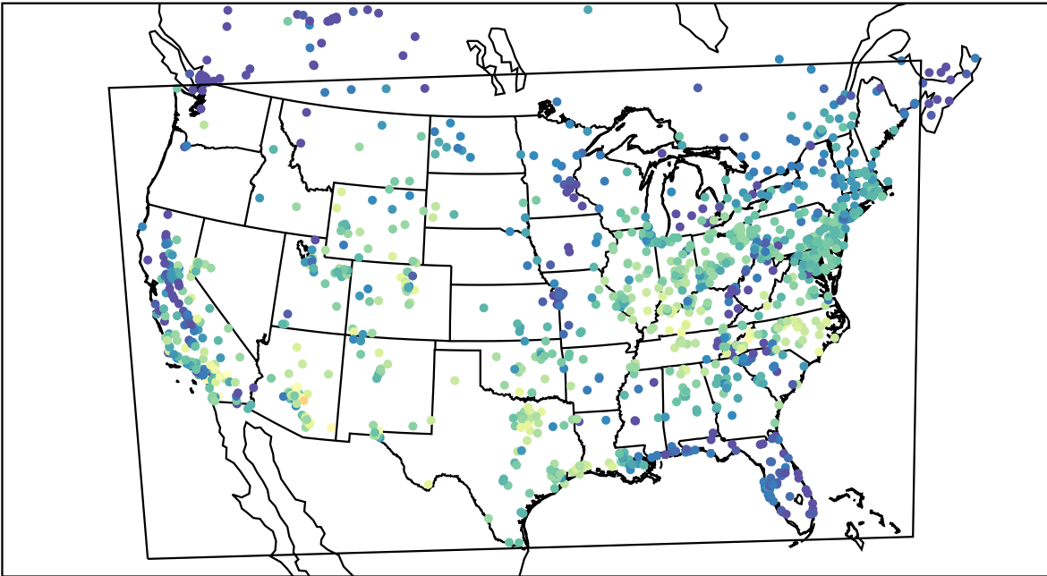
AirNOW (2019-10-19_16:00:00)
