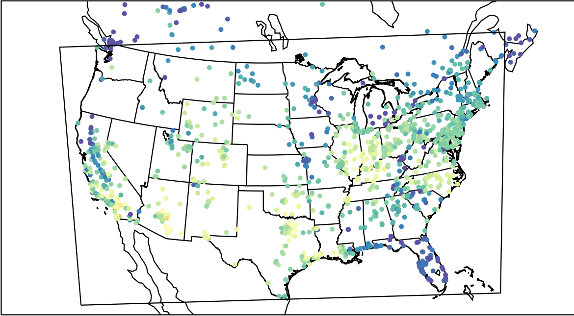
AirNOW (2019-10-19_17:00:00)
