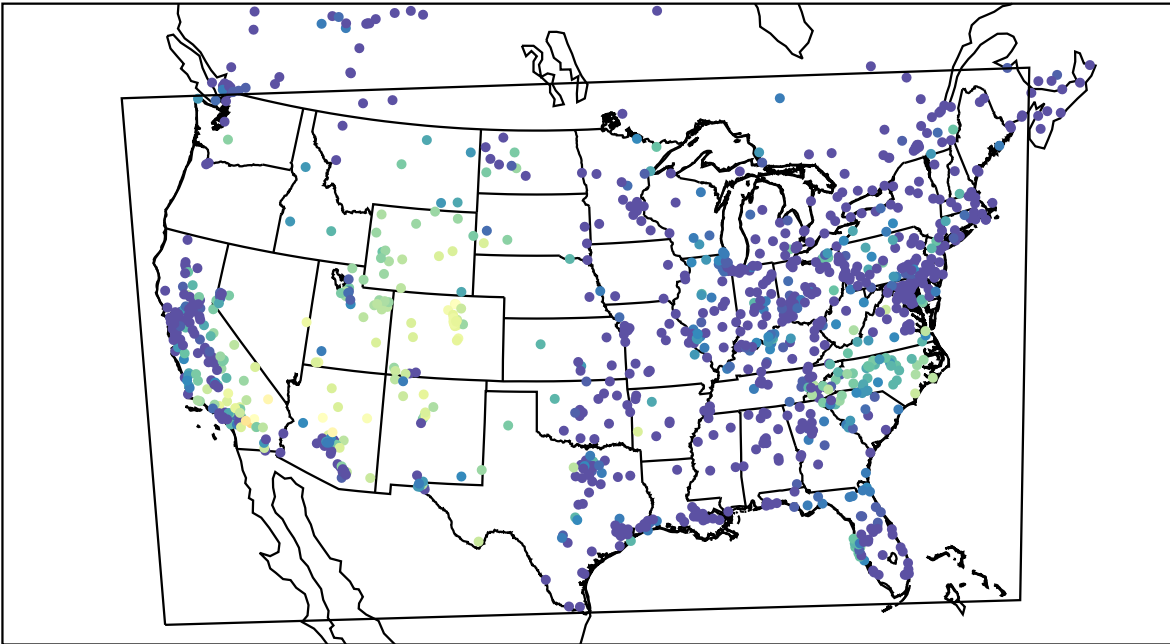
AirNOW (2019-10-20_09:00:00)
