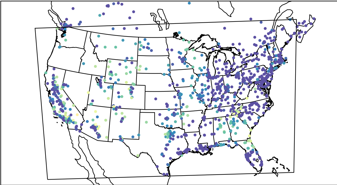
AirNOW (2019-10-19_10:00:00)
