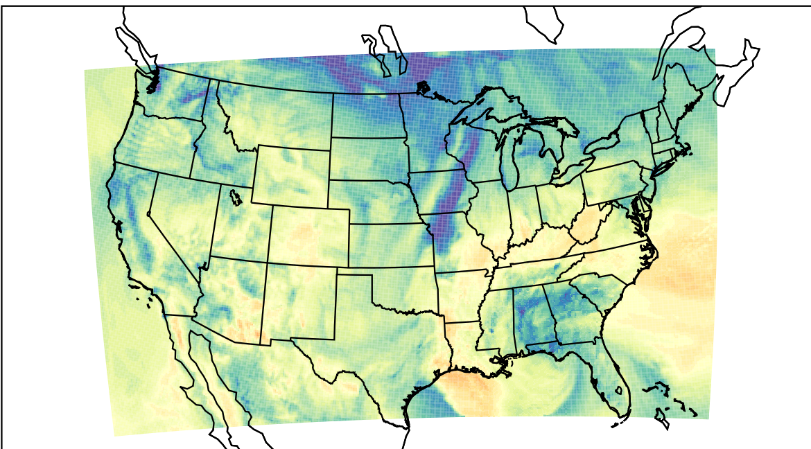
WRF (2019-10-19_17:00:00)
