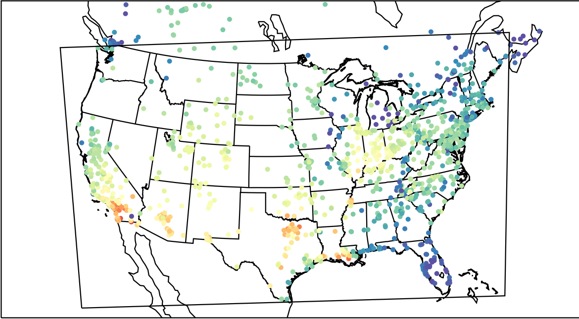
AirNOW (2019-10-19_21:00:00)
