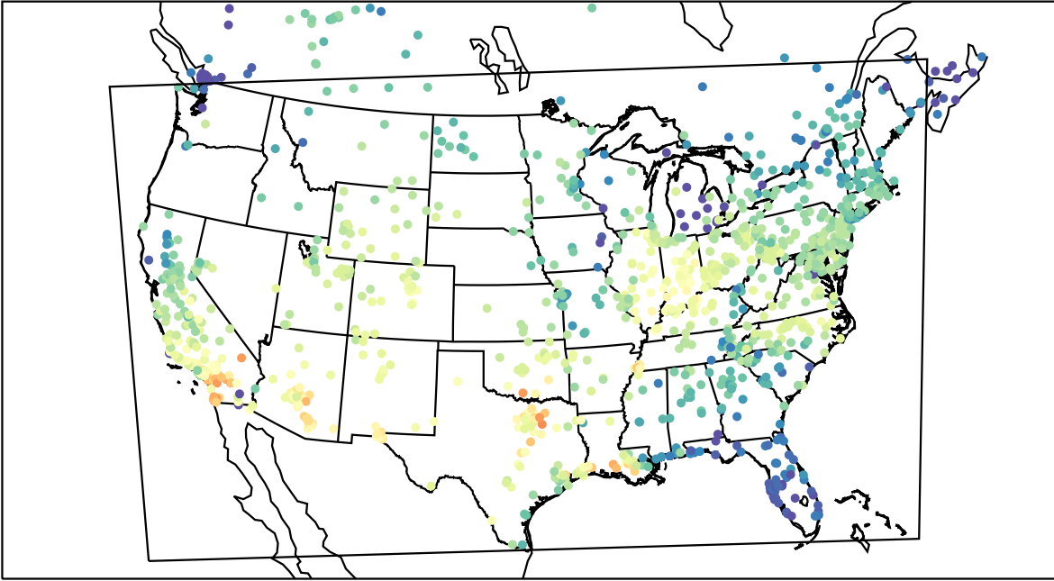
AirNOW (2019-10-19_19:00:00)
