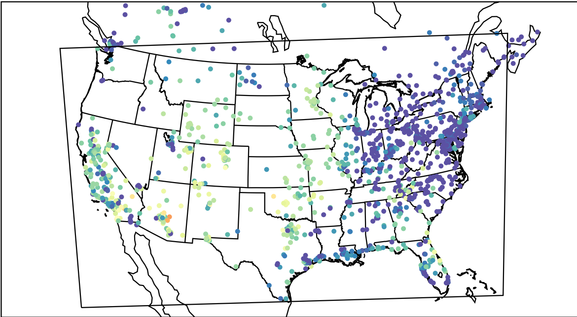
AirNOW (2019-10-19_02:00:00)
