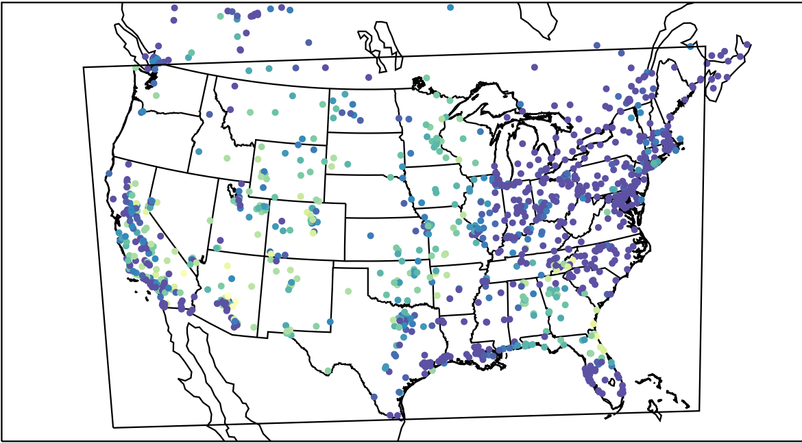
AirNOW (2019-10-19_07:00:00)
