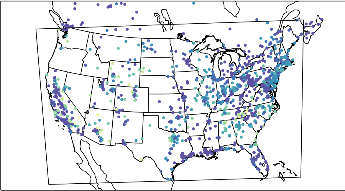
AirNOW (2019-10-19_14:00:00)
