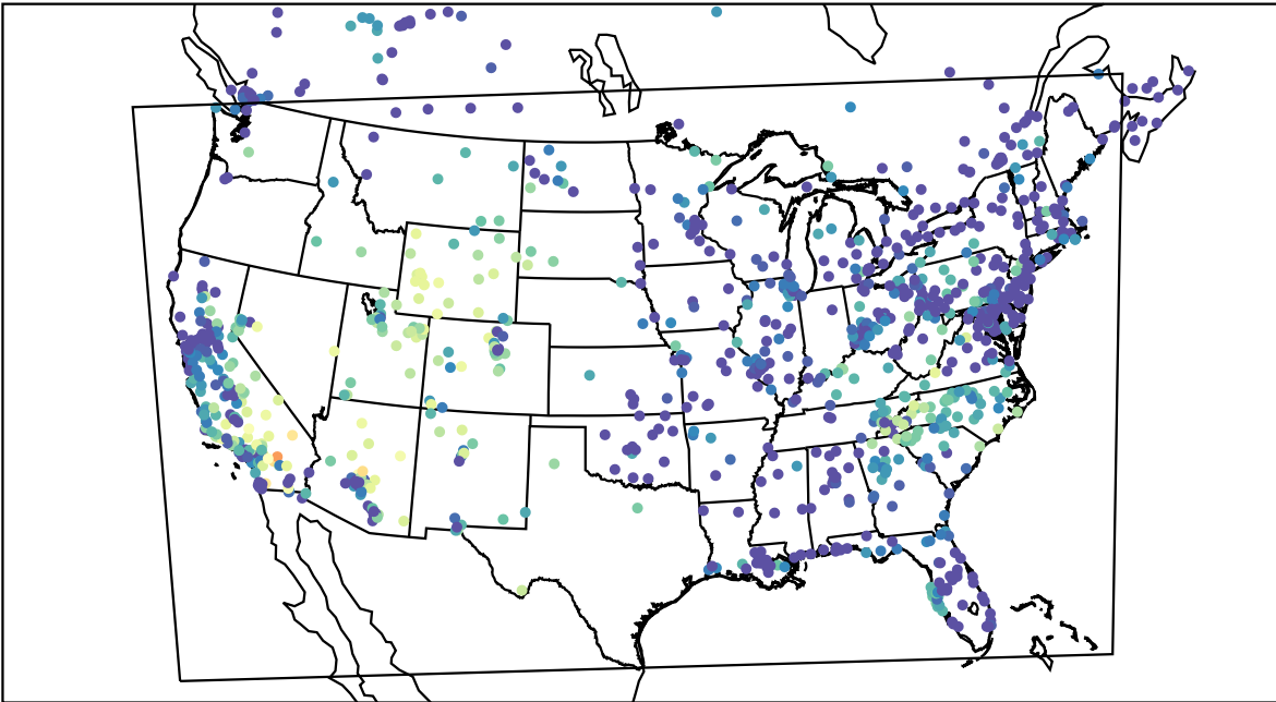
AirNOW (2019-10-20_05:00:00)
