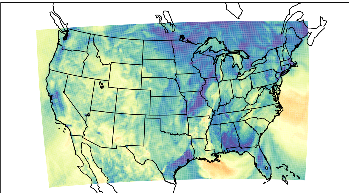
WRF (2019-10-20_05:00:00)
