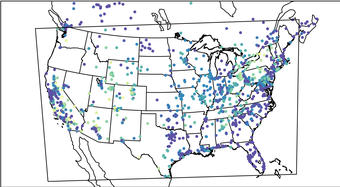
AirNOW (2019-10-22_07:00:00)
