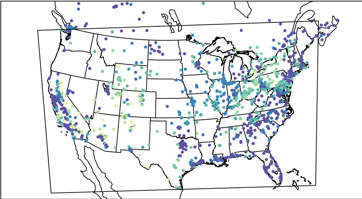
AirNOW (2019-10-22_05:00:00)
