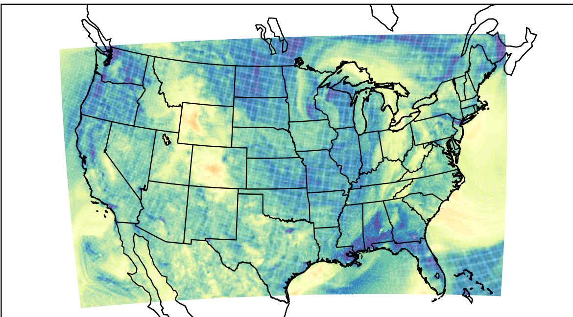
WRF (2019-10-22_05:00:00)
