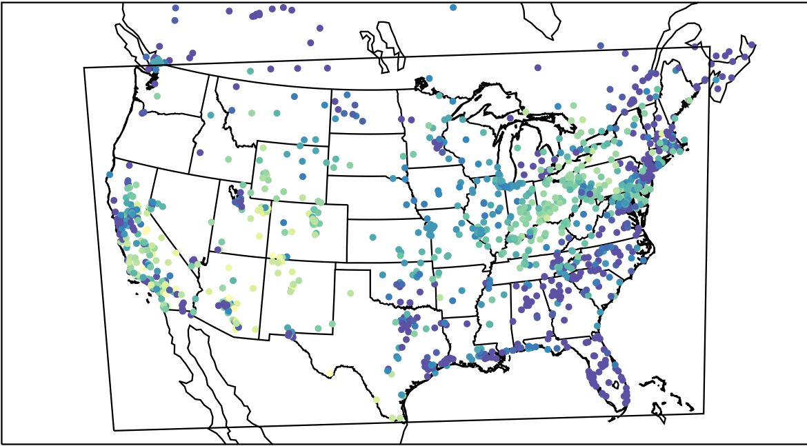
AirNOW (2019-10-22_02:00:00)
