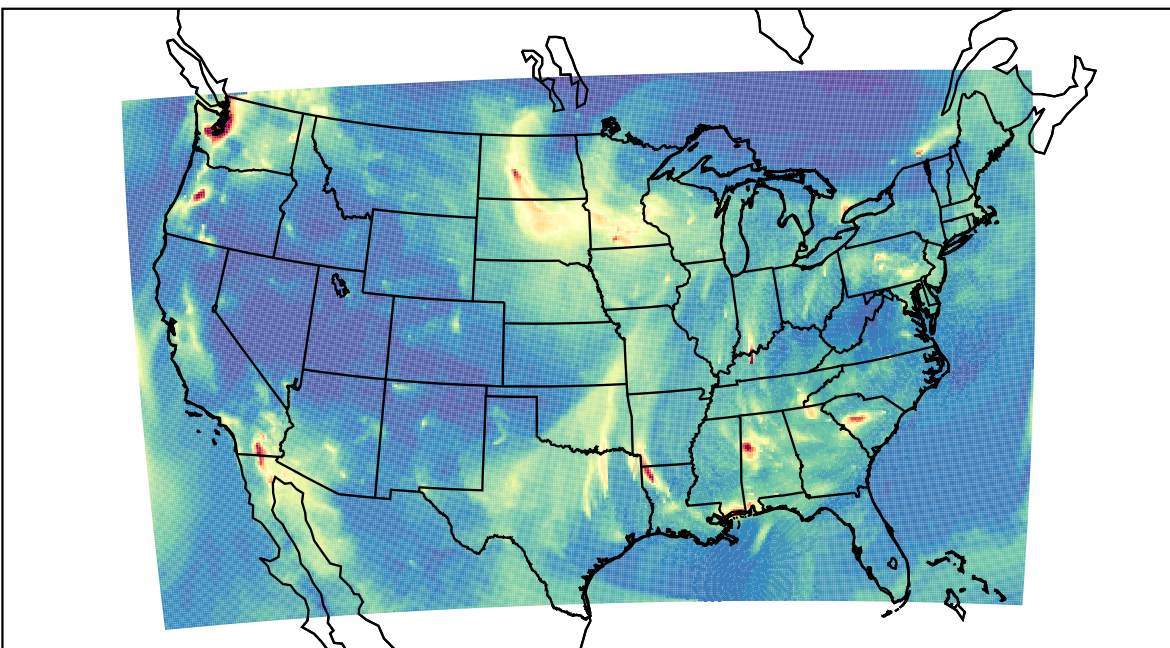
WRF 2019-11-04_07:00:00
