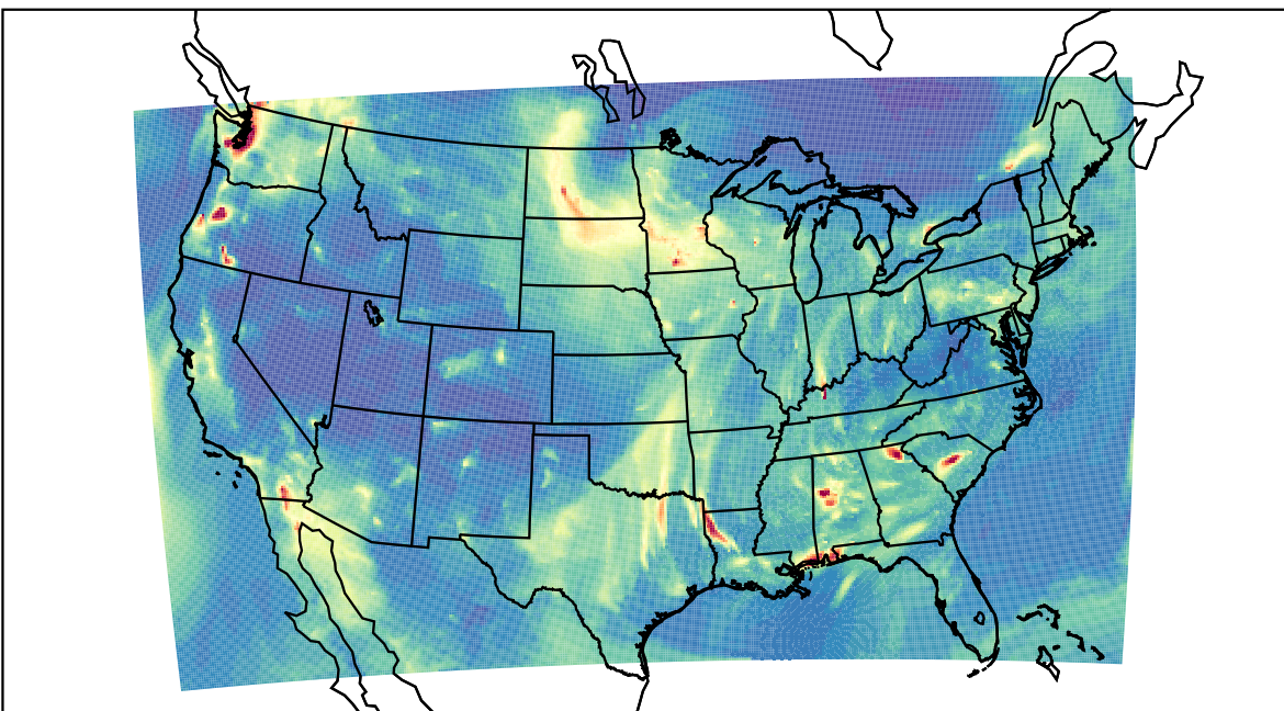
WRF 2019-11-04_05:00:00
