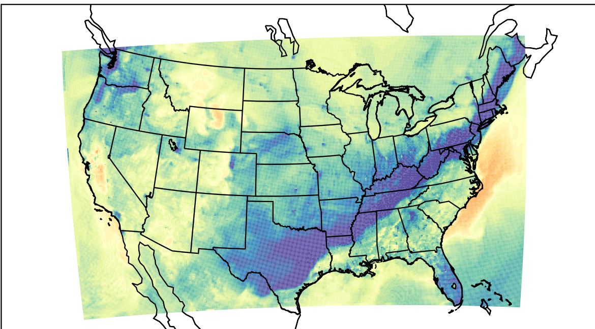
WRF (2019-11-08_00:00:00)
