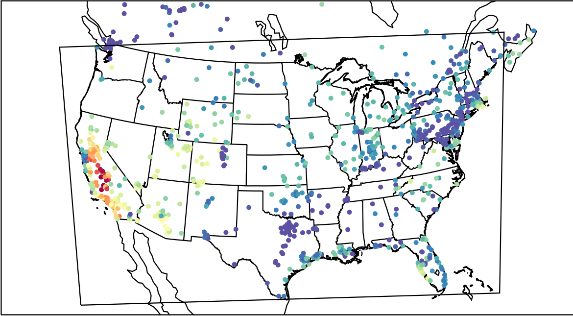
AirNOW (2019-11-07_22:00:00)
