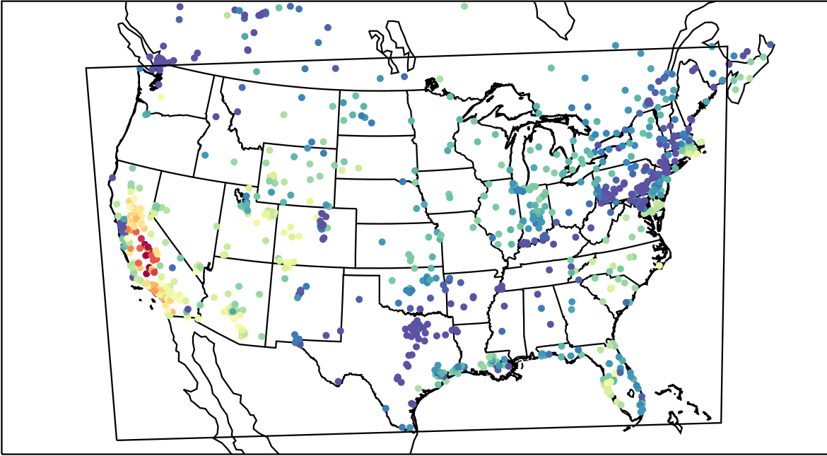
AirNOW (2019-11-07_21:00:00)
