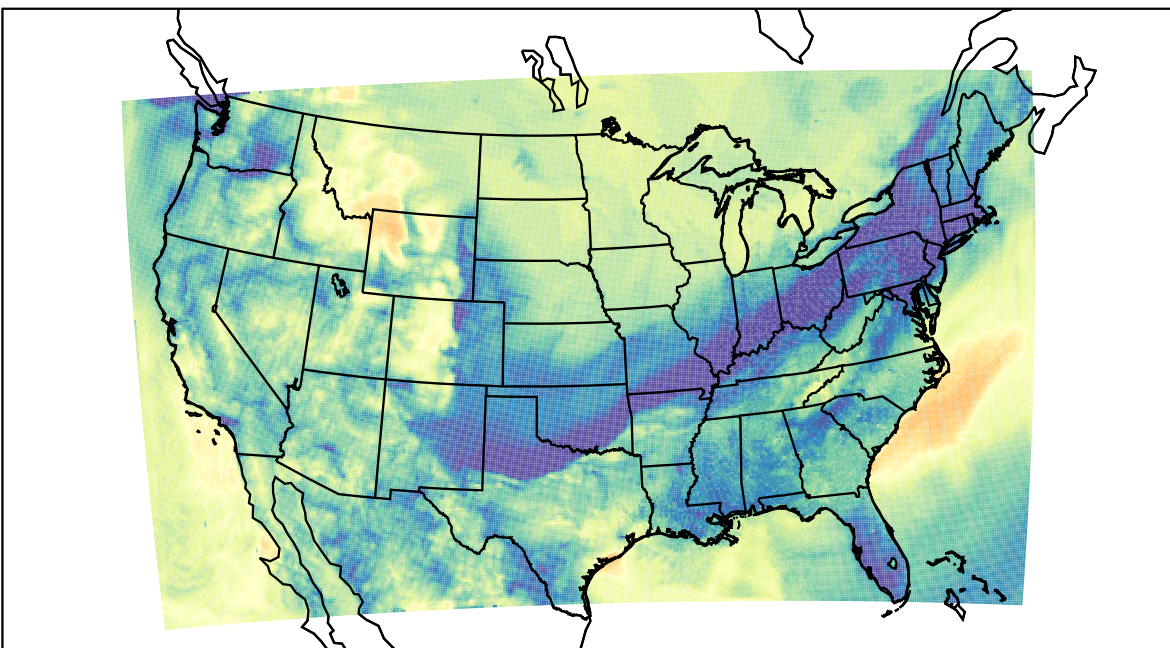
WRF (2019-11-07_11:00:00)
