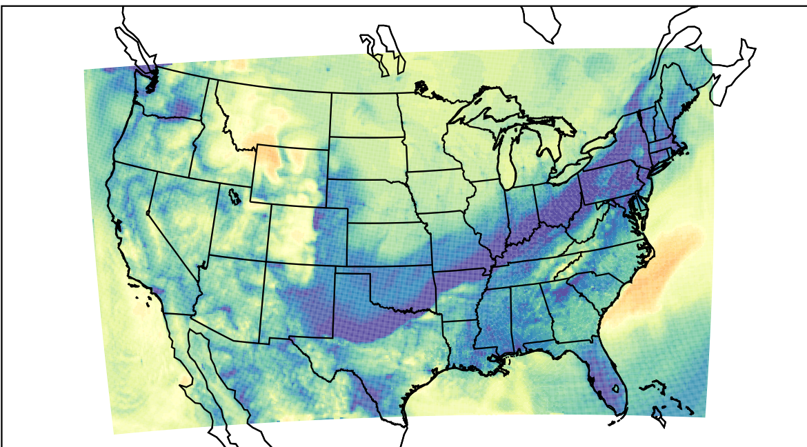
WRF (2019-11-07_13:00:00)
