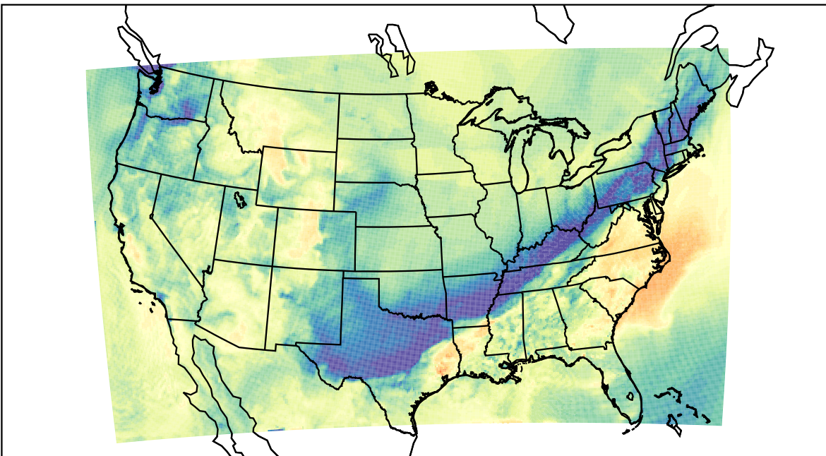
WRF (2019-11-07_19:00:00)
