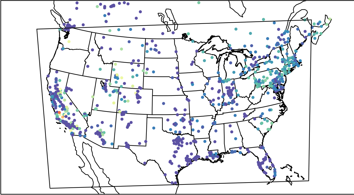
AirNOW (2019-11-08_07:00:00)
