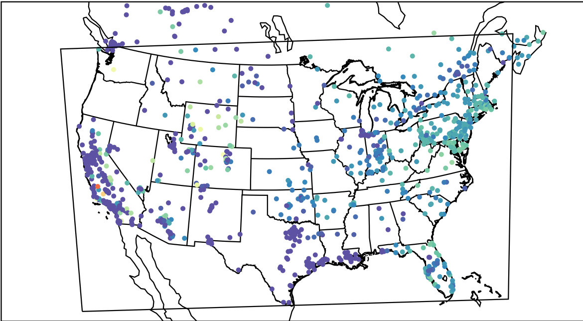
AirNOW (2019-11-08_15:00:00)
