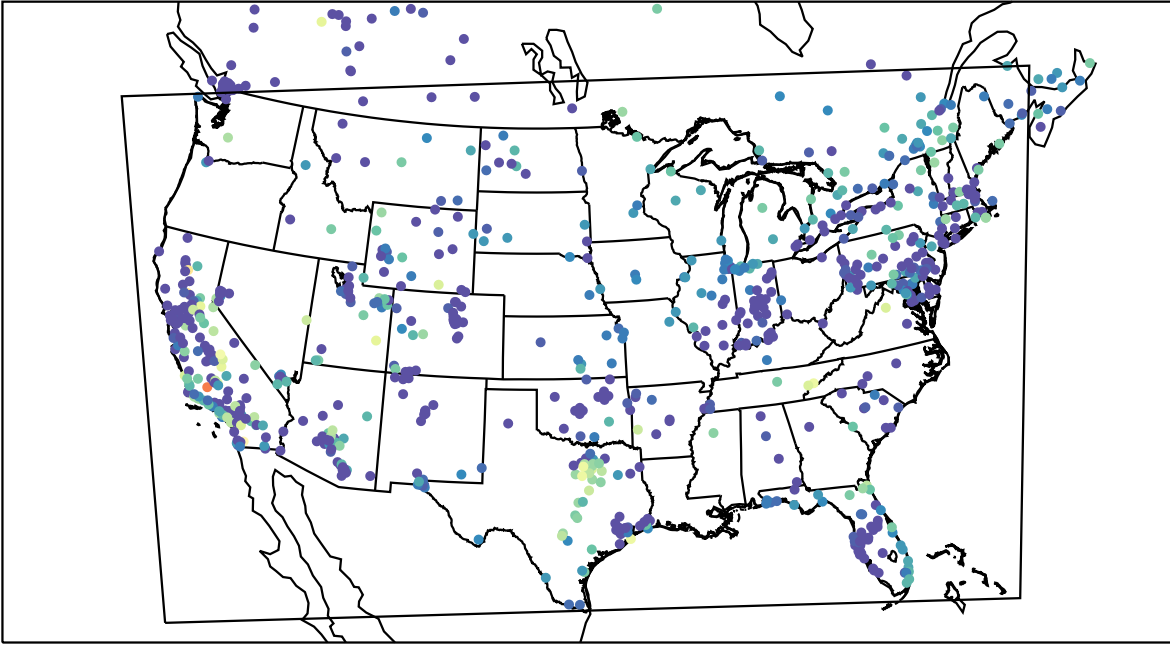
AirNOW (2019-11-07_07:00:00)
