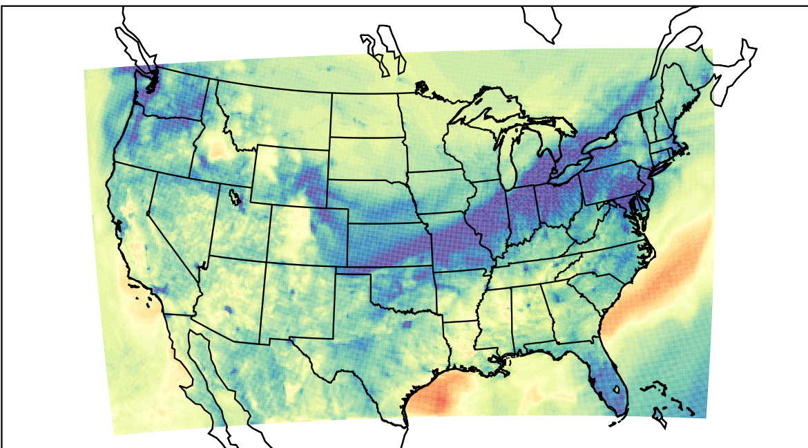
WRF (2019-11-07_02:00:00)
