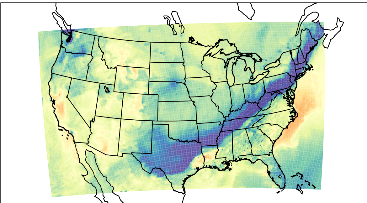
WRF (2019-11-07_22:00:00)
