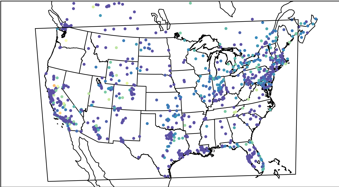
AirNOW (2019-11-07_12:00:00)
