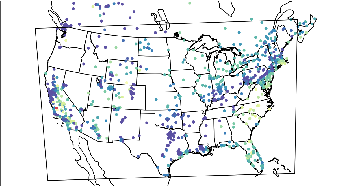
AirNOW (2019-11-07_17:00:00)
