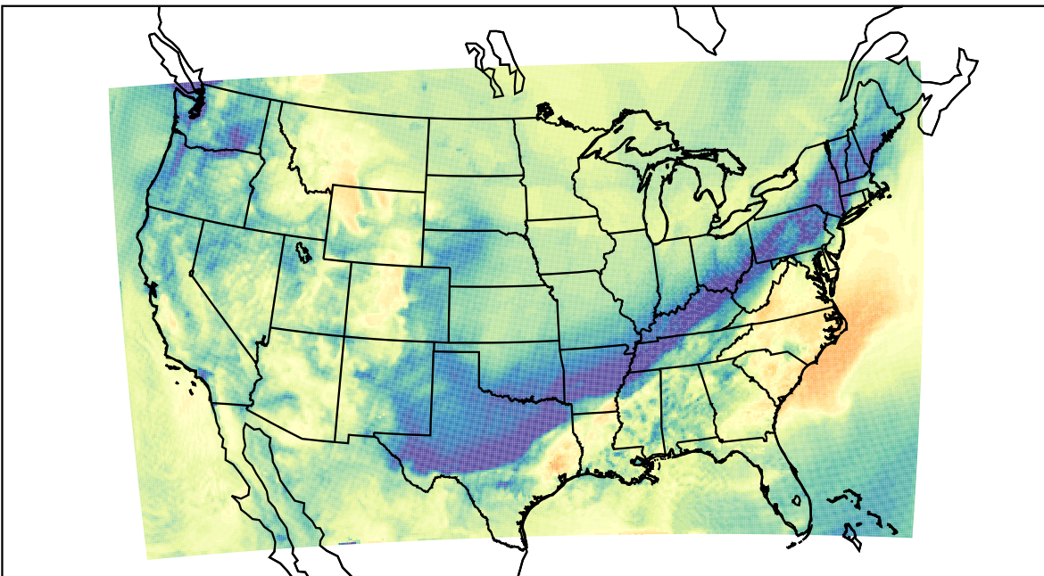
WRF (2019-11-07_18:00:00)
