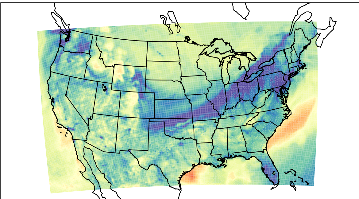
WRF (2019-11-07_05:00:00)
