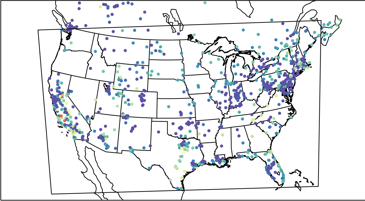
AirNOW (2019-11-07_03:00:00)
