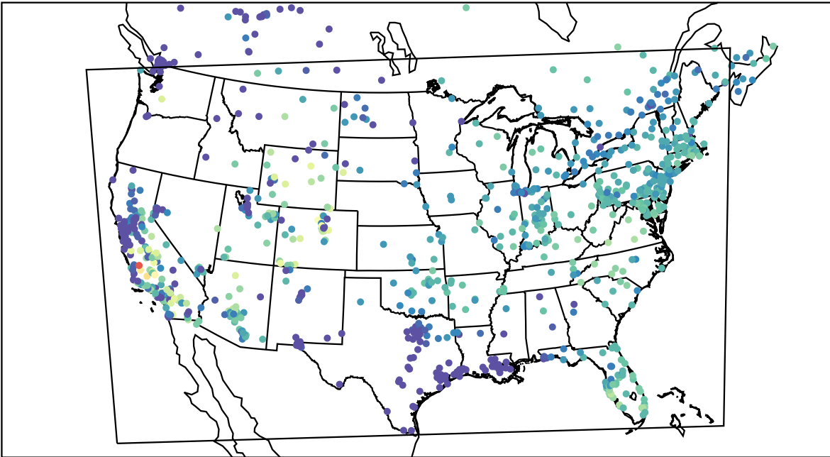
AirNOW (2019-11-08_17:00:00)
