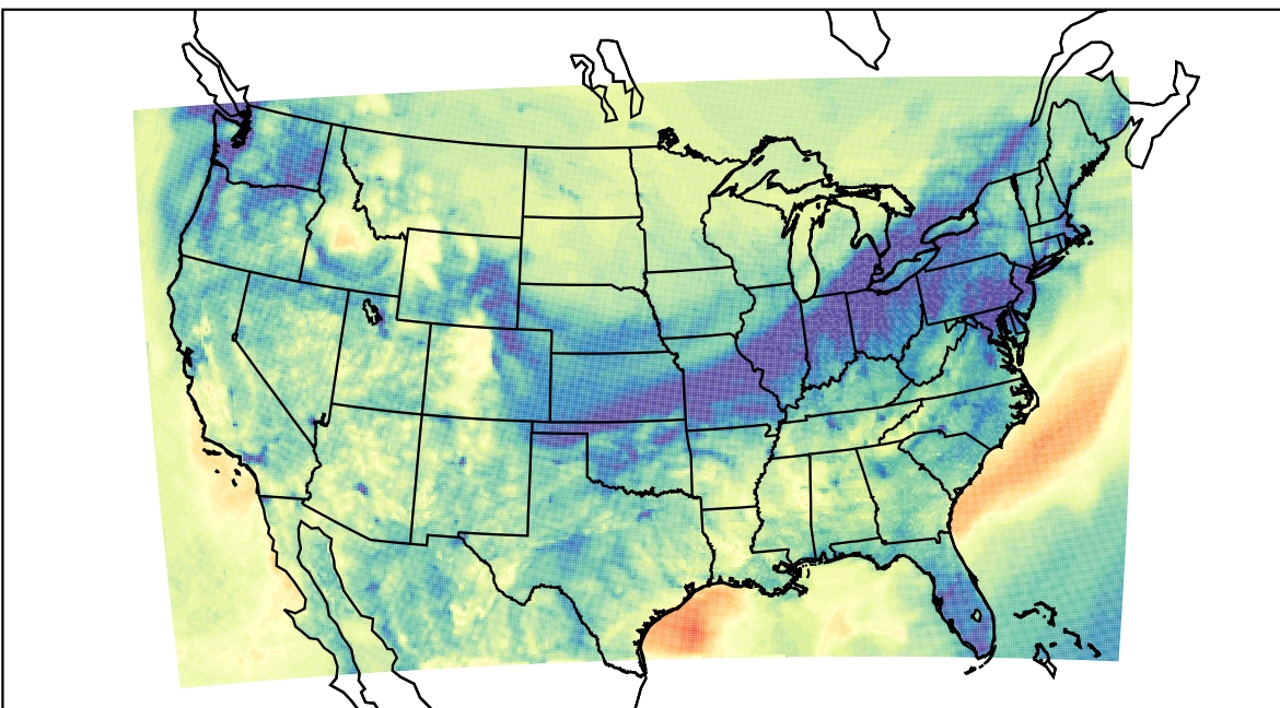
WRF (2019-11-07_03:00:00)
