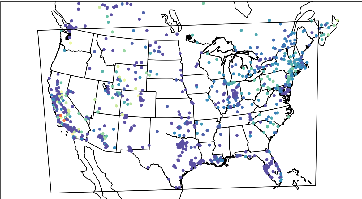
AirNOW (2019-11-08_06:00:00)
