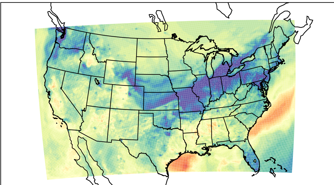
WRF (2019-11-07_00:00:00)
