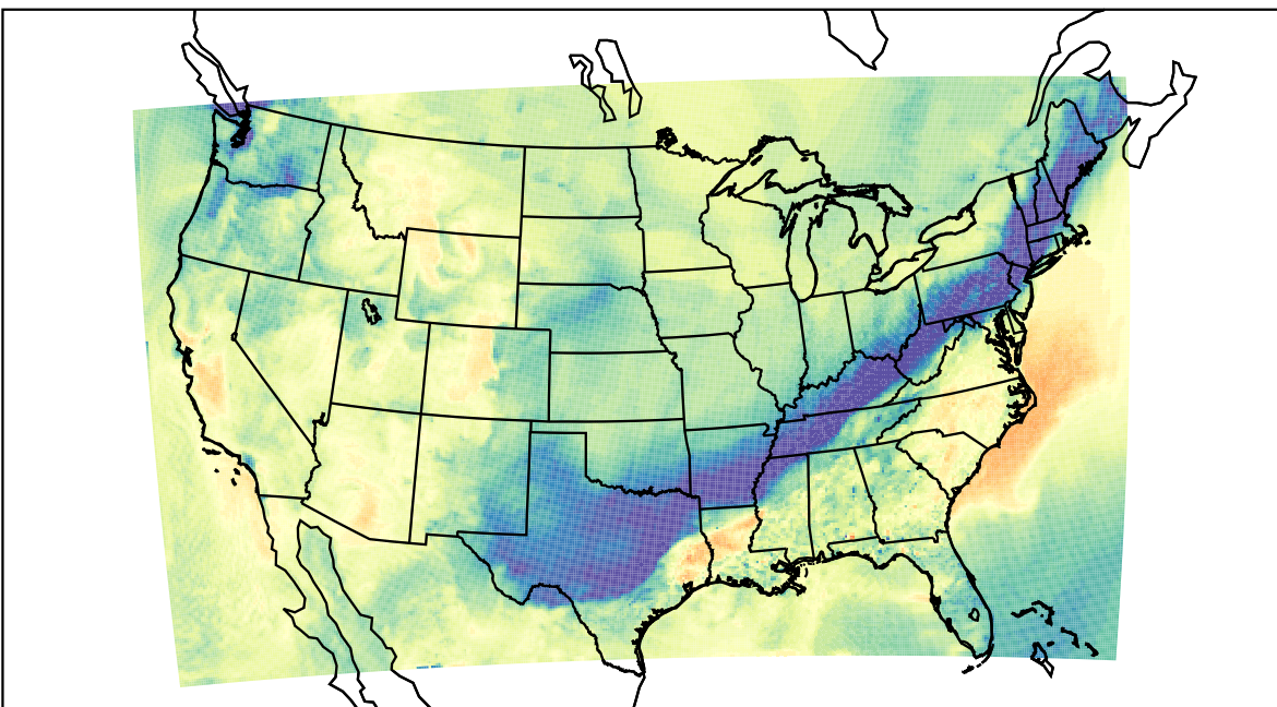
WRF (2019-11-07_21:00:00)
