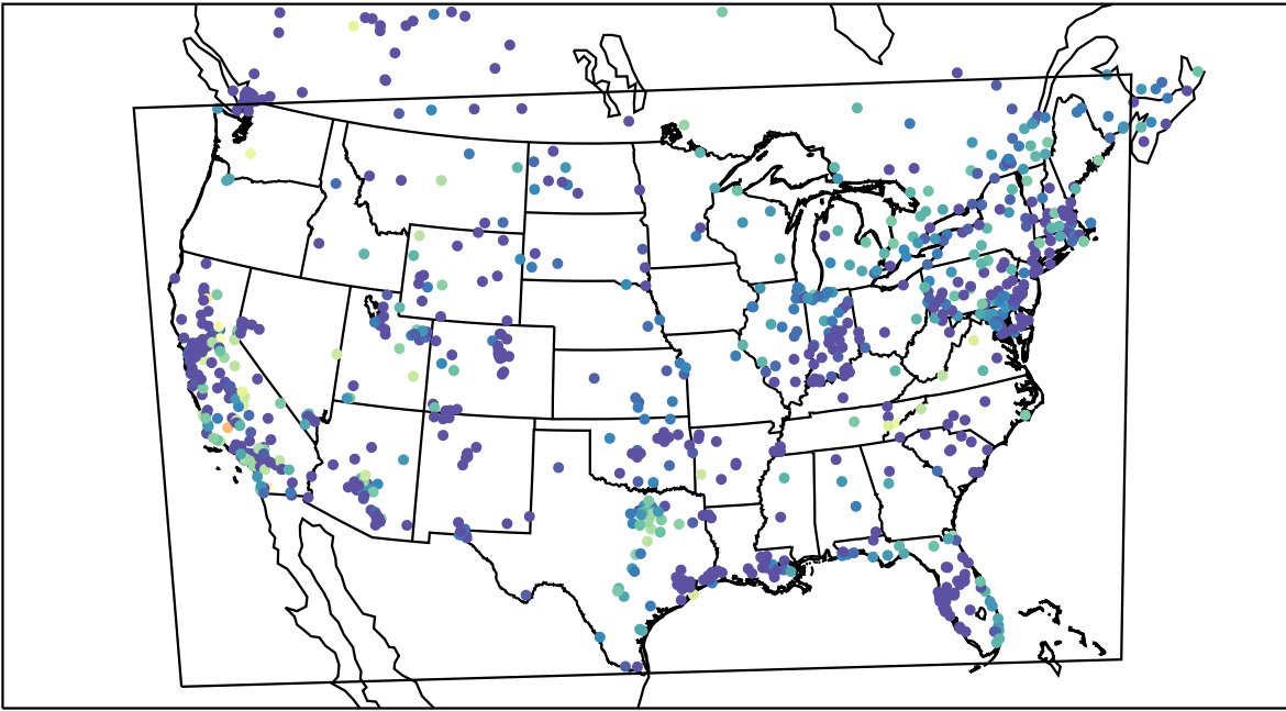
AirNOW (2019-11-07_09:00:00)
