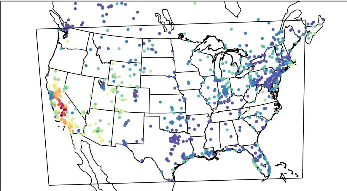
AirNOW (2019-11-07_23:00:00)
