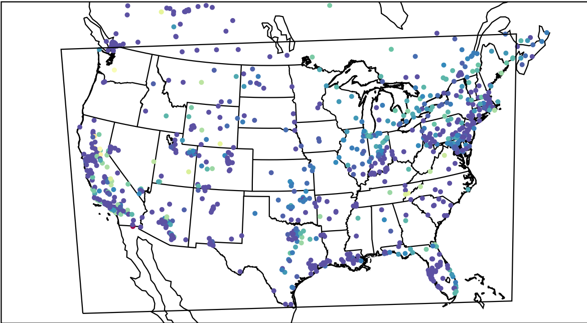
AirNOW (2019-11-07_11:00:00)
