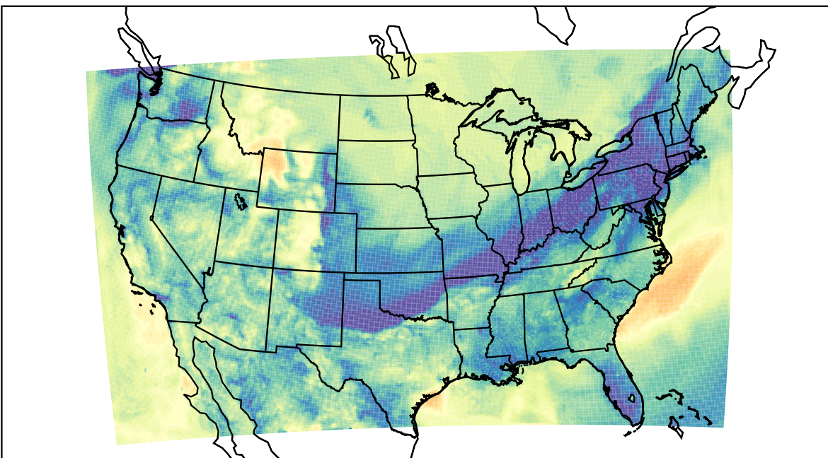
WRF (2019-11-07_10:00:00)
