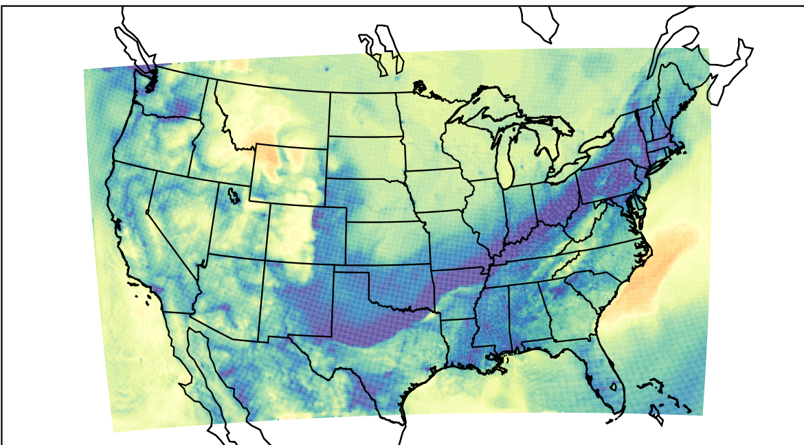
WRF (2019-11-07_14:00:00)
