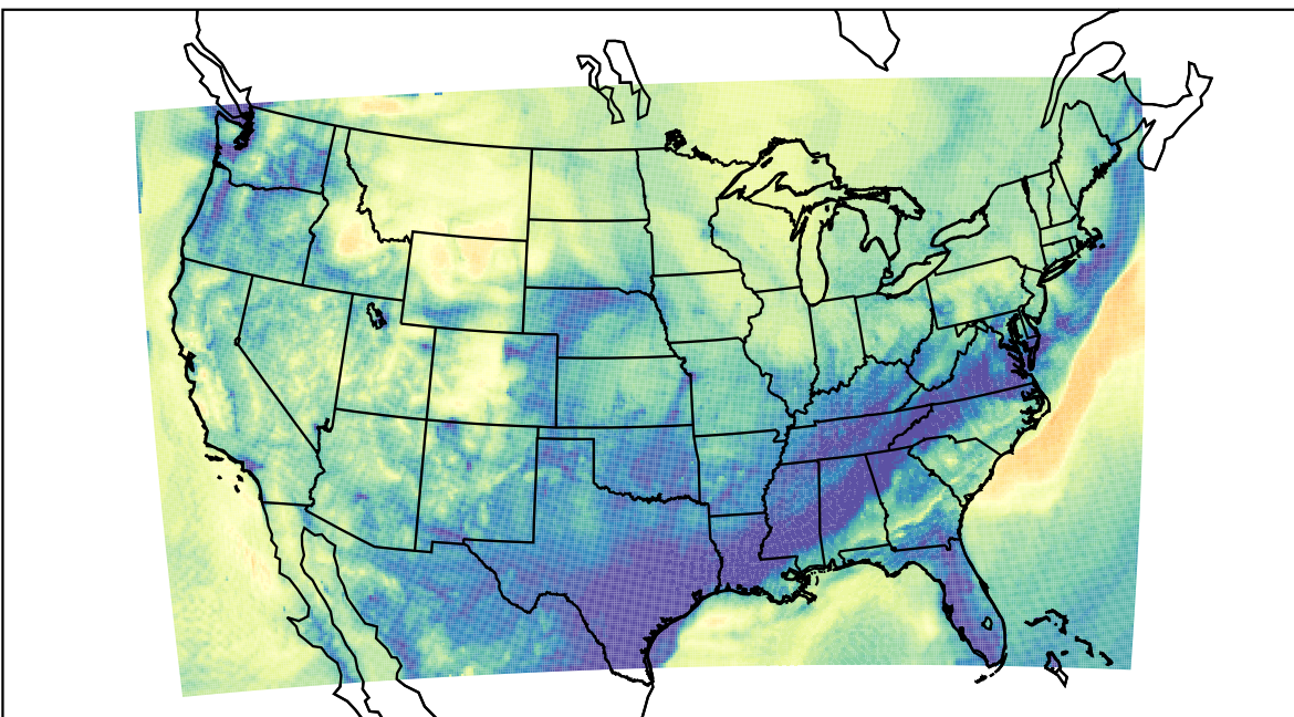
WRF (2019-11-08_07:00:00)
