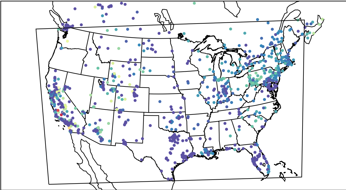
AirNOW (2019-11-08_05:00:00)
