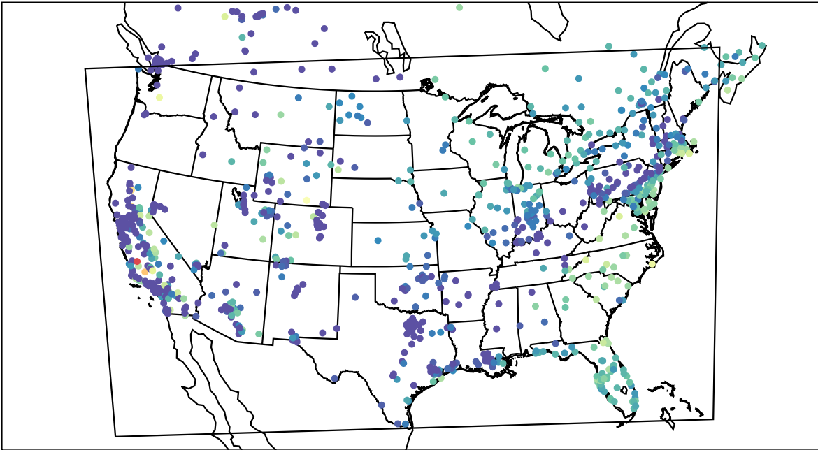
AirNOW (2019-11-07_16:00:00)
