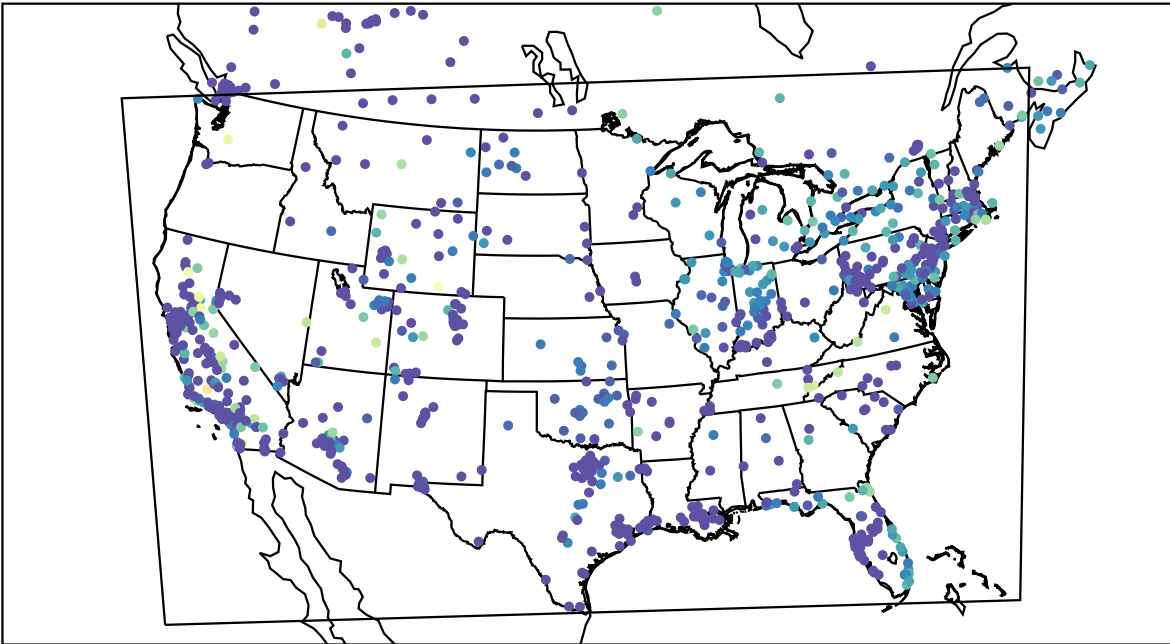
AirNOW (2019-11-07_13:00:00)
