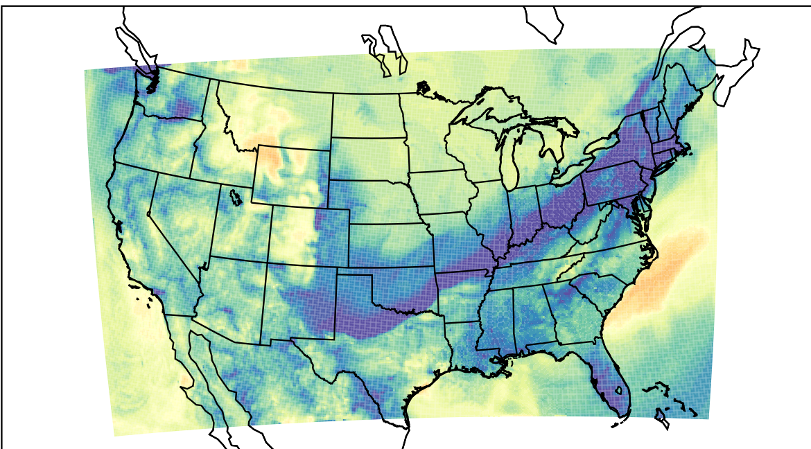
WRF (2019-11-07_12:00:00)
