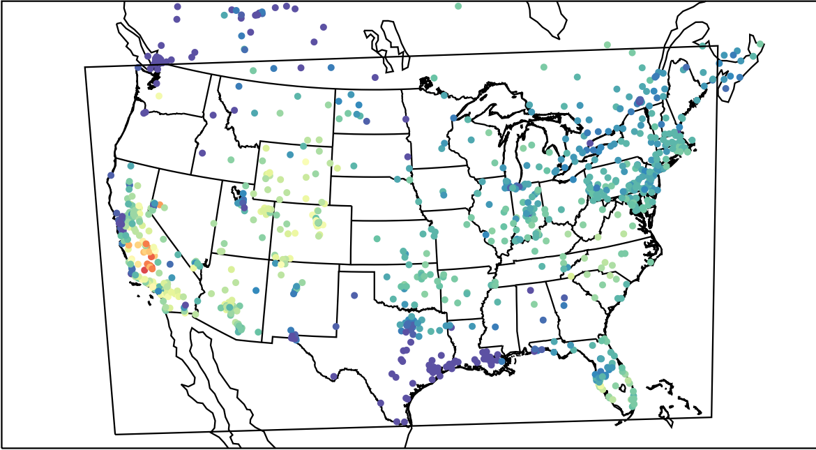
AirNOW (2019-11-08_19:00:00)
