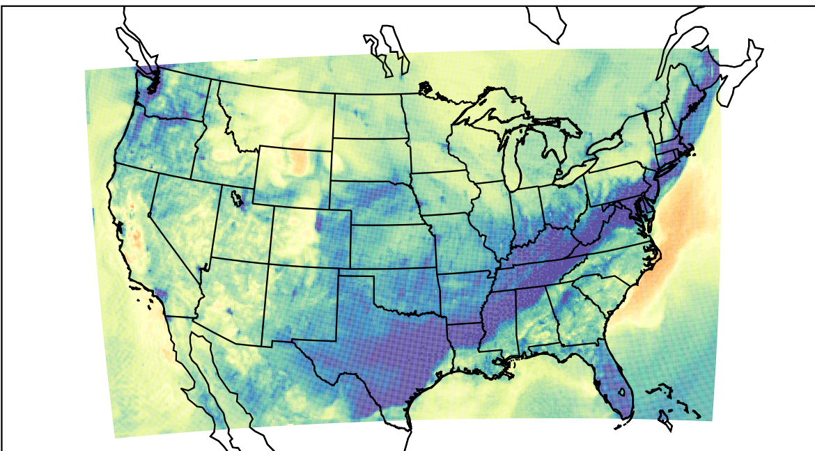
WRF (2019-11-08_02:00:00)
