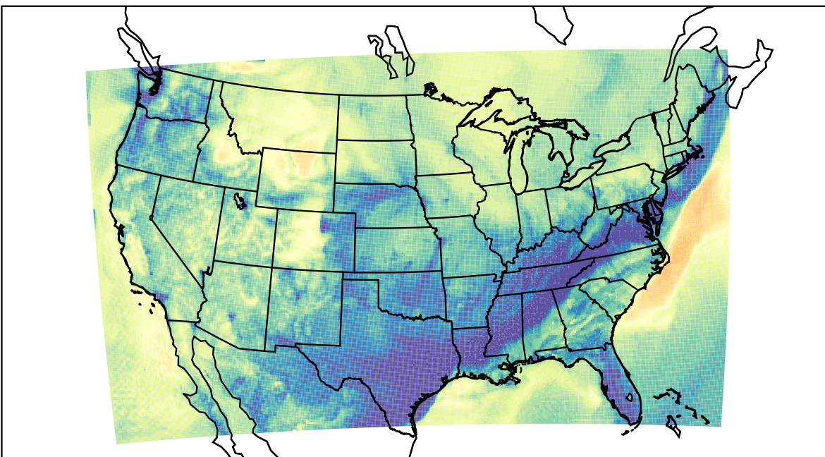
WRF (2019-11-08_05:00:00)
