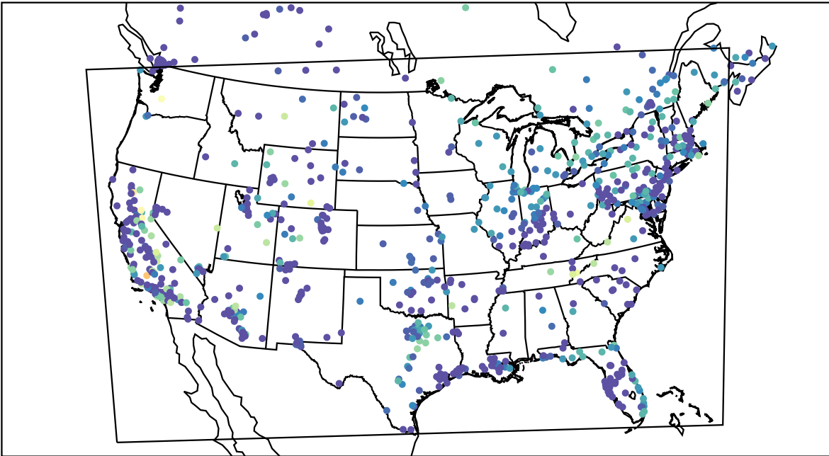
AirNOW (2019-11-07_10:00:00)
