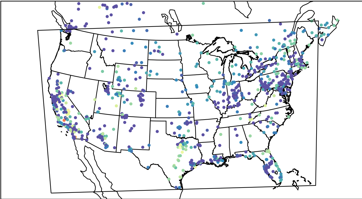
AirNOW (2019-11-07_05:00:00)
