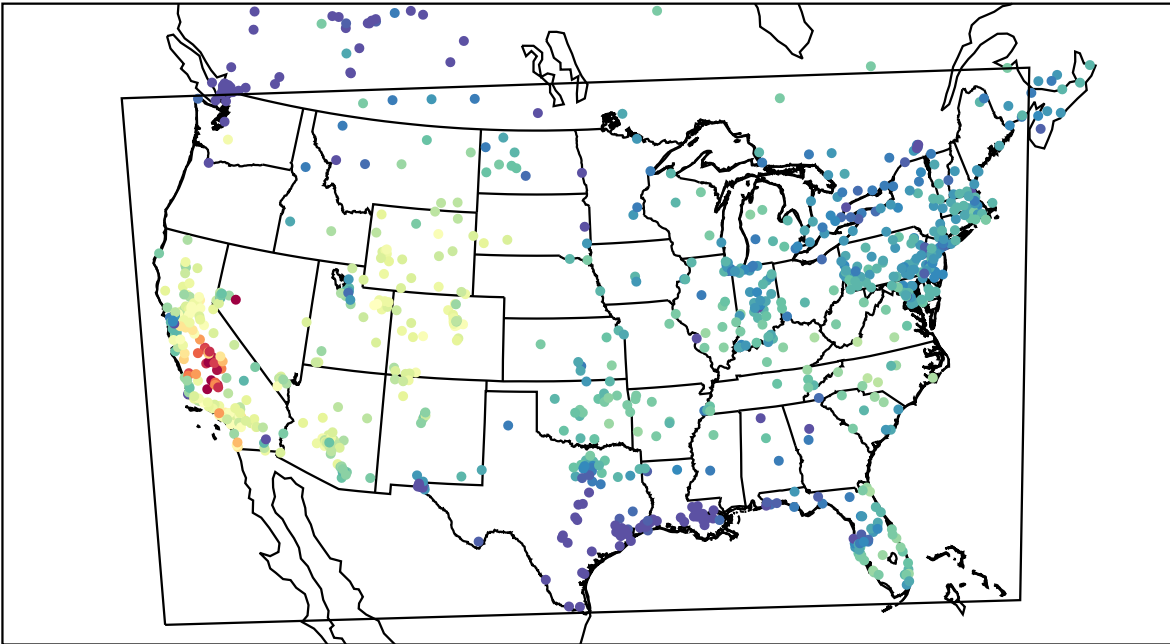
AirNOW (2019-11-08_21:00:00)
