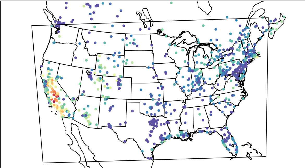
AirNOW (2019-11-08_00:00:00)
