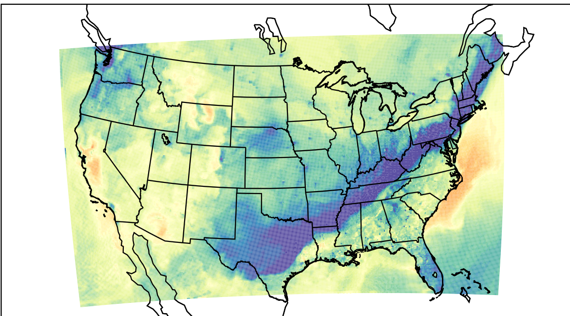
WRF (2019-11-07_23:00:00)
