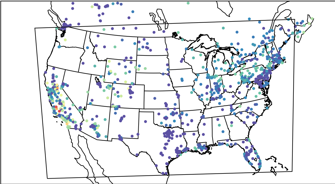
AirNOW (2019-11-08_02:00:00)
