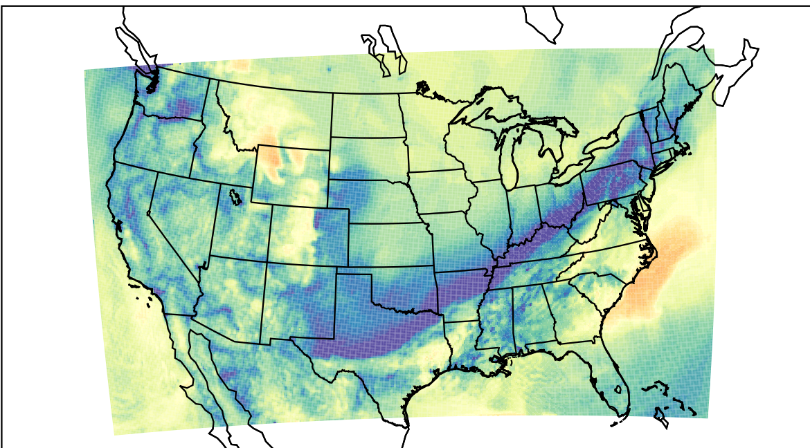
WRF (2019-11-07_16:00:00)
