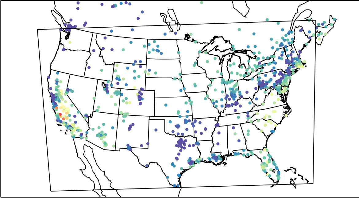
AirNOW (2019-11-07_18:00:00)
