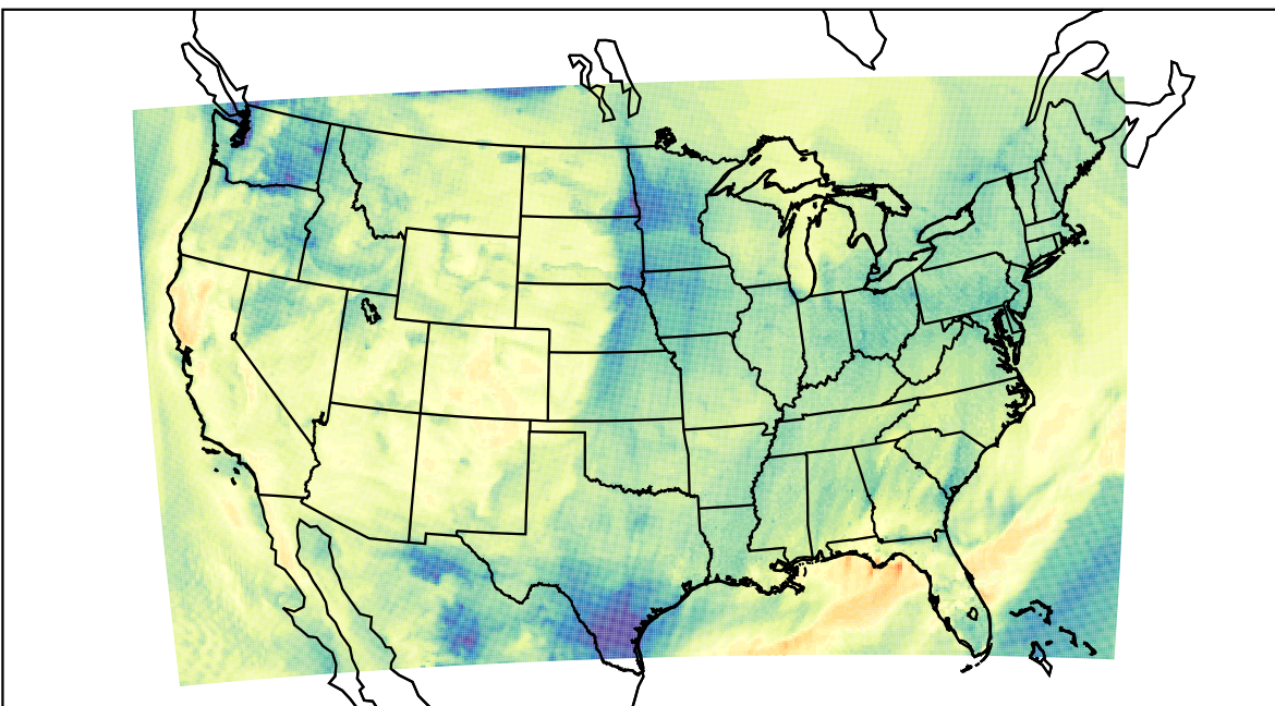
WRF (2019-11-08_21:00:00)
