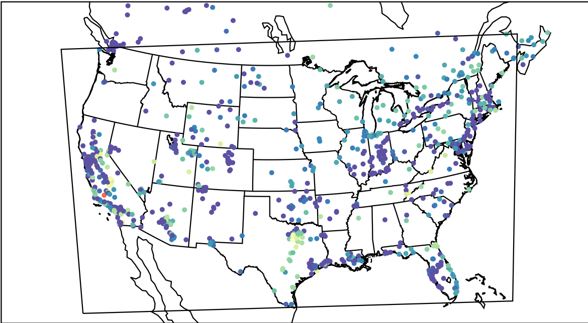
AirNOW (2019-11-07_06:00:00)
