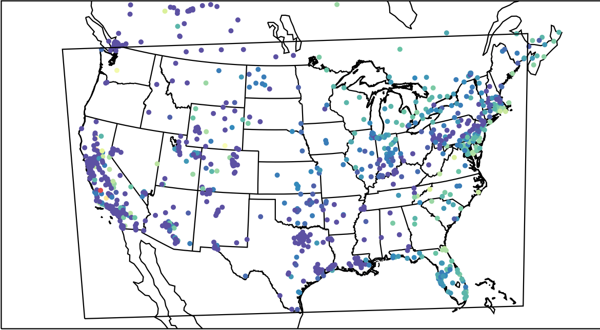
AirNOW (2019-11-07_15:00:00)
