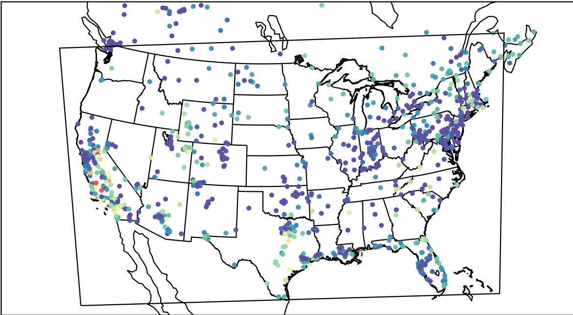
AirNOW (2019-11-07_02:00:00)
