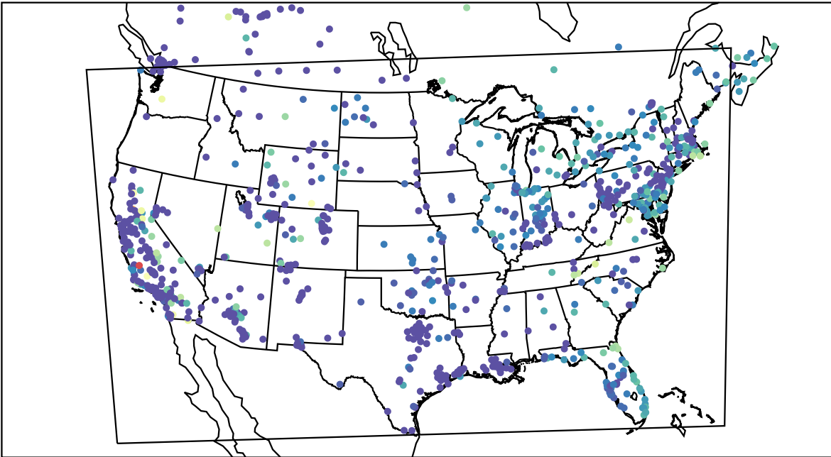
AirNOW (2019-11-07_14:00:00)
