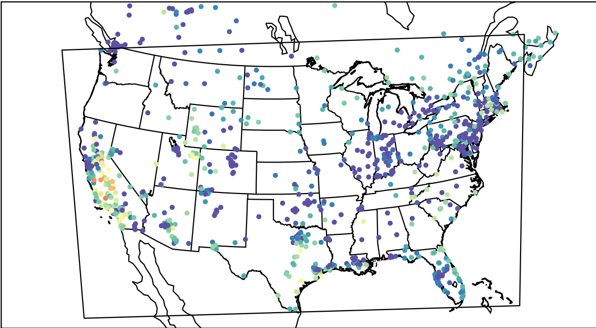
AirNOW (2019-11-07_01:00:00)
