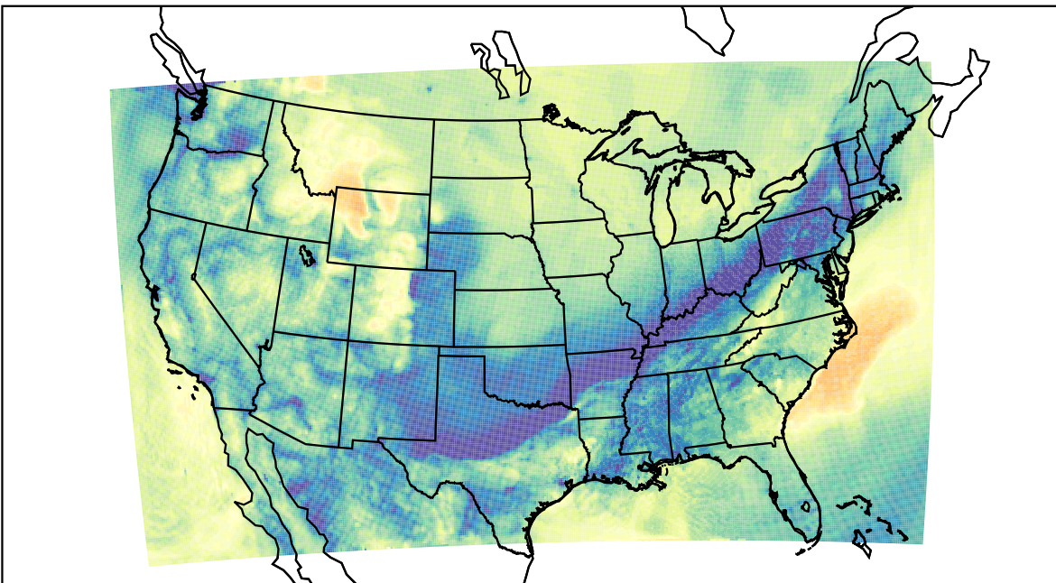
WRF (2019-11-07_15:00:00)
