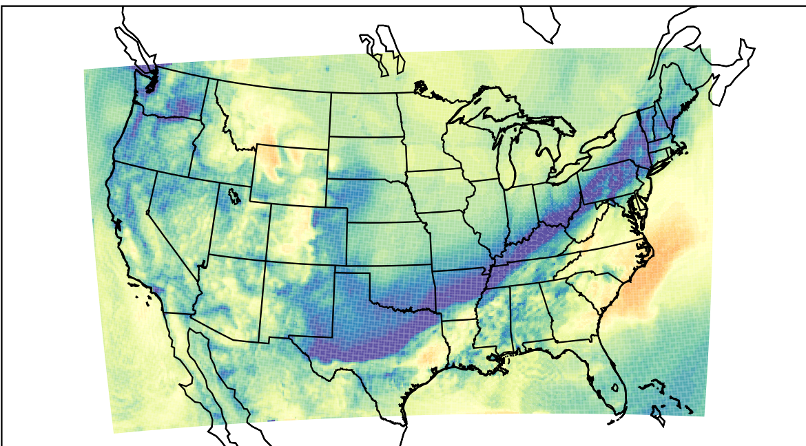
WRF (2019-11-07_17:00:00)
