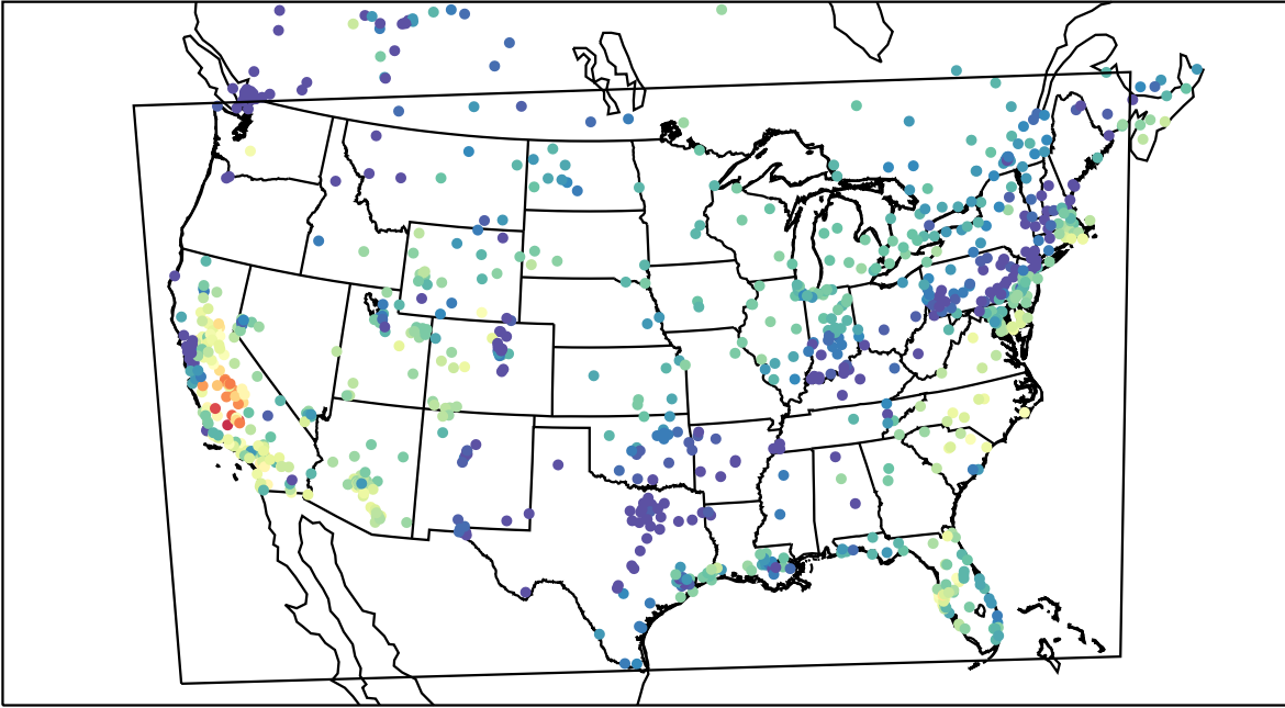
AirNOW (2019-11-07_19:00:00)
