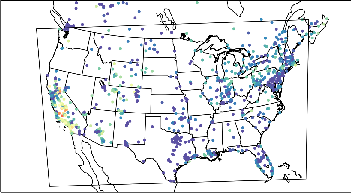
AirNOW (2019-11-08_01:00:00)
