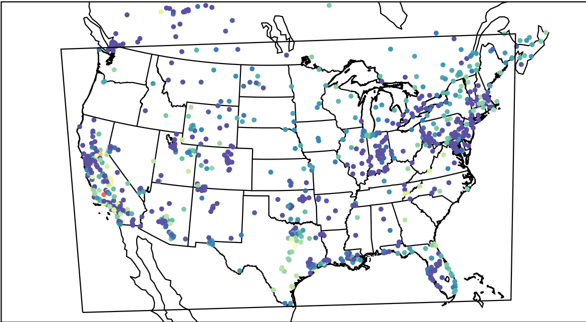
AirNOW (2019-11-07_04:00:00)
