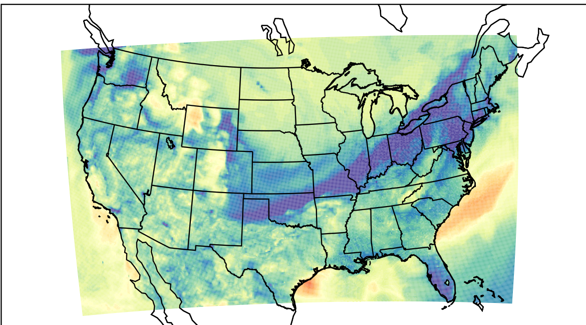
WRF (2019-11-07_07:00:00)
