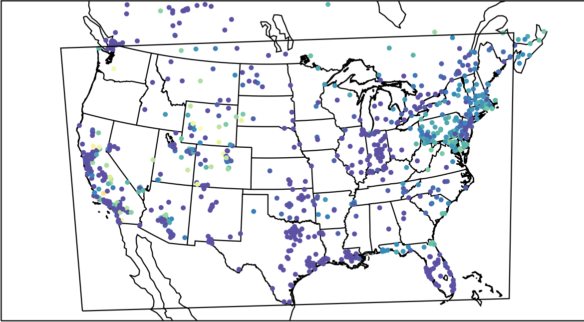
AirNOW (2019-11-08_12:00:00)
