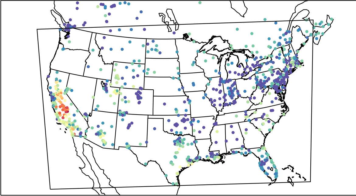
AirNOW (2019-11-07_00:00:00)
