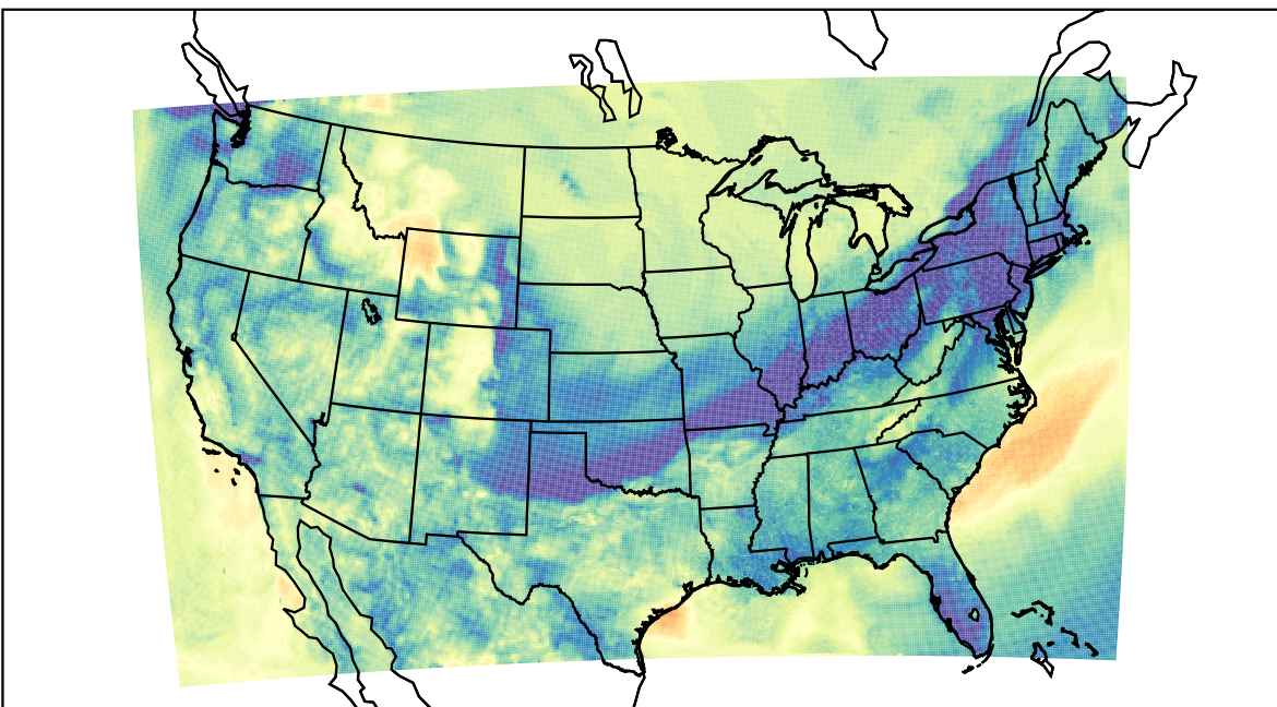
WRF (2019-11-07_09:00:00)
