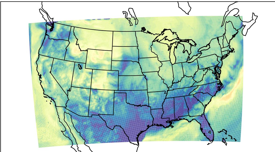
WRF (2019-11-08_12:00:00)
