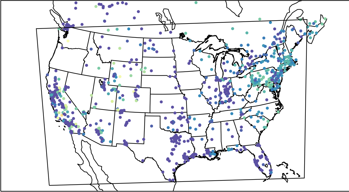
AirNOW (2019-11-08_09:00:00)
