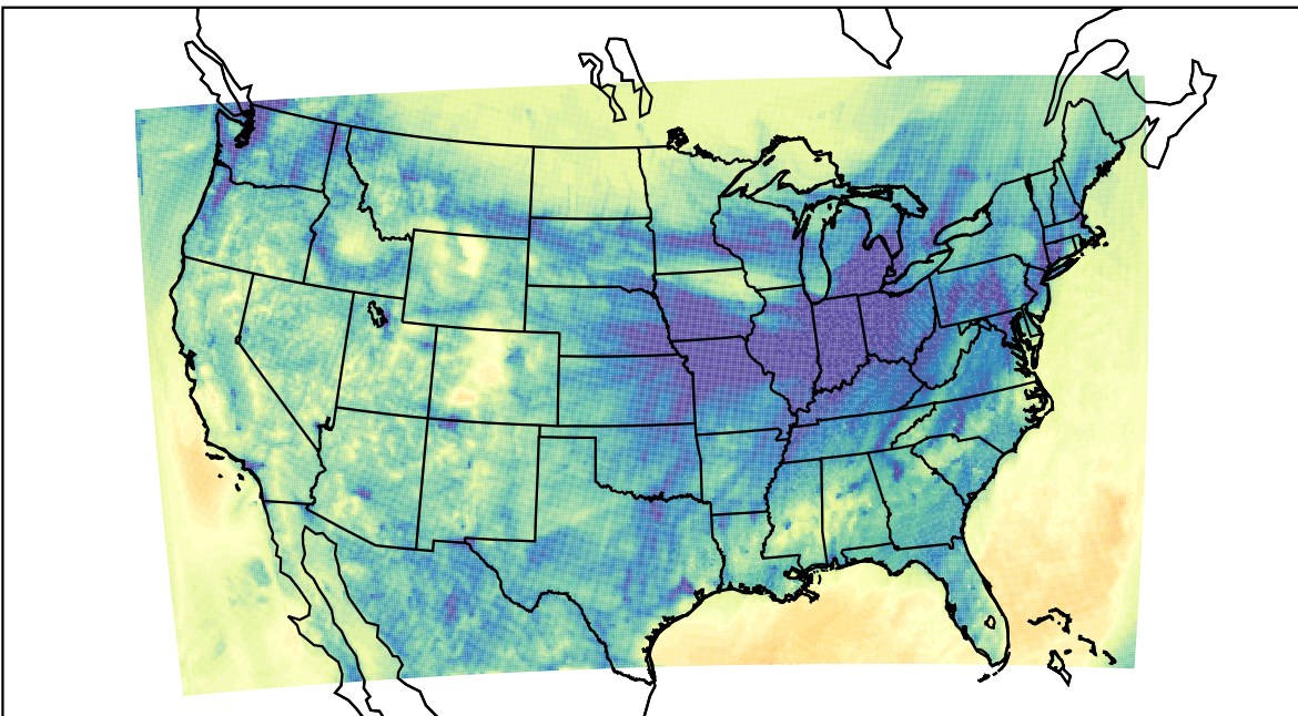
WRF (2019-11-10_05:00:00)
