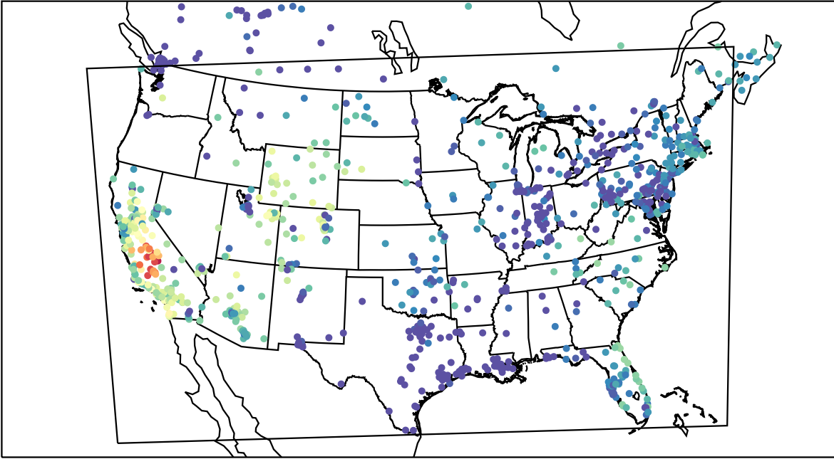
AirNOW (2019-11-09_00:00:00)
