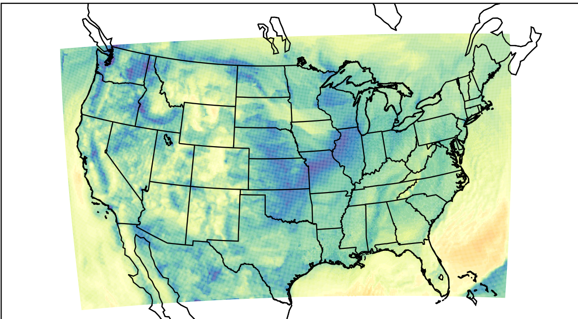
WRF (2019-11-09_17:00:00)
