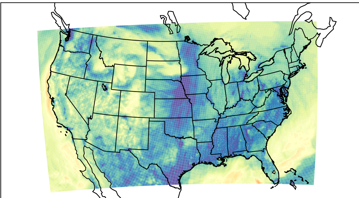
WRF (2019-11-09_05:00:00)
