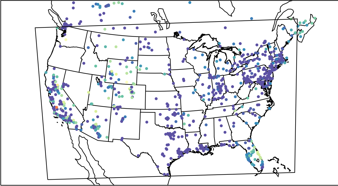
AirNOW (2019-11-09_11:00:00)
