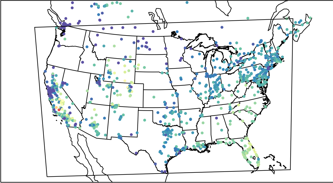
AirNOW (2019-11-09_17:00:00)
