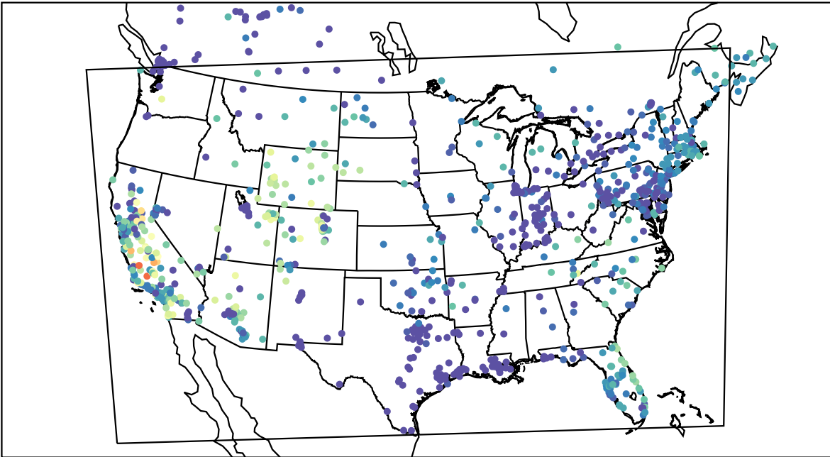
AirNOW (2019-11-09_01:00:00)
