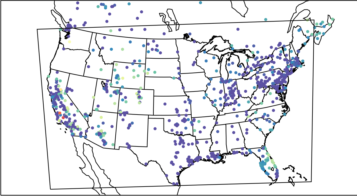
AirNOW (2019-11-09_09:00:00)
