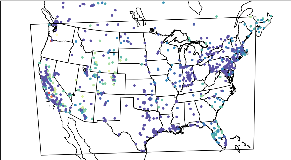
AirNOW (2019-11-09_07:00:00)
