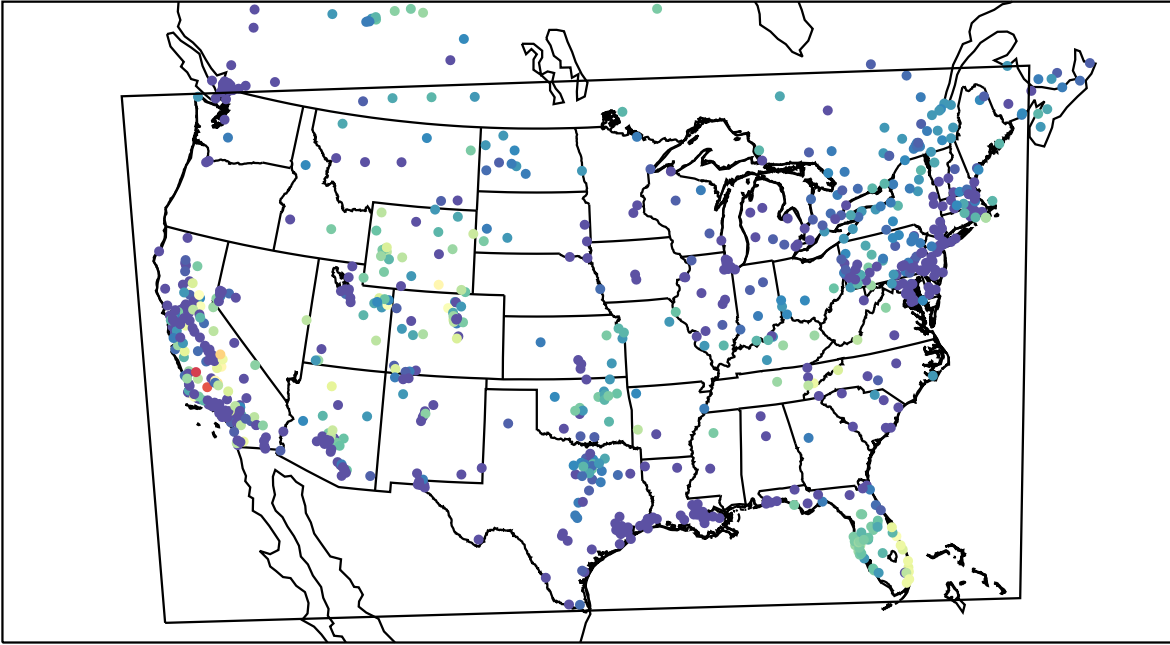
AirNOW (2019-11-10_05:00:00)
