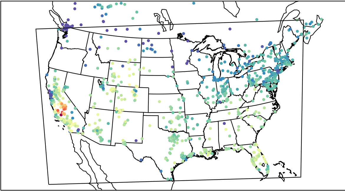
AirNOW (2019-11-09_19:00:00)
