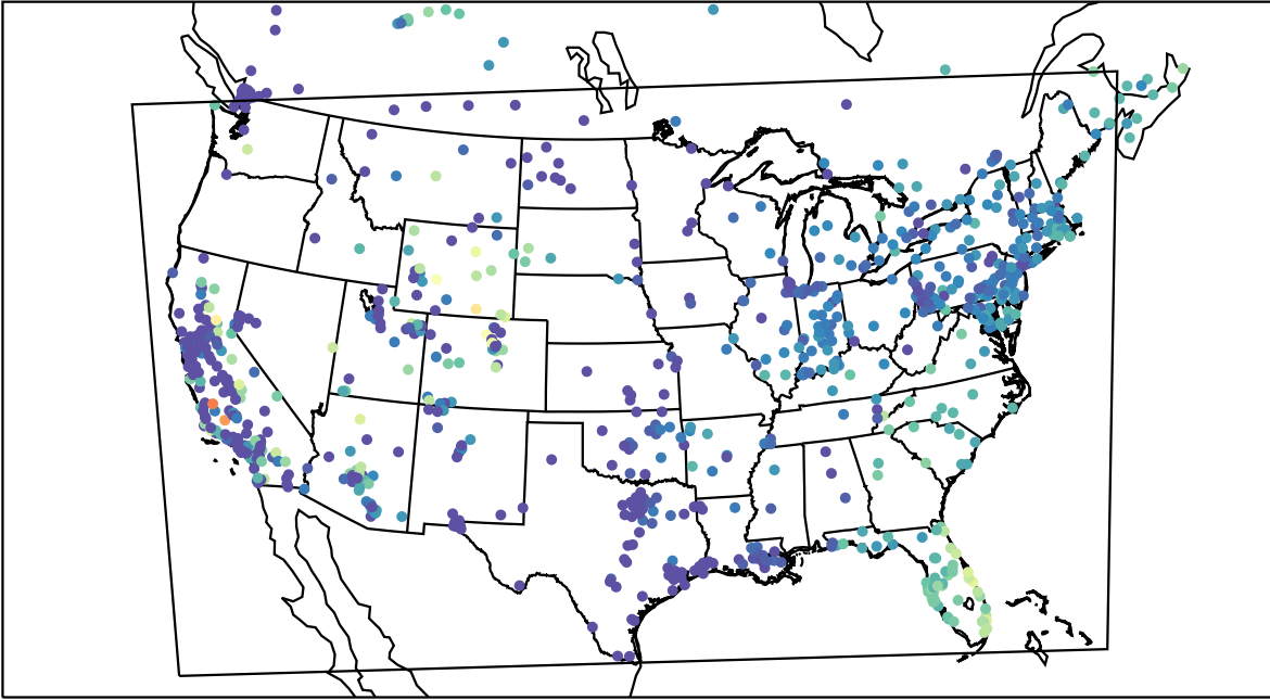
AirNOW (2019-11-09_15:00:00)
