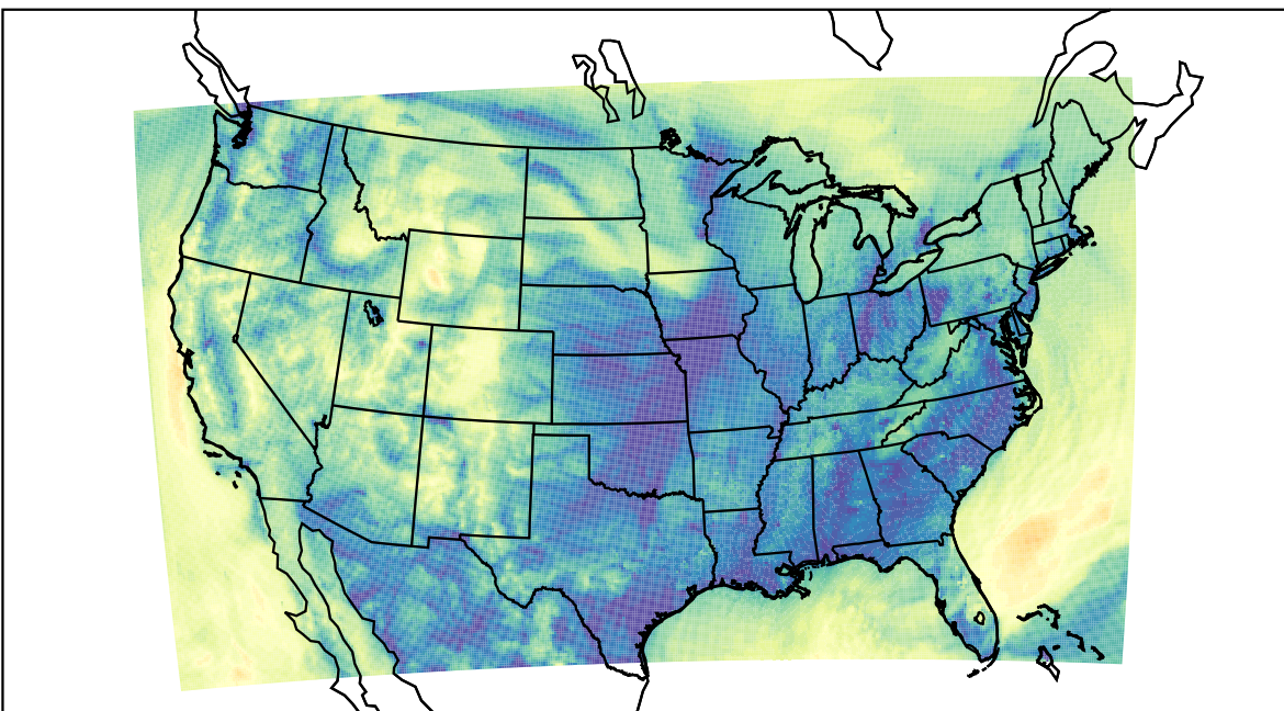
WRF (2019-11-09_12:00:00)
