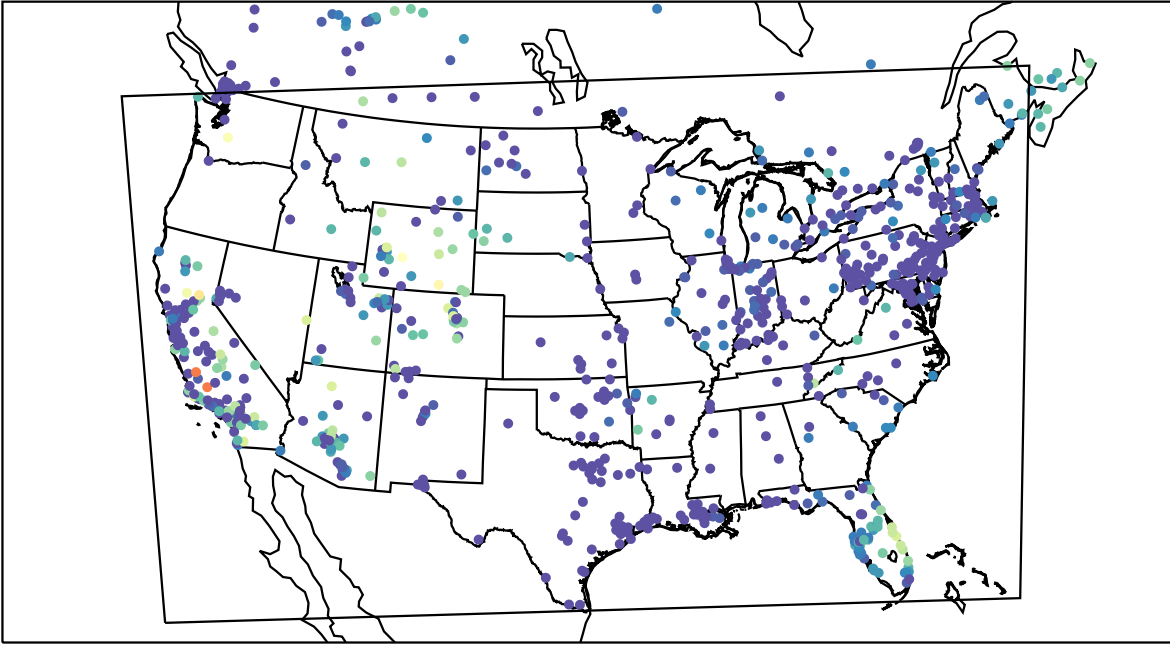
AirNOW (2019-11-09_12:00:00)
