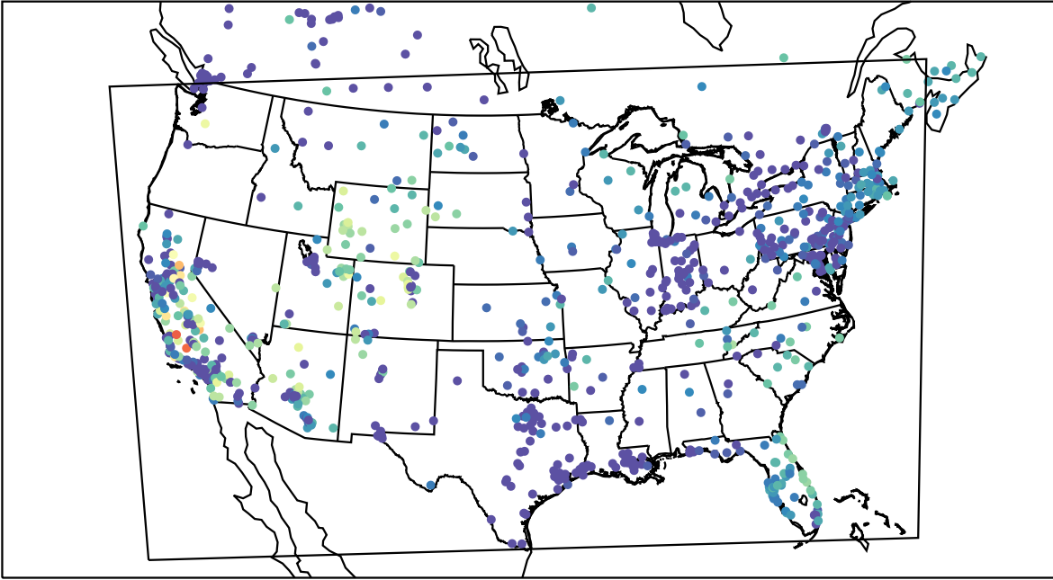
AirNOW (2019-11-09_02:00:00)
