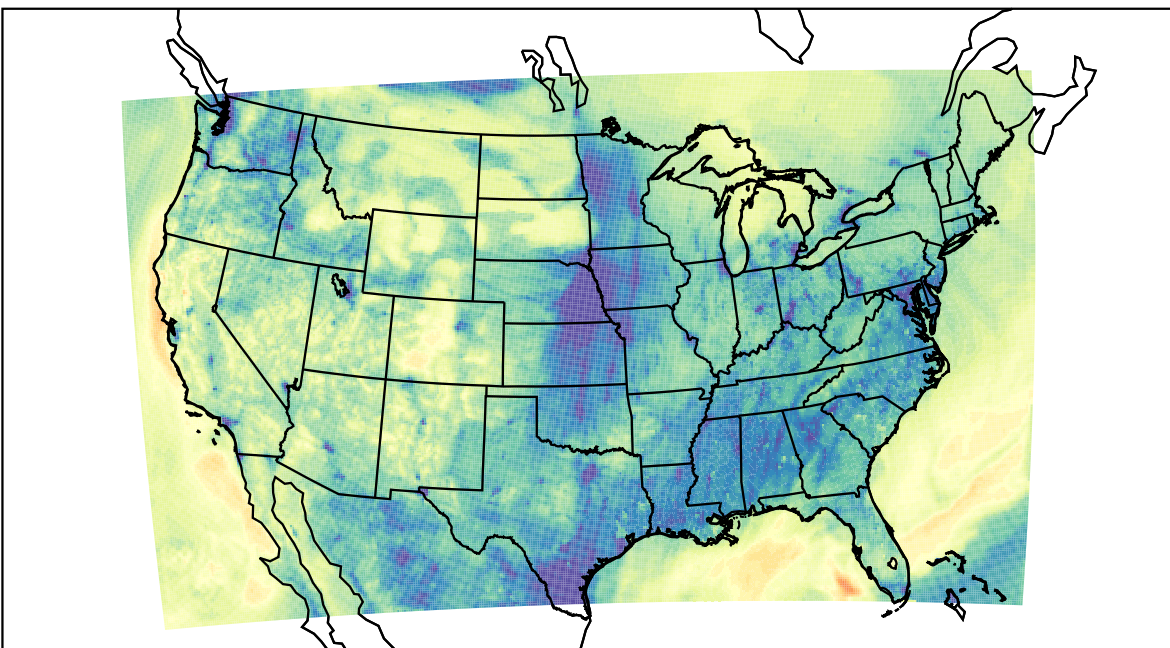
WRF (2019-11-09_02:00:00)
