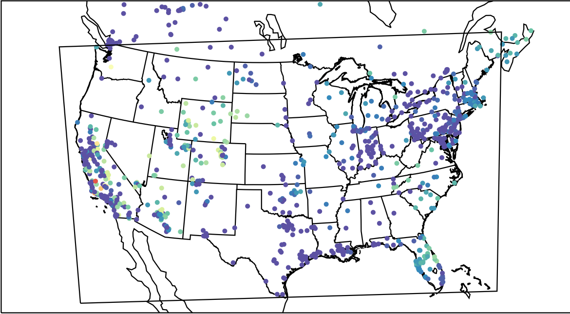
AirNOW (2019-11-09_05:00:00)
