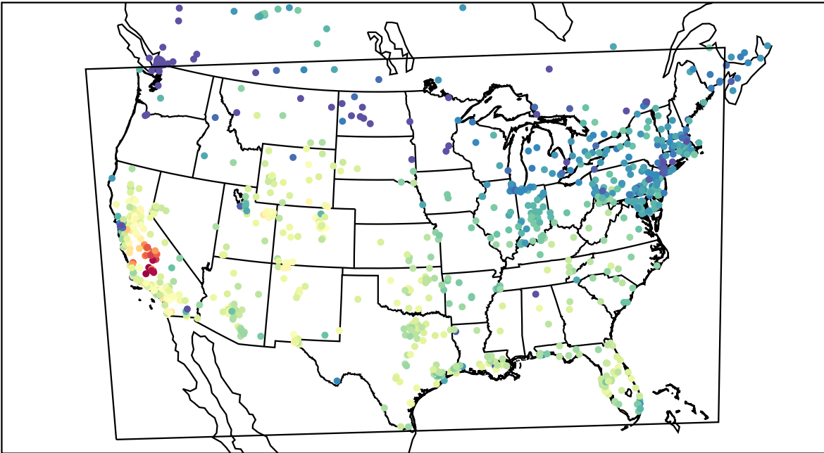
AirNOW (2019-11-09_21:00:00)
