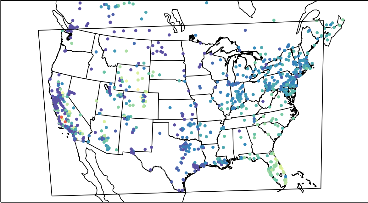
AirNOW (2019-11-09_16:00:00)
