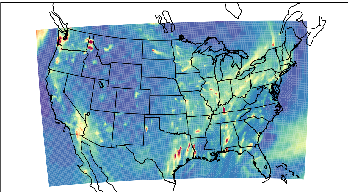
WRF 2019-11-15_05:00:00
